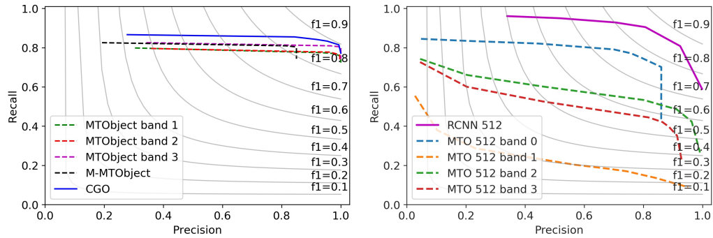
(a) Evaluation on the FDS Simulation. (b) RCNN vs. MTO on KiDS dataset.
