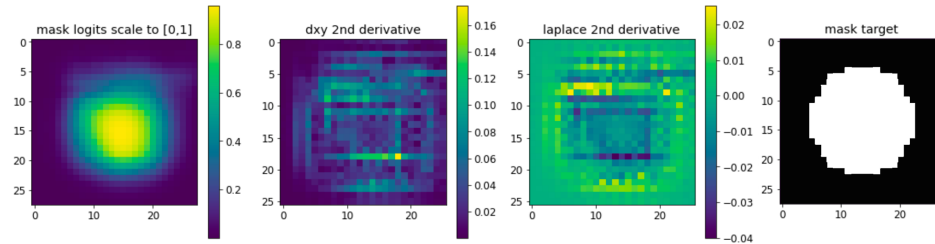
(b) The model with smoothness regularizer.
