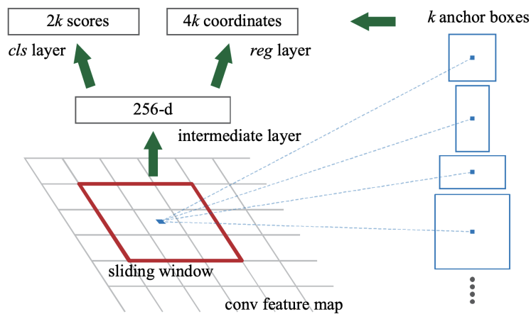
Figure 4.4: Anchor is defined by a center pixel, a scale, and a aspect ratio [Ren et al., 2015].
