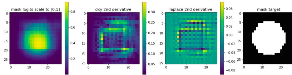
(a) The model without smoothness regularizer.
