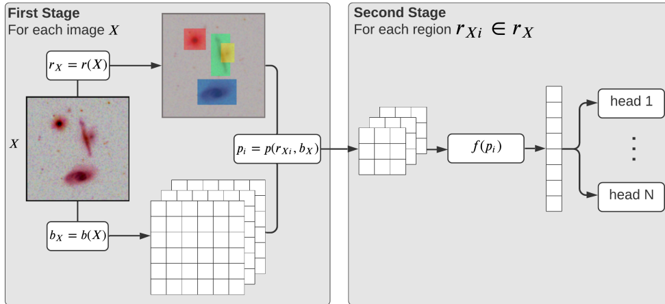
Figure 4.2: Generalized R-CNN Framework
