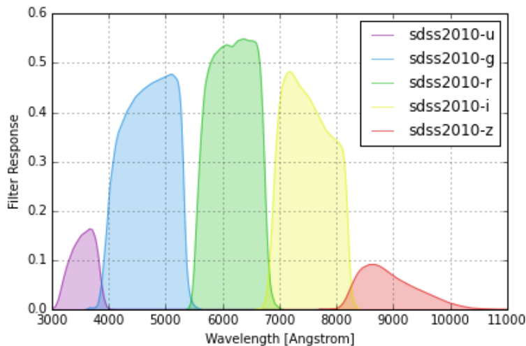
Figure 1.4: SDSS optical filter responses [Doi et al., 2010].
