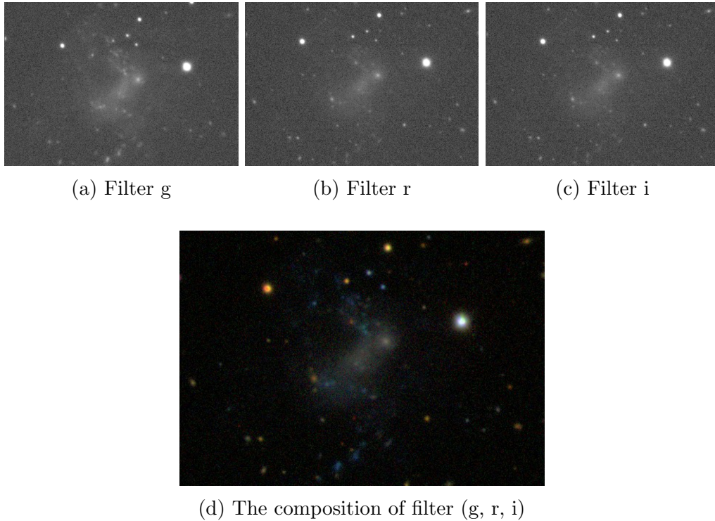
Figure 1.6: The UGC 07332: (a-c) Three single-band images associate to three filters g r i and (d) The composition of the three single-band images, source SDSS.
