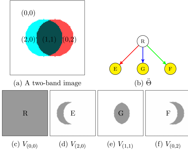
Figure 3.5: Partial object detection: (a) A two-band image I valued on \mathbb{V} = \{(0,0), (2,0), (0,2), (1,1)\} equipped with the marginal order relation \leq_m ; (b) The CG \tilde{\Theta} of the input image where yellow nodes are significant; and (c-f) The threshold sets V_v for v \in \mathbb{V} .
