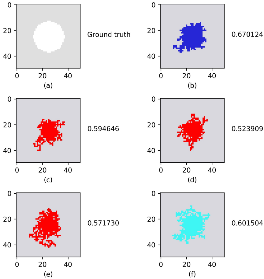
Figure 3.11: Single Source Simulation An example of similarity upper bound components \text{Sup} with Jaccard index J(N, gt) on: (a) Ground truth component gt ; The most similar component to the gt in (b) the component-graph of the multi-band; (c-e) in the component-tree of three separate bands; and (f) in the component-tree of the average band.
