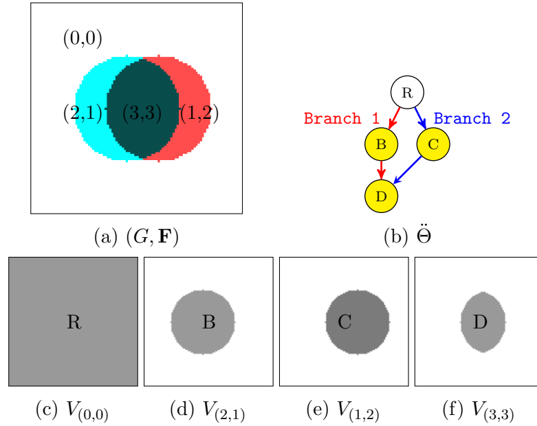
Figure 3.4: Duplicated objects detection: (a) A two-band image, (b) The CG \ddot{\Theta} , where significant nodes are marked yellow. Branch 1 and Branch 2 are incomparable and growing to the same leaf node.
