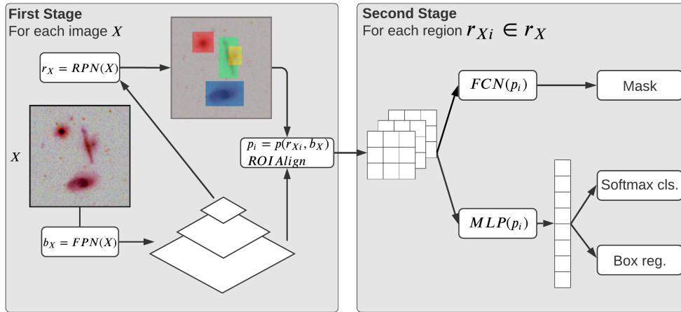
Figure 4.5: Mask R-CNN Framework with FPN backbone.
