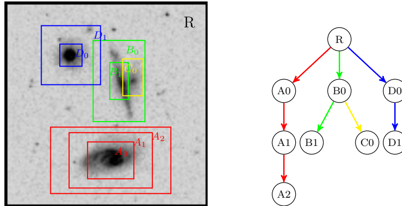
(a) Region proposals of an image. (b) Corresponding proposal hierarchy.
