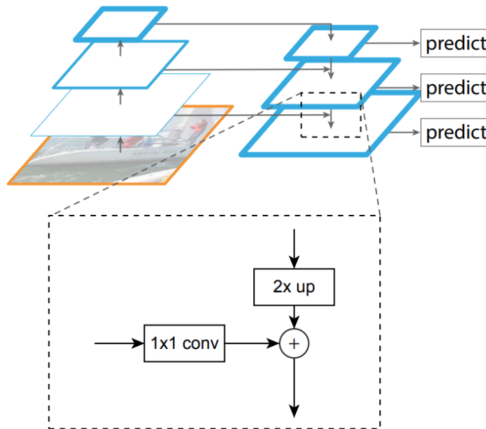
Figure 4.8: The FPN bottom-up/top-down pathway architecture with lateral connections: (2 \times up) is up-sampling by a factor of 2; (1 \times 1conv) is convolution operator to reduce channel dimension but retain the spatial resolution; and merge operator (+) is element-wise addition [Lin et al., 2017a].
