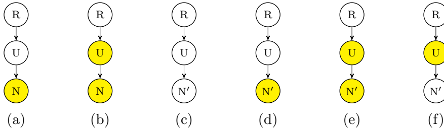
Figure 3.8: The possible links between nodes in the max-tree of N , N' adjacent to N , and U = N \cup N' in the band b : (a-b) L(N)_b > L(N')_b and (c-f) L(N)_b \leq L(N')_b .
