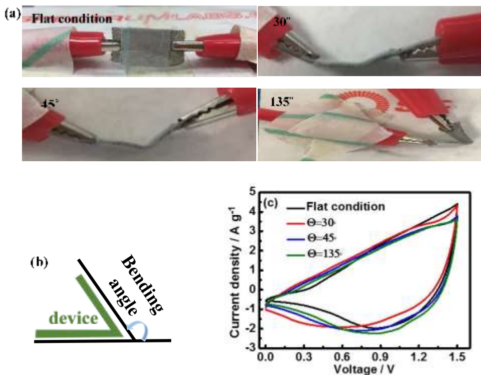
Figure 2.14: (a) Images of the bent cells, (b) Schematic illustration of the bent cell, (c) CV curves of the ASC at 50 mV/s under different bending angles of 0-135°.
