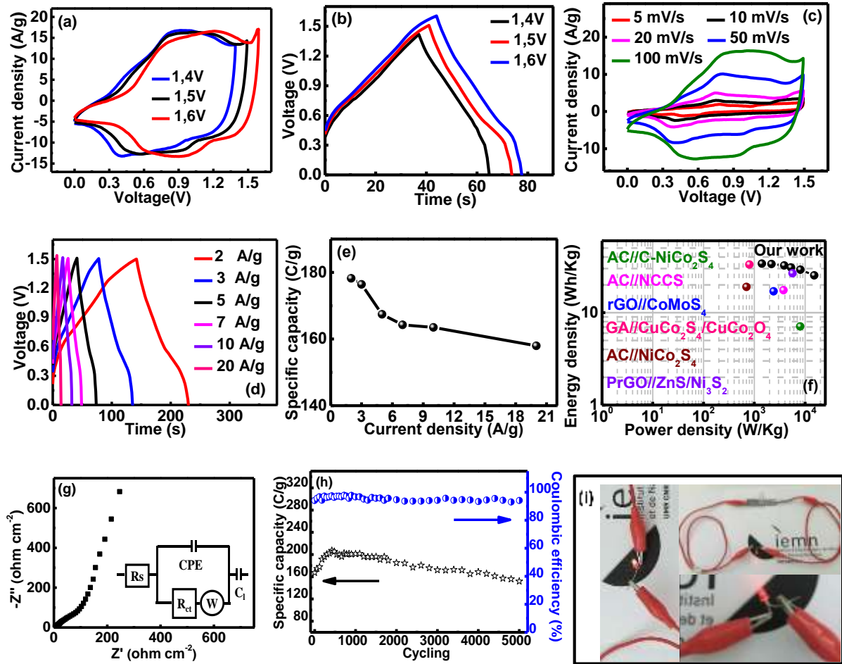
Figure 5.8: Electrochemical properties of the hybrid PrGO// Sb: Cr: Co(1:3:4) supercapacitor: (a) and (b) are the CV and GCD curves at different cell voltage values, respectively, (c) CV curves recorded at various scan rates, (d) GCD curves acquired at various current densities, (e) variation of the specific capacity vs. current density, (f) typical Ragone plot of the prepared supercapacitor, (g) Nyquist plot of the prepared supercapacitor, (h) cycling performance and coulombic efficiency of the fabricated supercapacitor at a current density of 5 \text{ A g}^{-1} , (i) photographs of the red LED lighted up by two connected hybrid supercapacitors.
