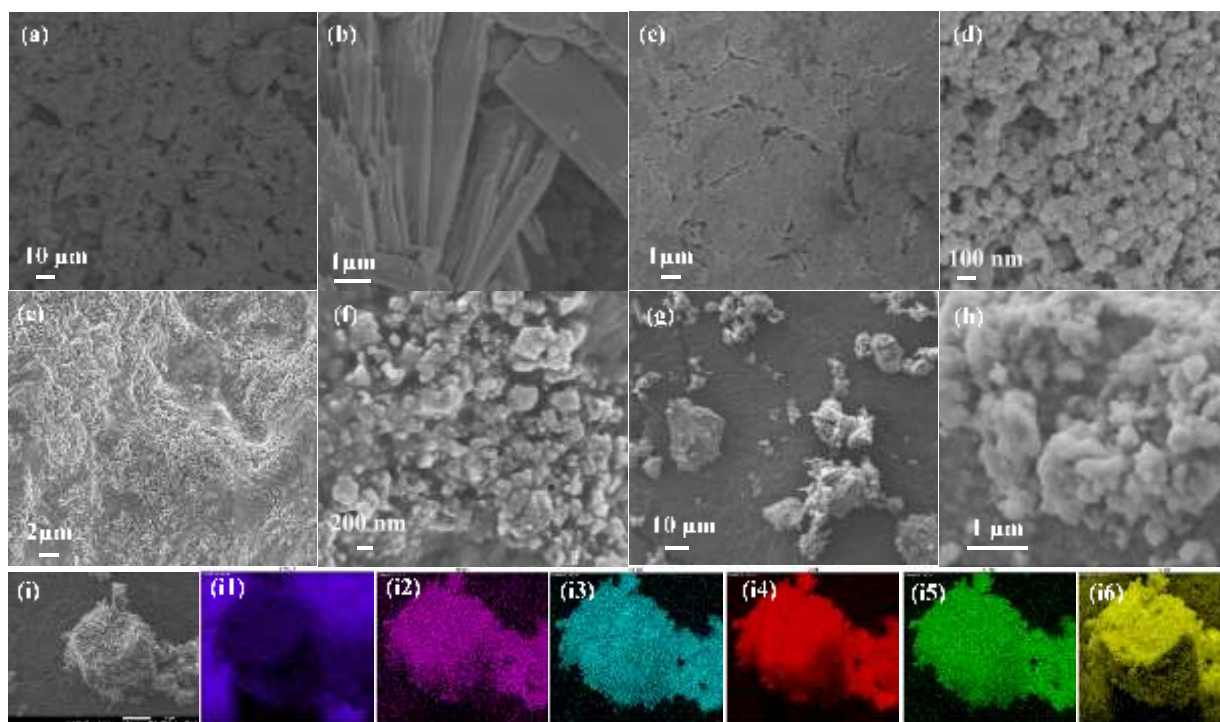
Figure 5.4: SEM images of \text{Sb}_2\text{S}_3 (a, b), \text{CrOOH} (c, d), \text{CoS}_2 (e, f) and \text{Sb}_2\text{S}_3/\text{CoS}_2/\text{CrOOH} (g, h), and element mappings of C, Sb, Co, S, Cr, O elements recorded from \text{Sb}_2\text{S}_3/\text{CoS}_2/\text{CrOOH} (i).
