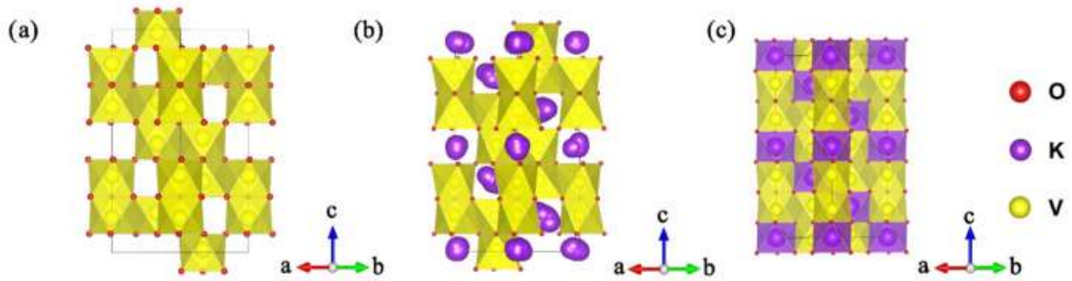
Figure 1.10: Electrochemical behavior calculated by DFT; a) optimized structure of V_2O_5 , b) trajectories of K ions in KV_2O_5 obtained by the ab initio molecular dynamics (AIMD) simulation at 2000K for 4ps, c) optimized structures of KV_2O_5 [60].
