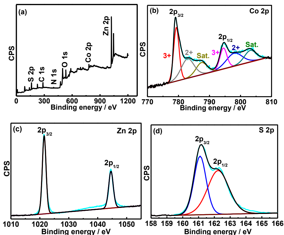
Figure 3.16: XPS analysis of Zn: Co (1:2) 50 electrode material: (a) full spectrum, and high resolution spectra of (b) \text{Co}_{2p} , (c) \text{Zn}_{2p} , (d) \text{S}_{2p} . “Sat.” in the Fig. 3.15 denotes satellite peaks.
