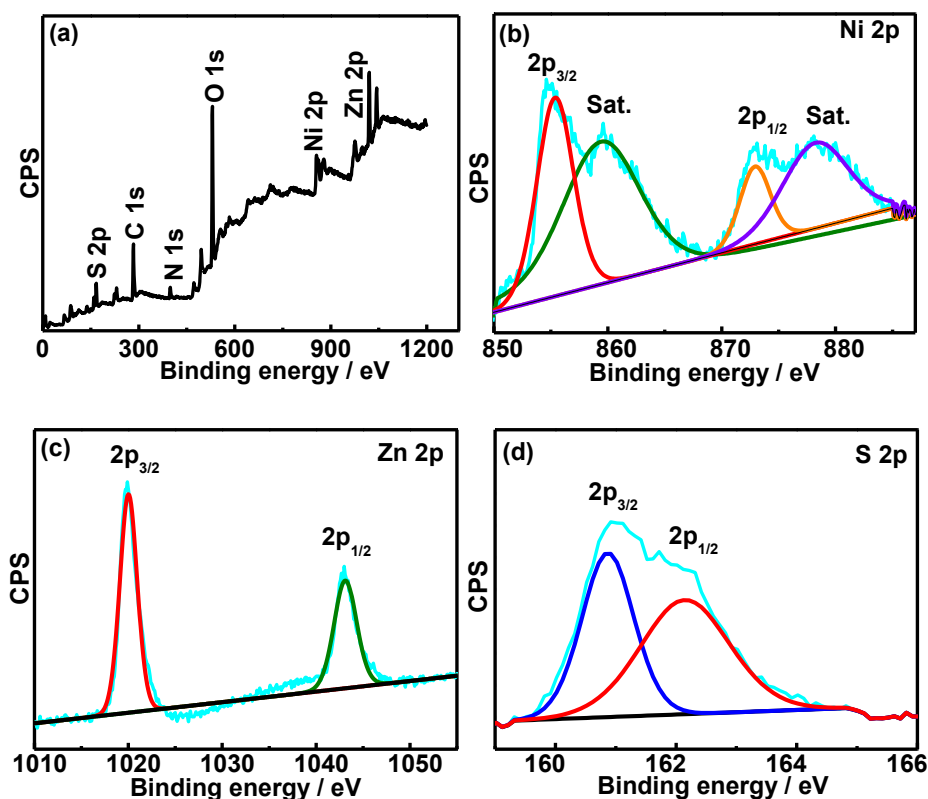
Figure 4.2: XPS analysis of ZnS/Ni 3 S 2 : (a) full spectrum; (b), (c) and (d) are respectively the Ni 2p , Zn 2p and S 2p high resolution spectra. “Sat” in Fig. 4.2b denotes satellite peaks.
