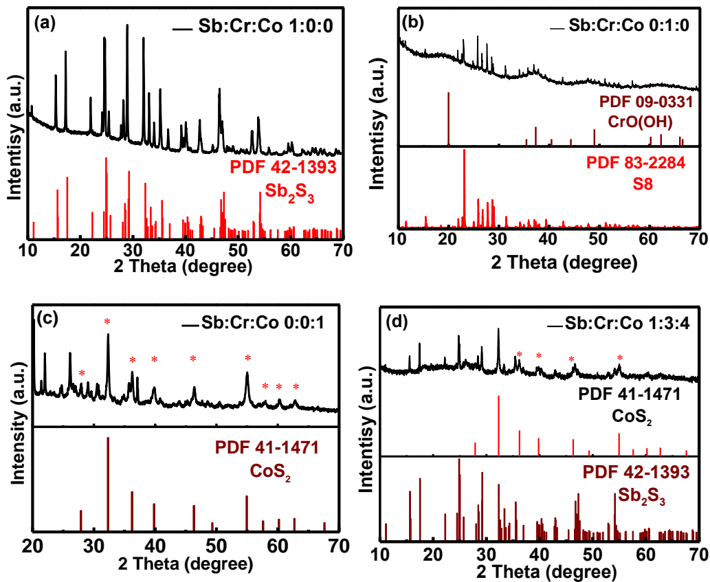
Figure 5.2: XRD patterns of the prepared Sb: Cr: Co samples.
