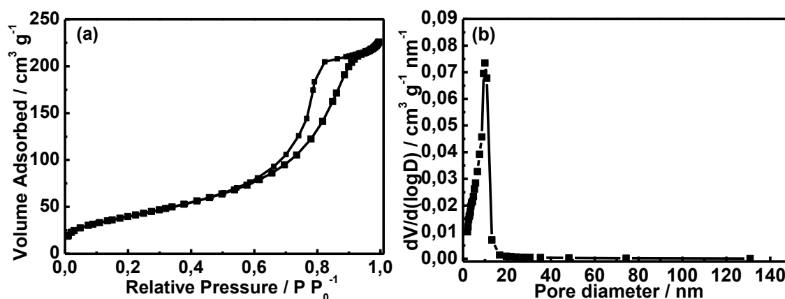
Figure 4.4: (a) Nitrogen adsorption-desorption isotherm and (b) pore size distribution curve of ZnS/Ni 3 S 2 .
