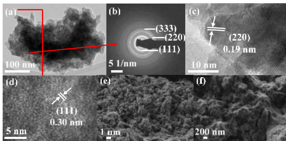
Figure 3.18: TEM images (a), SAED pattern (b), HRTEM images (c, d), and SEM images (e, f) of Zn: Co (1:2) 50.
