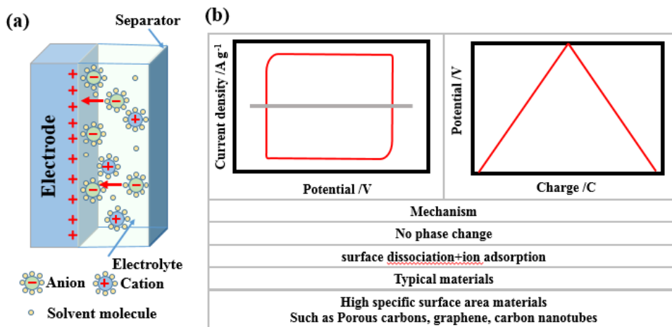
Figure 1.3: The schematic illustration of electrical double layer capacitance (EDLC) (a), summary of characteristic metrics such as CV, GCD, key mechanism descriptions and typical materials (b) [8, 9].
