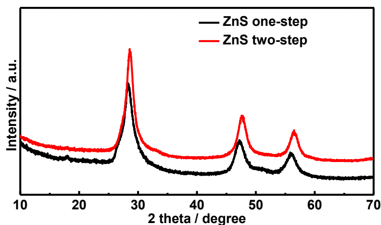
Figure 3.2: XRD patterns of as-obtained ZnS electrode materials.
