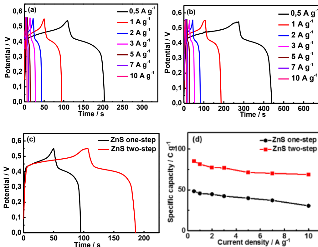
Figure 3.5: GCD curves at different current densities of ZnS (one-step) (a), ZnS (two-step) (b), comparison of GCD curves at a current density of 1 A g -1 (c), specific capacity at different current densities (d).
