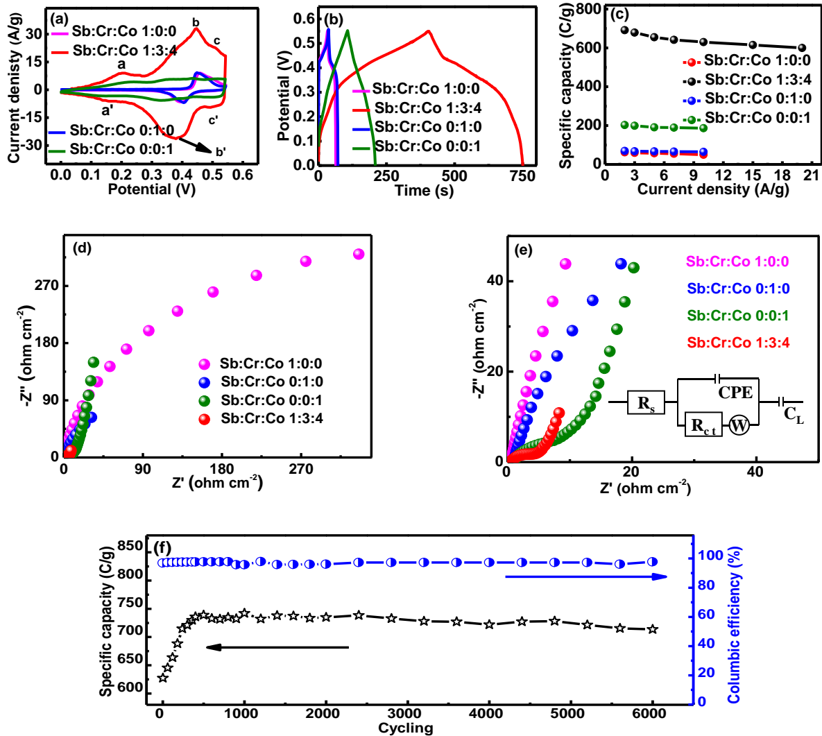
Figure 5.6: (a) CV curves of all electrodes recorded at a scan rate of 10 mV/s; (b) GCD curves recorded of all electrodes at a current density of 2 A g -1 ; (c) Specific capacity of all electrodes acquired at current densities of 2-20 A g -1 ; (d, e) Nyquist plots of all Sb:Cr:Co electrodes; (f) cycling performance and columbic efficiency of Sb:Cr:Co (1:3:4) at 20 A g -1 for 6,000 cycles, the inset in (e) is the corresponding equivalent circuit.
