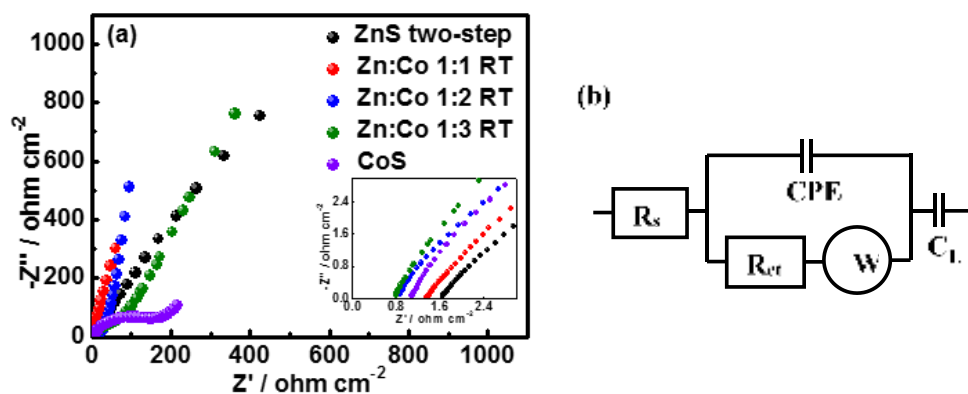
Figure 3.14: Nyquist plots of ZnCoS RT electrodes (a), the corresponding equivalent circuit (b).
