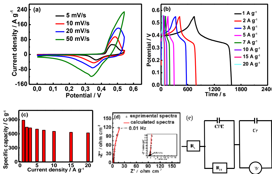
Figure 4.7: Electrochemical properties of ZnS/Ni 3 S 2 electrode in 2 M KOH: (a) CV curves at different scan rates (5 to 50 mV s -1 ), potential=0 to +0.55V; (b) GCD profiles at various current densities of 1, 2, 3, 5, 7, 10, 15 and 20 A g -1 ; (c) the corresponding specific capacities within the current density span of 1 to 20 A g -1 ; (d) Nyquist plots; (e) the corresponding equivalent circuit.
