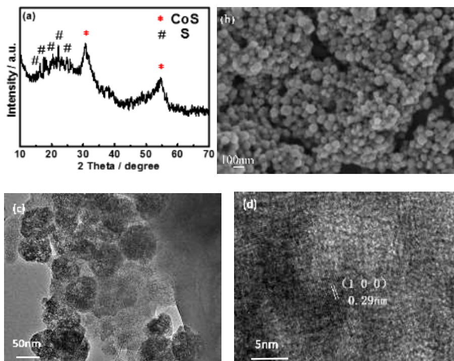
Figure 2.3: XRD pattern (a), SEM (b), TEM (c) and HRTEM (d) images of CoS sample.
