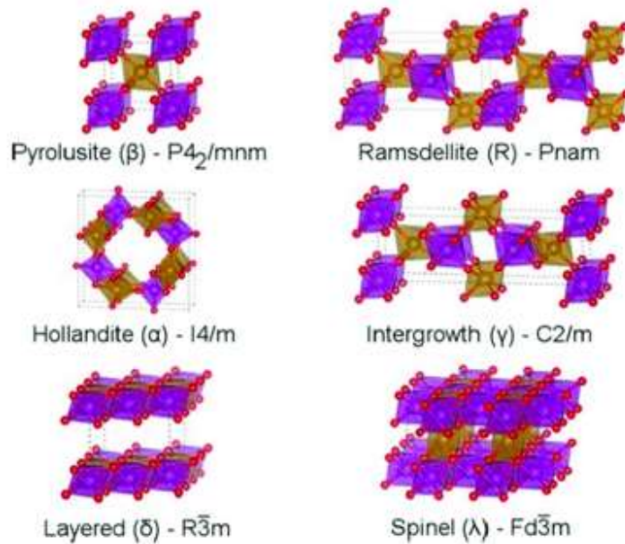
Figure 1.9: Illustration of the crystal structures of selected common manganese oxides [50].
