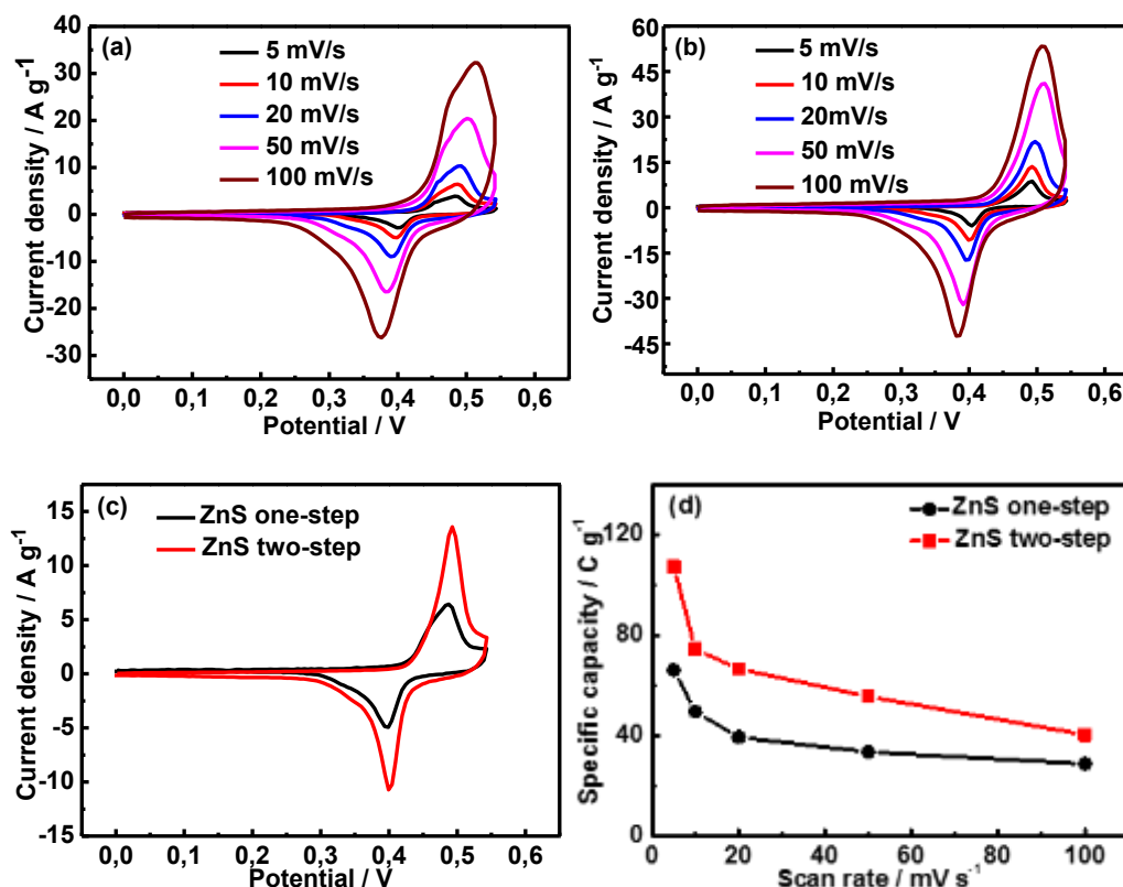
Figure 3.4: CV curves at different scan rates of ZnS one-step (a), ZnS two-step (b), comparison of CV curves at a scan rate of 10 mV/s (c), specific capacity at different scan rates (d).
