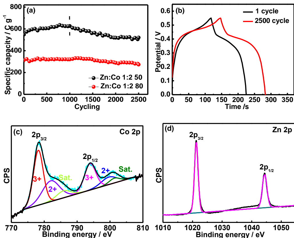
Figure 3.23: (a) Cycling performance of Zn: Co 1:2 electrodes; (b) GCD curves after the first and 2,500 th cycle acquired at a current density of 5 A g -1 ; high resolution XPS spectrum of the Co 2p (c) and Zn 2p (d) after 2,500 cycles of Zn: Co (1:2) 50.
