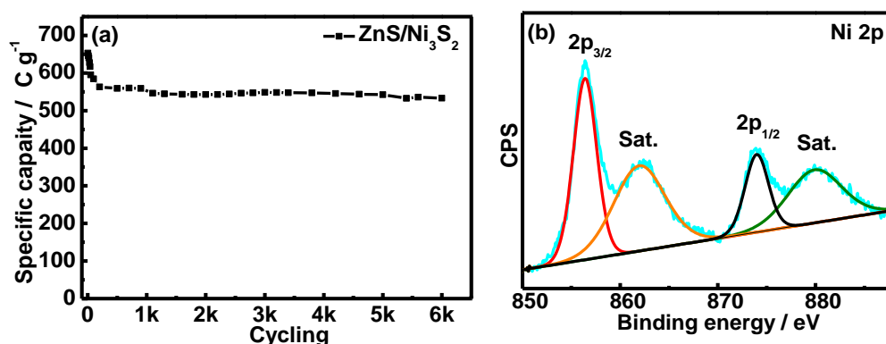
Figure 4.8: (a) Stability test of ZnS/Ni 3 S 2 electrode at 10 A g -1 for 6,000 cycles; (b) Ni 2p high resolution XPS spectrum after 6,000 cycles. “Sat” in Fig. 6b denotes satellite peaks.
