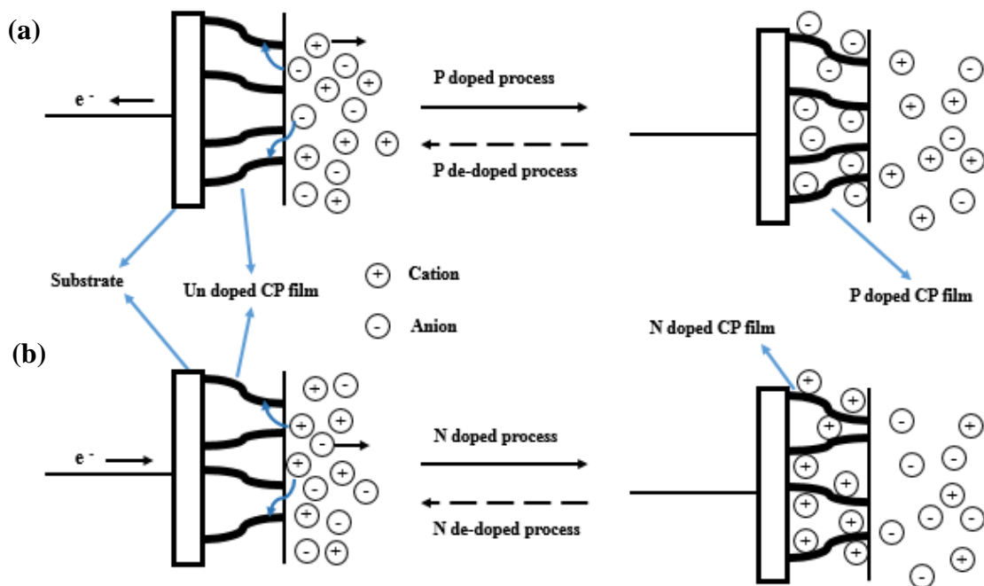
Figure 1.12: Schematic representation of electrochemical doping of CPs: (a) p-doping and (b) n-doping [77].
