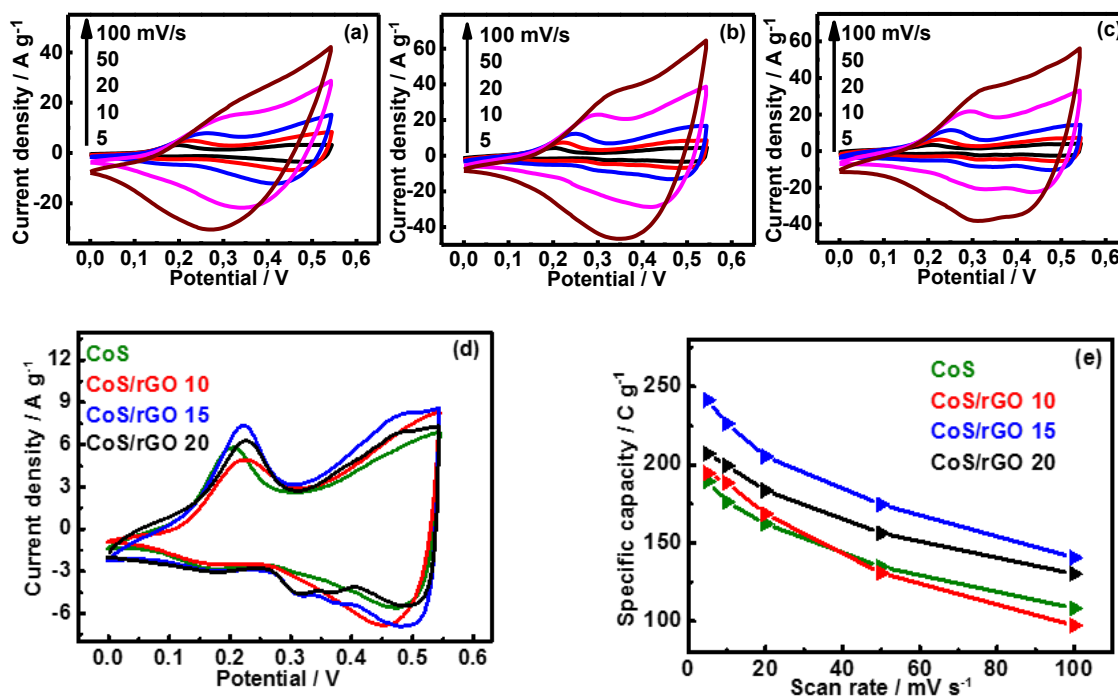
Figure 2.7: CV curves of CoS/rGO 10 (a), CoS/rGO 15 (b), CoS/rGO 20 (c) electrodes, comparison of CV curves at a scan rate of 10 mV/s (d), specific capacity of all CoS/rGO electrodes at different scan rates (e).
