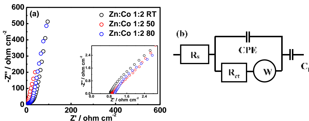
Figure 3.22: Nyquist plots of Zn: Co (1:2) electrodes (a), and the corresponding equivalent circuit (b).
