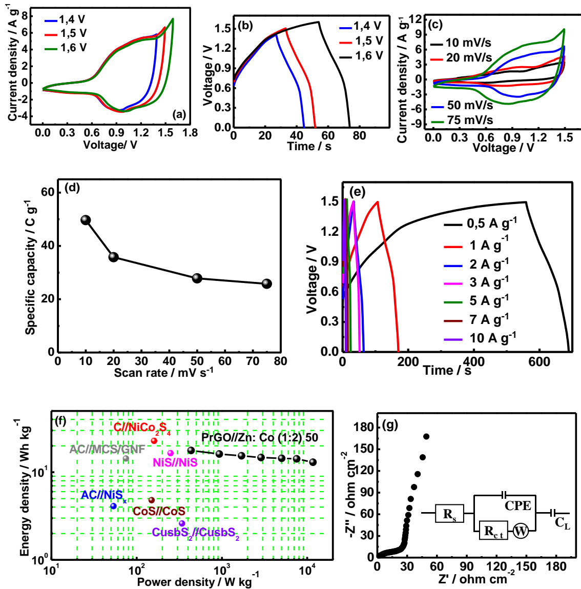
Figure 3.28: (a) CV and (b) GCD curves at different cell voltage values, (c) CV curves at various scan rates, (d) variation of the specific capacity as a function of scan rate, (e) GCD curves at various current densities, (f) typical Ragone plot, (g) Nyquist plot of the fabricated asymmetric supercapacitor device, the inset in (g) is the corresponding equivalent circuit.
