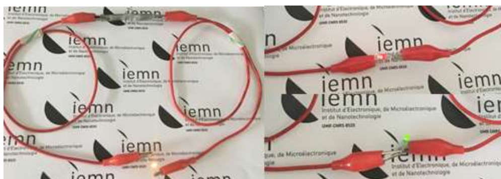
Figure 4.10: Photographs of the LEDs (yellow, red and green) powered by two asymmetric supercapacitor connected in series.
