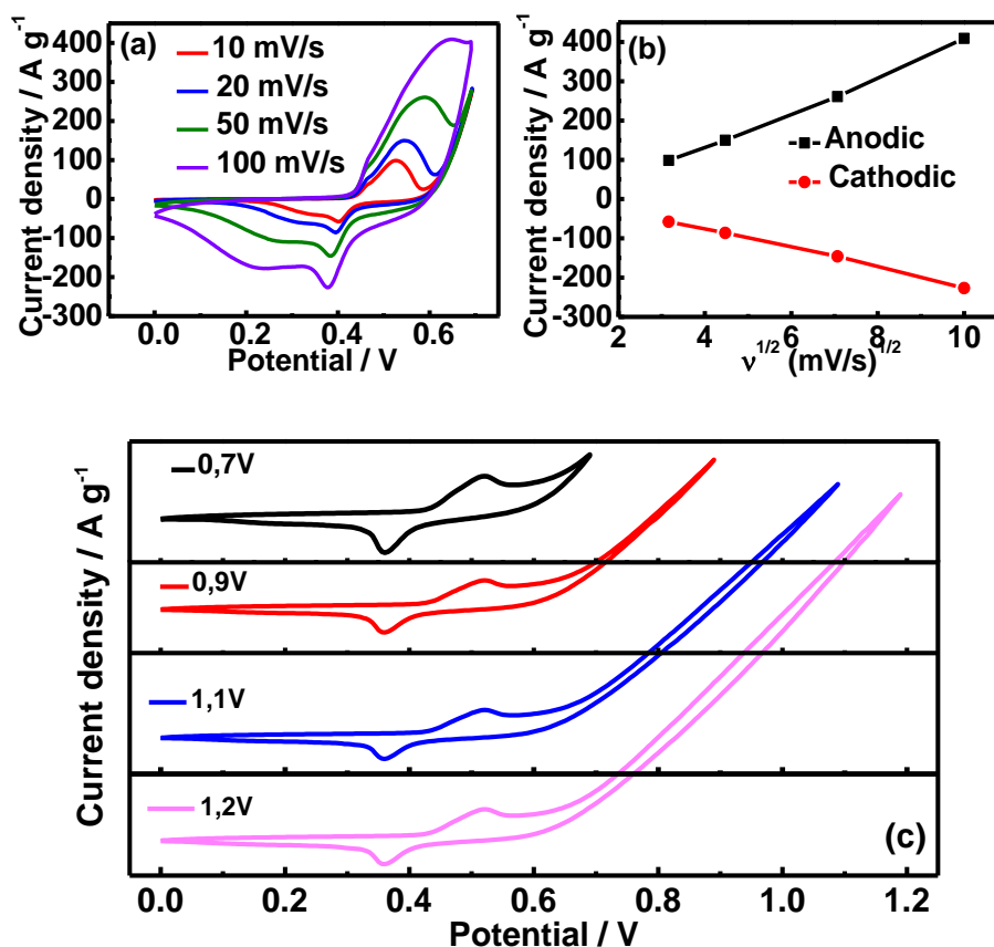
Figure 4.5: Electrochemical properties of ZnS/Ni 3 S 2 electrode within the potential range of 0 to +0.7 V in 2 M KOH: (a) CV curves, (b) the anodic and cathodic peak current densities v_s vs. the square root of scan rate, (c) CV curves of ZnS/Ni 3 S 2 electrodes recorded in different potential windows at a scan rate of 50 mV s -1 .
