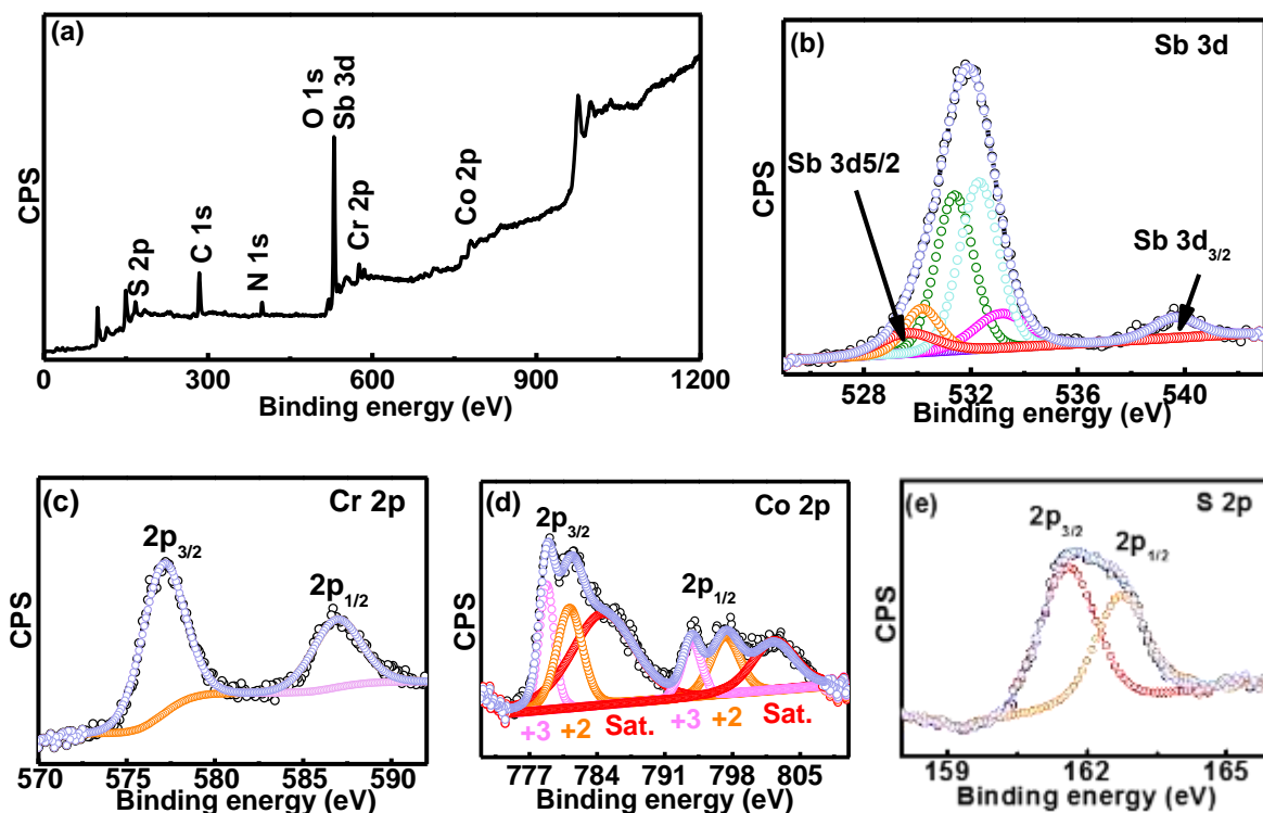
Figure 5.3: XPS analysis of Sb: Cr: Co (1:3:4): (a) survey spectrum, (b), (c) (d) and (e) are the high-resolution spectra of \text{Sb}_{3d} ( \text{O}_{1s} ), \text{Cr}_{2p} and \text{Co}_{2p} and \text{S}_{2p} , respectively. “Sat” in Fig. d denotes satellite peaks.
