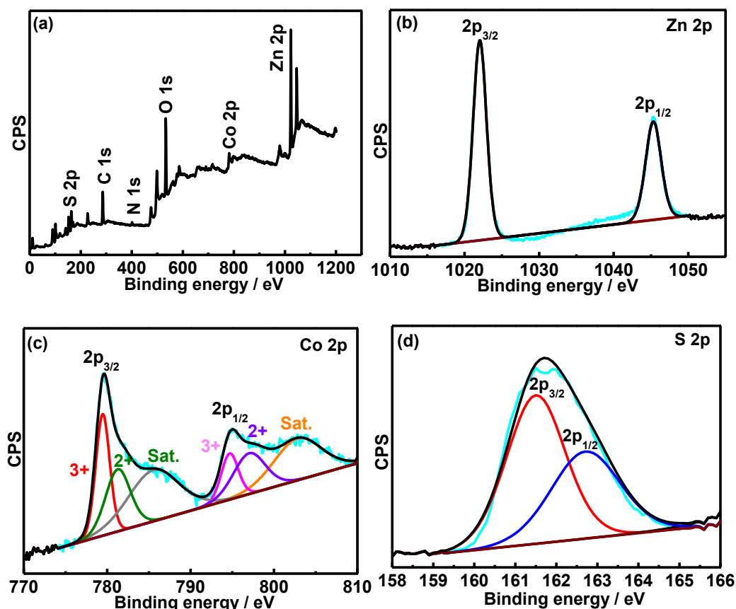
Figure 3.8: XPS analysis of Zn: Co (1:2) RT electrode material: (a) full spectrum, high resolution spectra of (b) Zn_{2p} , (c) Co_{2p} and (d) S_{2p} . “Sat.” in the Fig. 3.8 denotes satellite peaks.
