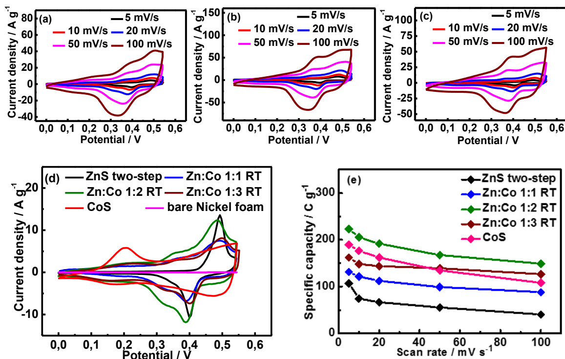
Figure 3.12: CV curves at different scan rates of ZnCoS RT electrodes, (a) Zn: Co (1:1) RT, (b) Zn: Co (1:2) RT, (c) Zn: Co (1:3) RT, (d) comparison of the CV curves recorded at a scan rate of 10 mV/s, (e) specific capacity at different scan rates.
