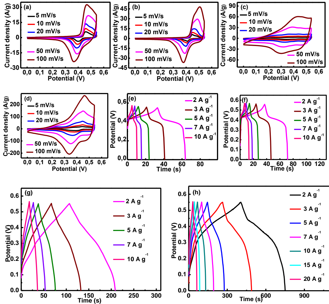
Figure 5.5: Electrochemical properties of Sb: Cr: Co electrode materials in 2 M KOH in the operating potential window (0 - 0.55 V): (a-d) CV curves of Sb: Cr: Co (1:0:0), (0:1:0), (0:0:1), (1:3:4) electrodes recorded at various scan rates (5 -100 mV/s); (e-h) GCD curves of Sb: Cr: Co (1:0:0), (0:1:0), (0:0:1), (1:3:4) electrodes acquired at different current densities (2-20 \text{A g}^{-1} );
