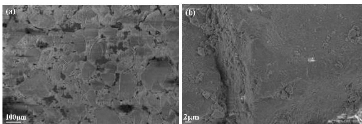
Figure 3.3: SEM images of the ZnS two-step at different magnifications.
