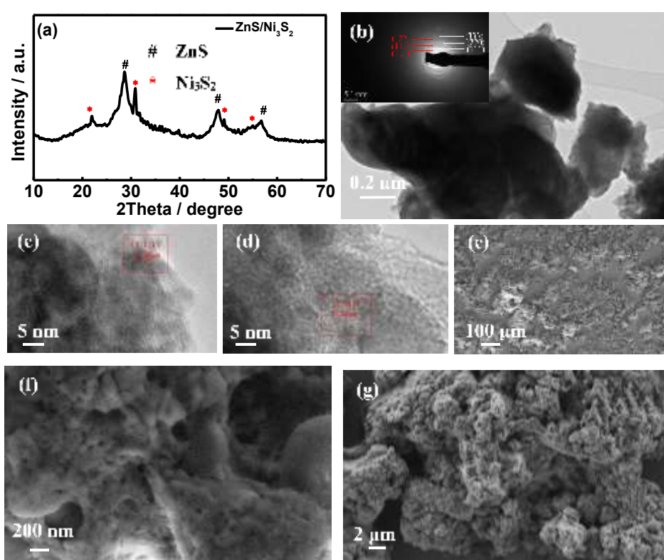
Figure 4.3: (a) XRD pattern, (b) TEM image, (c, d) HRTEM images and (e, f, g) SEM images of ZnS/Ni 3 S 2 ; the inset in (b) is the SAED pattern.
