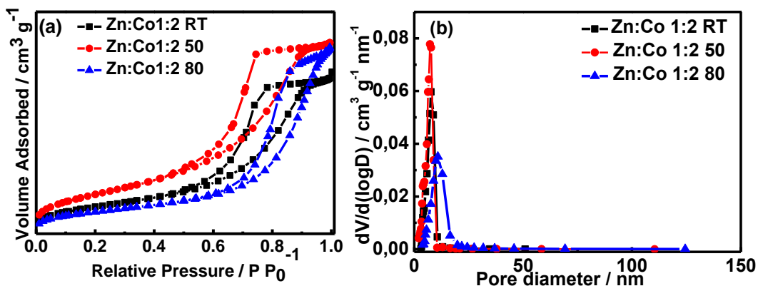
Figure 3.19: Nitrogen adsorption-desorption isotherms (a), and pore size distribution curves (b) of ZnCoS samples.
