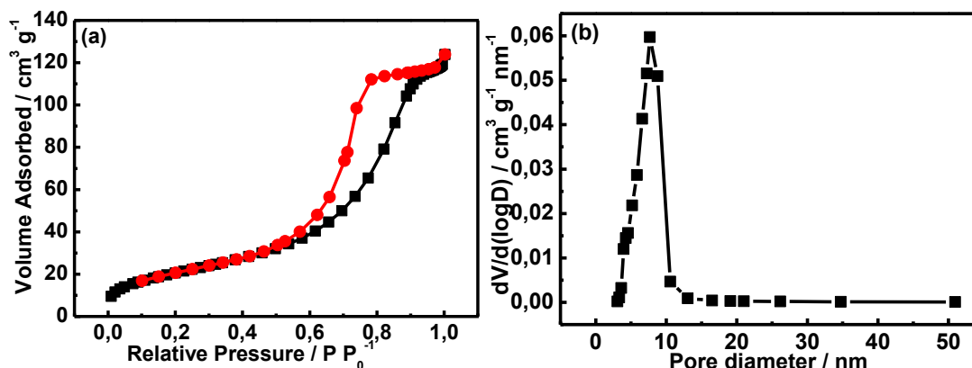
Figure 3.11: Nitrogen adsorption/desorption isotherm (a), and pore size distribution curve (b) of Zn: Co (1:2) RT electrode material.
