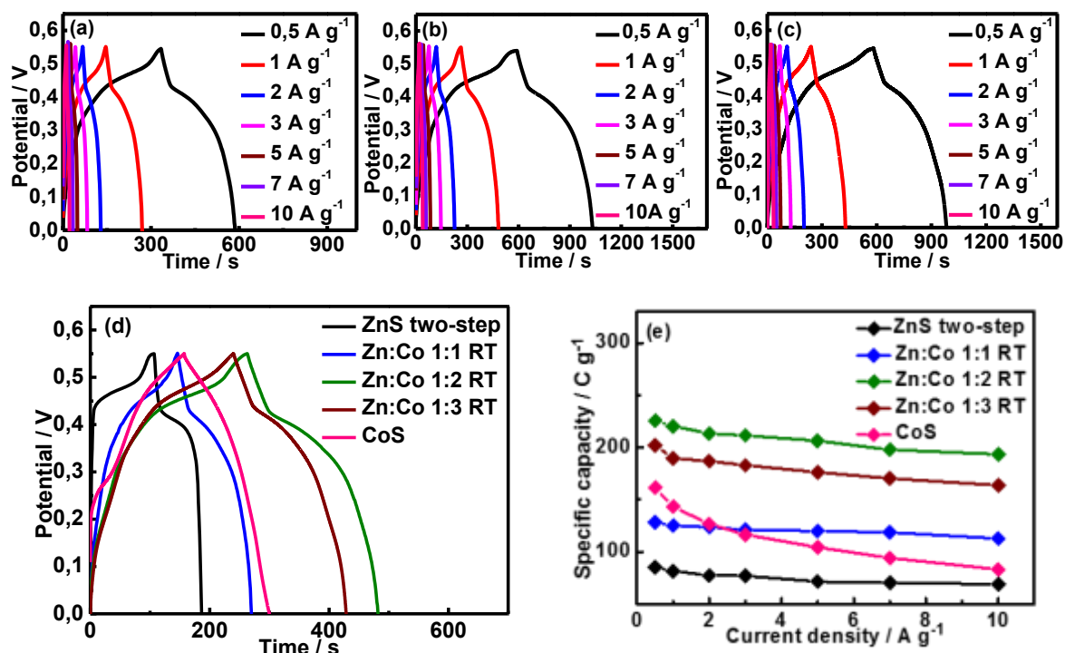
Figure 3.13: GCD curves of ZnCoS RT electrodes at different current densities. (a) Zn: Co (1:1) RT, (b) Zn: Co (1:2) RT, (c) Zn: Co (1:3) RT, (d) comparison of GCD curves at a current density of 1 \text{ A g}^{-1} , (e) specific capacity at different current densities.
