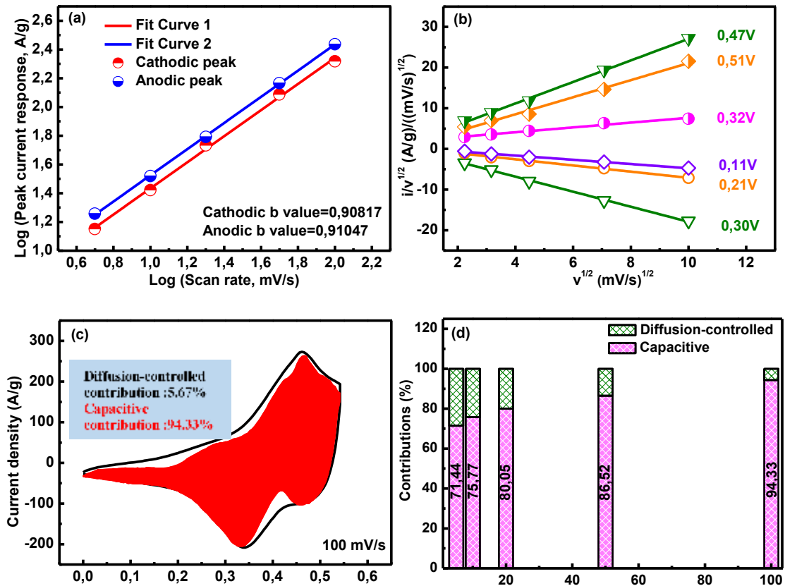
Figure 5.7: log (scan rate) - log (cathodic or anodic peak current response) of Sb: Cr: Co (1:3:4) electrode (a), fitting linear relationship between i/v^{1/2} vs. v^{1/2} used to calculate values of k_1 at different potentials (b), CV curves of the Sb: Cr: Co (1:3:4) electrode at a scan rate of 100 mV/s, the shaded area represents the capacitive contribution (c), the normalized contribution ratio of capacitive and diffusion-controlled charge storage of the Sb: Cr: Co (1:3:4) electrode at different scan rates (d).
