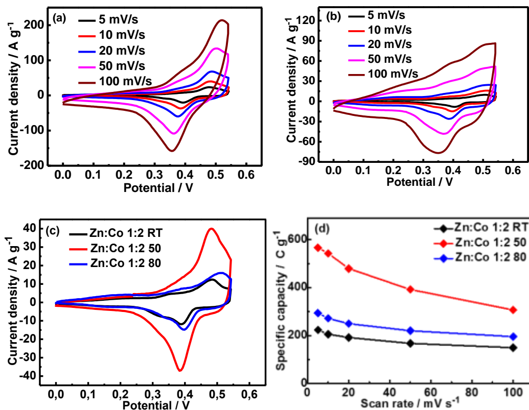
Figure 3.20: CV curves acquired at different scan rates of ZnCoS (1:2) electrodes. (a) Zn: Co (1:2) 50, (b) Zn: Co (1:2) 80, (c) comparison of the CV curves at a scan rate of 10 mV/s, (d) specific capacity at different scan rates.
