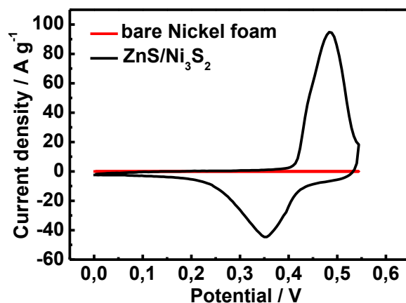
Figure 4.6: CV curves of ZnS/Ni 3 S 2 electrodes and bare nickel foam at a scan rate of 10 mV s -1 in the potential range of 0 to +0.55 V.
