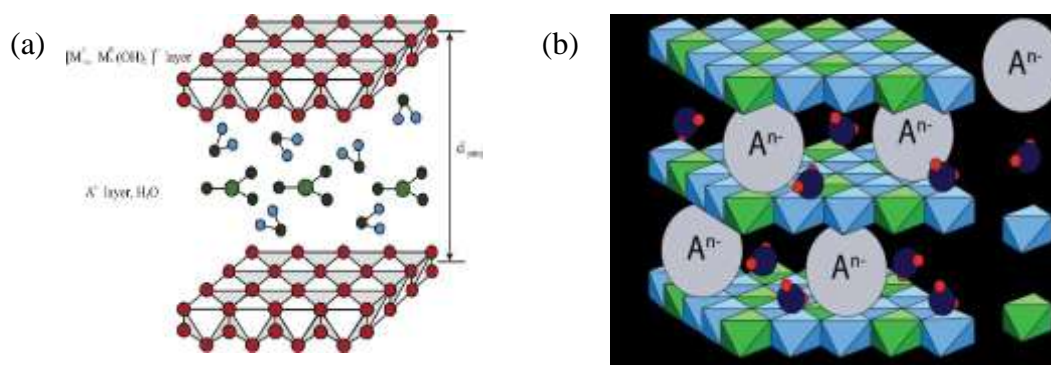
Figure 1.11: Hydrotalcite-like (a), and brucite-like (b) structures [62, 63].
