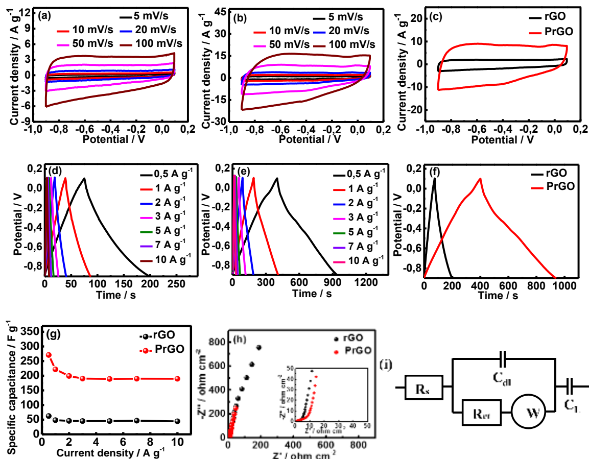
Figure 3.26: Electrochemical properties of rGO and PrGO in 2 M KOH: CV curves of rGO (a) and PrGO (b), CV curves of rGO and PrGO electrodes at a scan rate of 50 \text{ mV s}^{-1} in the potential range of -0.9 to +0.1 \text{ V} (c); GCD plots of rGO (d) and PrGO (e), GCD plots of rGO and PrGO electrodes at a current density of 0.5 \text{ A g}^{-1} in the potential range of -0.9 to +0.1 \text{ V} (f); the corresponding specific capacitance values at different current densities ( 0.5 - 10 \text{ A g}^{-1} ) (g); Nyquist plots (h), and the corresponding equivalent circuit (i).
