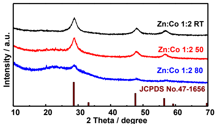
Figure 3.17: XRD patterns of the prepared Zn: Co (1:2) electrode materials at different temperatures during the precipitation process.
