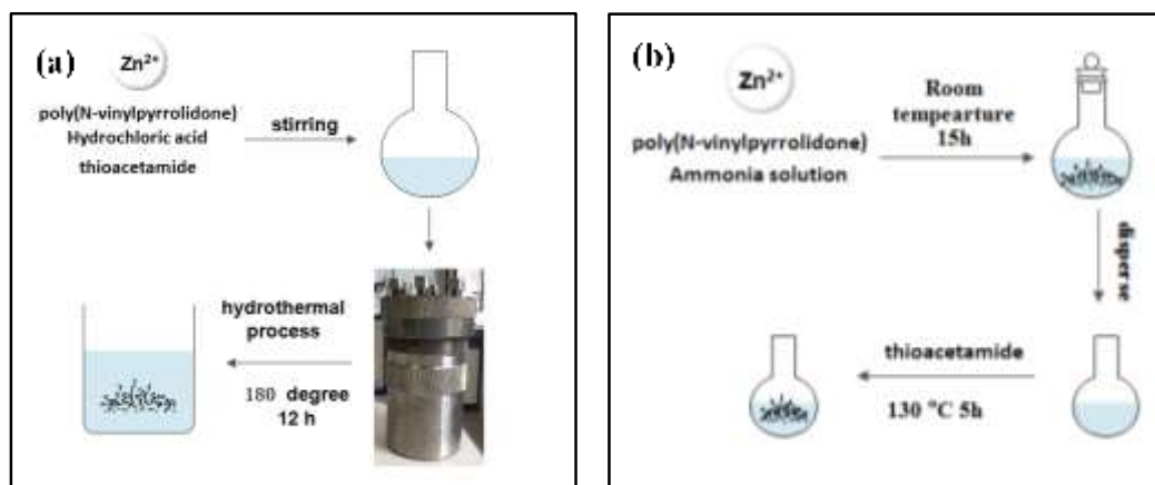
Figure 3.1: Illustration of the synthesis route of ZnS electrode materials, (a) one-step hydrothermal method, (b) two-step ion-exchange sulfurization method.
