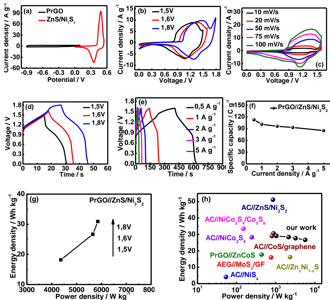
Figure 4.9: (a) CV curves of the positive and negative electrodes at a scan rate of 10 \text{ mV s}^{-1} ; (b) CV curves recorded at different cell voltages; (c) CV curves at different scan rates; (d) GCD curves recorded at different cell voltages; (e) GCD plots recorded as a function of current density; (f) the corresponding specific capacity as a function of current density; (g) the corresponding Ragone plot of the hybrid supercapacitor for different cell voltages (current density = 5 \text{ A g}^{-1} ); (h) typical Ragone plot of the hybrid supercapacitor.
