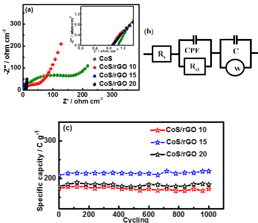
Figure 2.9: Nyquist plots of all CoS/rGO electrodes (a), the corresponding equivalent circuit (b), stability performance of all CoS/rGO electrodes at 5 \text{ A g}^{-1} in 2M KOH for 1,000 cycles (c).
