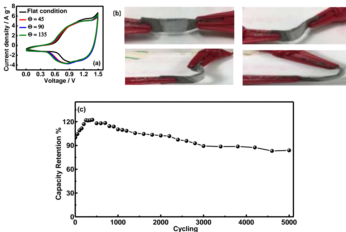
Figure 3.29: CV curves of the ASC at 50 mV/s under different bending angles of 0-135 ° in 2 M KOH solution (a), images of the bent cells (b), cycling performance of the fabricated flexible ASC device at 2 A g -1 for 5,000 cycles (c).
