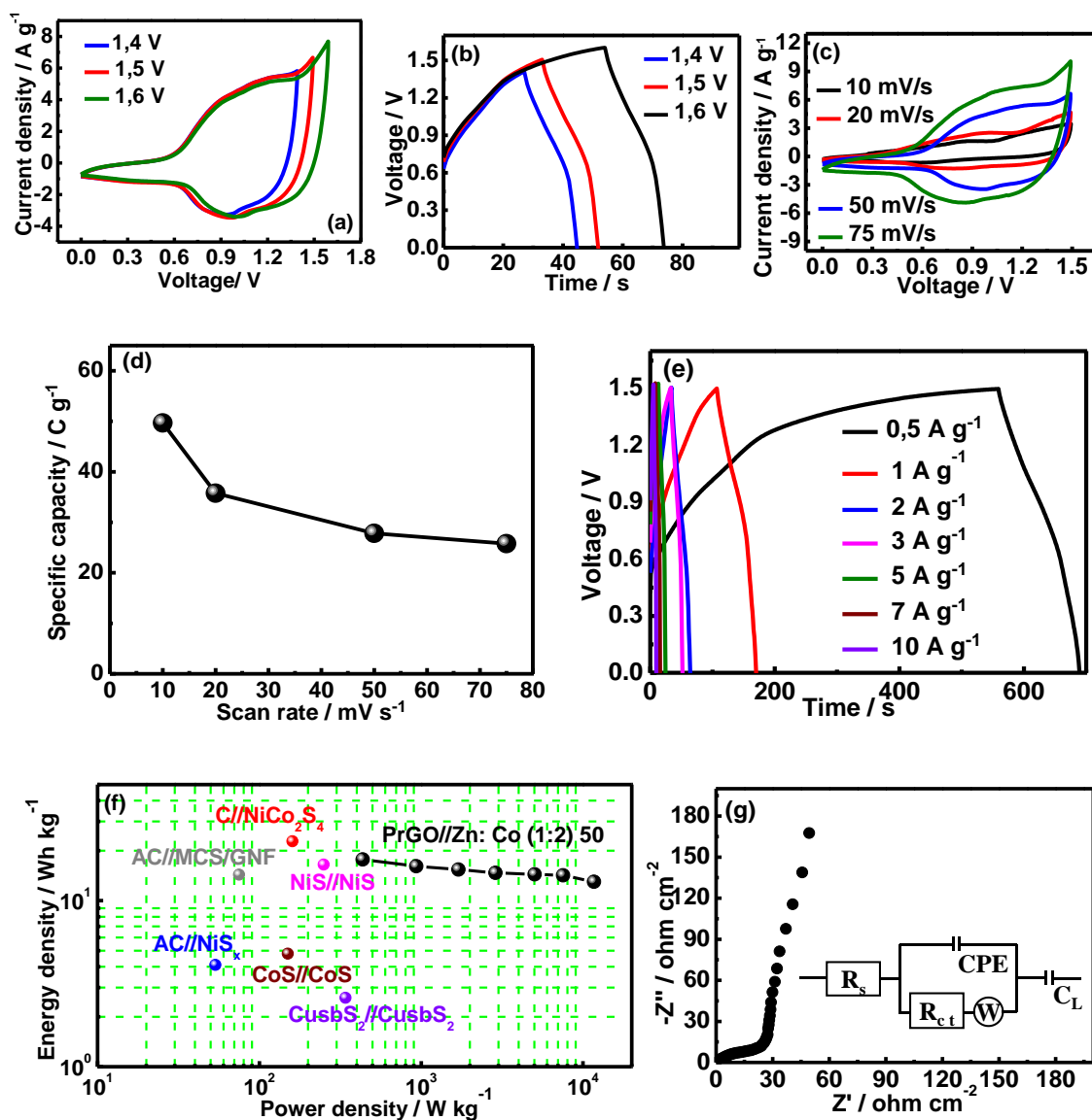
Figure 3.28: (a) CV and (b) GCD curves at different cell voltage values, (c) CV curves at various scan rates, (d) variation of the specific capacity as a function of scan rate, (e) GCD curves at various current densities, (f) typical Ragone plot, (g) Nyquist plot of the fabricated asymmetric supercapacitor device, the inset in (g) is the corresponding equivalent circuit.
