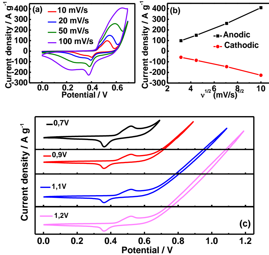
Figure 4.5: Electrochemical properties of ZnS/Ni 3 S 2 electrode within the potential range of 0 to +0.7 V in 2 M KOH: (a) CV curves, (b) the anodic and cathodic peak current densities vs. the square root of scan rate, (c) CV curves of ZnS/Ni 3 S 2 electrodes recorded in different potential windows at a scan rate of 50 mV s -1 .
