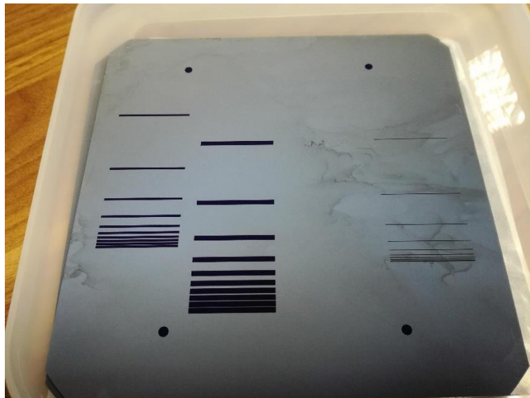
Figure 66: Picture of a sample with completely removed hot-melt after 1.5 minute in KOH free etchant with ultrasounds (35kHz)
