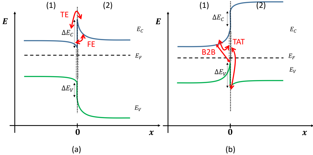
Figure 27: n/n (a) and n/p (b) heterojunctions
