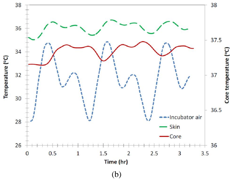
Figure 2.8: (a) Metabolic and evaporative heat rates and (b) incubator and baby temperature variation in time (modified from Dane and Sauer [30])
