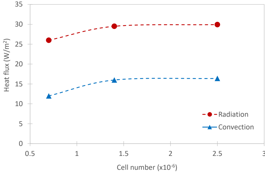
Figure 4.3: Mesh sensitivity for the body radiative and convection heat fluxes.
