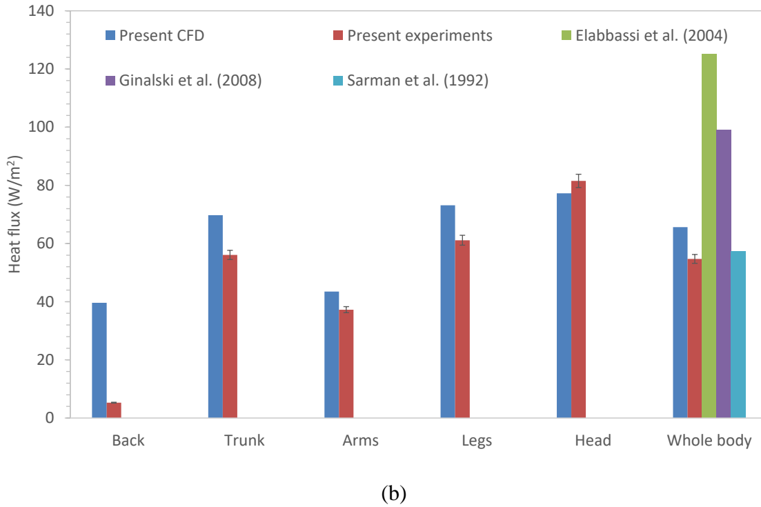
Figure 5.14: Total heat flux for the different body segments compared to CFD data and to values from the open literature: (a) cool incubator at 30°C and (b) warm incubator at 35°C.
