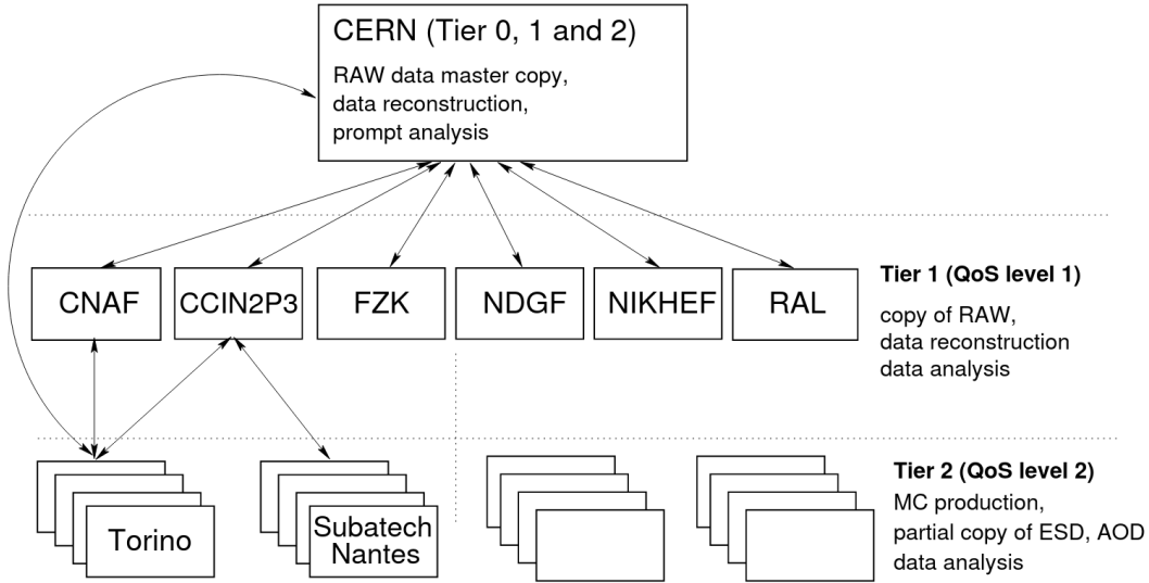
Figure 6.9: Schematic view of the computing grid hierarchy in the framework of the tiered MONARC model. Figure taken from Ref. [236].
