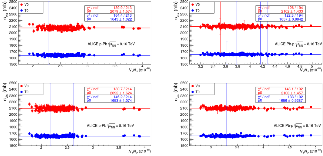
Figure 4.6: Visible cross sections for the V0 (red) and T0 (blue) processes measured in vdM scans in p–Pb (left) and Pb–p (right) collisions at \sqrt{s_{NN}} = 8.16 TeV, as a function of the product of the colliding bunches intensities. The top and bottom plots correspond to two different scans, the solid line is a constant fit to the data. Figure taken from [196].
