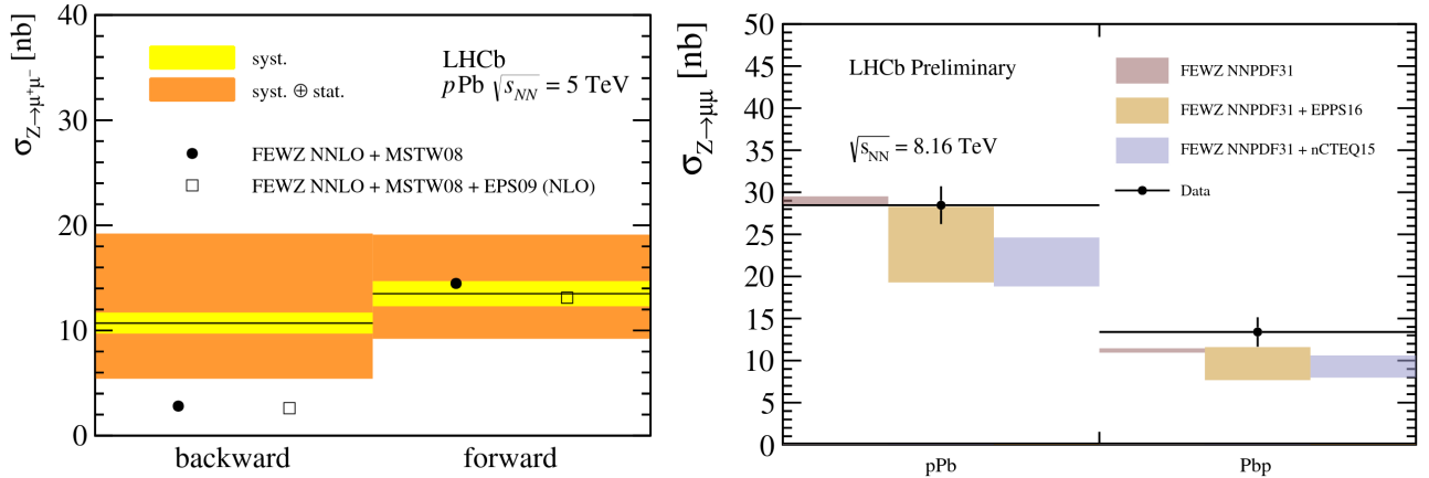
Figure 3.13: Left: Z^0 -boson cross section measured in p–Pb collisions at \sqrt{s_{NN}} = 5.02 TeV by the LHCb Collaboration, at backward and forward rapidities. The inner bands represent the systematic uncertainty, while the outer ones indicate the statistical and systematic uncertainties summed in quadrature. The measurements are compared with predictions from the MSTW2008 [177] PDF set, with and without including the nuclear corrections using EPS09 [98]. The uncertainties on the theoretical predictions are negligible compared to those on the experimental results, they are therefore not shown. Figure taken from Ref. [172]. Right: same measurements from p–Pb collisions at \sqrt{s_{NN}} = 8.16 TeV. The error bars correspond to the total uncertainty. Predictions from the NNPDF3.1 [49] free-PDF set are shown, along with calculations including the nuclear corrections from the EPPS16 [54] and nCTEQ15 [55] models. Figure taken from Ref. [173].
