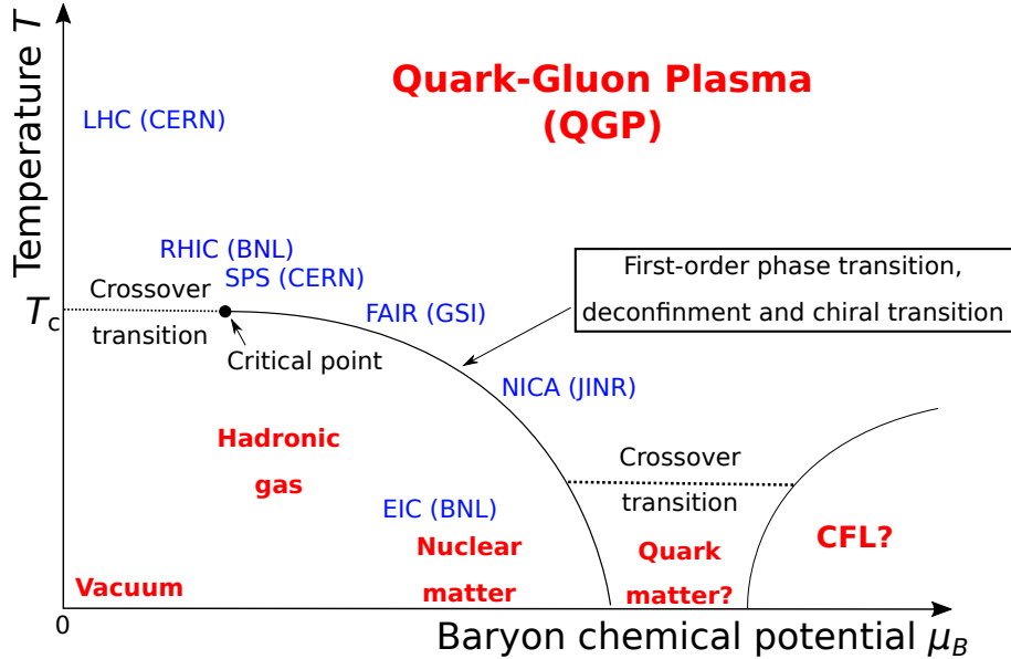
Figure 1.3: Schematic view of the phases of the QCD matter in the plane of temperature T and baryon-chemical potential \mu_B . The various phases, observed or predicted, are reported on the figure. The lines indicate the phase transitions, while the critical point is reported as a circle. The dashed lines correspond to expected crossovers. LHC, RHIC, SPS, FAIR, NICA, and EIC are the acronyms of the heavy-ion collision experiments described in Section 2.2.
