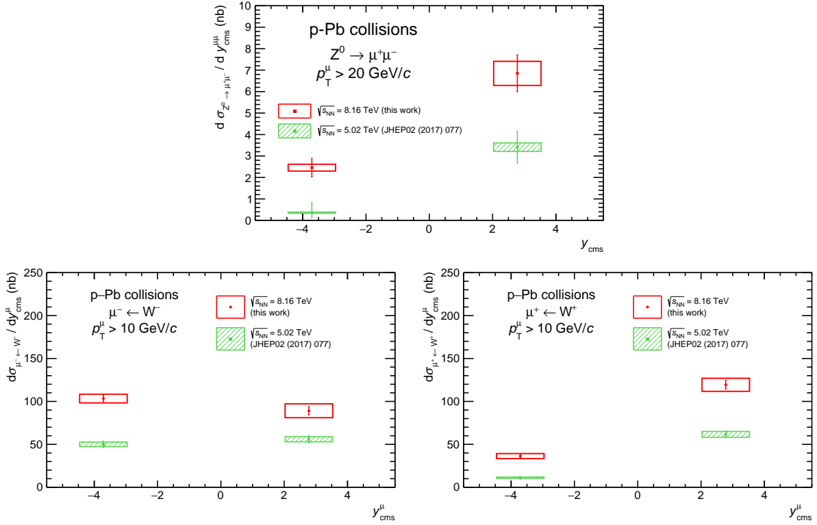
Figure 9.2: Production cross sections of the muonic decays of Z^0 (top), W^- (bottom left) and W^+ (bottom right) bosons measured in p–Pb collisions at \sqrt{s_{\text{NN}}} = 8.16 TeV (this work) and \sqrt{s_{\text{NN}}} = 5.02 TeV from Ref. [156]. The bars and boxes indicate the statistical and systematic uncertainties, respectively.
