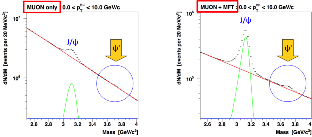
Figure 7.10: Dimuon invariant mass distribution in the J/\psi family region for p_T^{\mu\mu} < 10 GeV/ c , in Pb–Pb collisions, without (left) and with (right) including information from the MFT.
