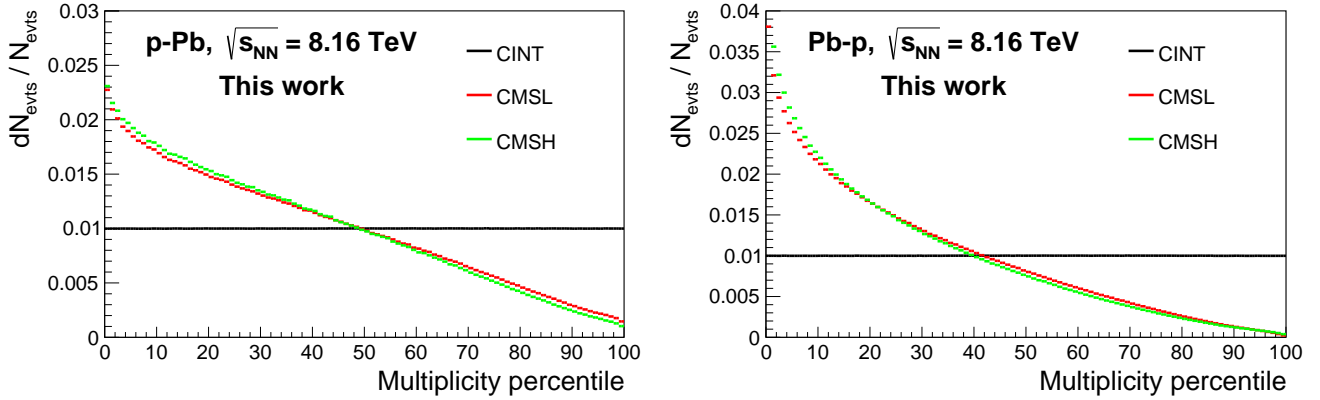
Figure 8.3: Multiplicity distribution of MB, MSL and MSH triggered events measured by VOM in p–Pb (left) and Pb–p (right) collisions.
