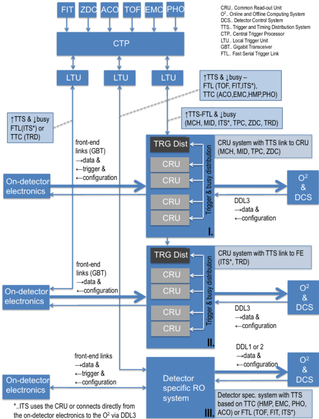
Figure 7.4: Upgraded readout scheme of ALICE. Configuration I: CRU is used as readout processor and trigger distribution system. Configuration II: CRU is used as readout processor, the trigger distribution is done from the CTP/LTU directly to the on-detector electronics. Configuration III: CRU is not used as the detectors do not upgrade their electronics and use detector-specific readout systems. Figure taken from Ref. [252].
