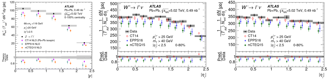
Figure 3.9: Normalised yields of the Z^0 (left), W^+ (middle) and W^- (right) bosons as a function of the absolute rapidity ( Z^0 ) or pseudorapidity ( W^\pm ) measured in Pb–Pb collisions at \sqrt{s_{\text{NN}}} = 5.02 TeV by the ATLAS Collaboration. The bars and boxes correspond to the statistical and systematic uncertainties, respectively. The measurement are compared with predictions from the EPPS16 [54] and nCTEQ15 [55] nPDF models, as well as prediction from the free-nucleon CT14 [63] PDF, accounting the isospin but without nuclear modifications. The bottom panels show the ratios of the predicted yields to the measured ones. Figures taken from Refs. [163, 164].
