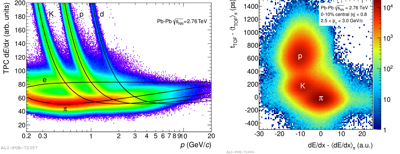
Figure 4.12: Left: Specific energy loss dE/dx in the TPC as a function of the particle momentum, in Pb–Pb collisions at \sqrt{s_{NN}} = 2.76 TeV. The lines correspond to parametrisations of the Bethe-Block equation. Right: K/\pi separation by combining the arrival time measurement in TOF and dE/dx in the TPC. Figures taken from Ref. [185].
