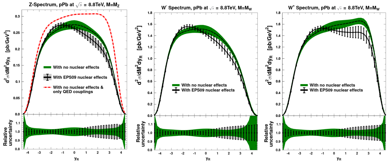
Figure 3.7: Production cross section of the Z^0 (left), W^- (middle) and W^+ (right) bosons in p–Pb collisions at \sqrt{s_{\text{NN}}} = 8.8 TeV, calculated at the boson pole mass M^2 = M_{Z^0, W^\pm}^2 . The dashed line and green uncertainty band correspond to predictions with the CTEQ6.6 [154] PDF set, without application of nuclear modifications. The full line corresponds to predictions with the CTEQ6.6 PDF, modified by the EPS09 [98] parametrisation of the nuclear modifications. The black vertical lines indicate the uncertainty from the nPDF. The lower panels show the relative uncertainties with the same colour code. The red dashed curve superimposed to the Z^0 distribution correspond to the cross section for virtual photon exchange only. The abscissae are labelled y_R to indicate that the rapidity is the boson one, in the absence of final state radiations. Figures taken from Ref. [153].
