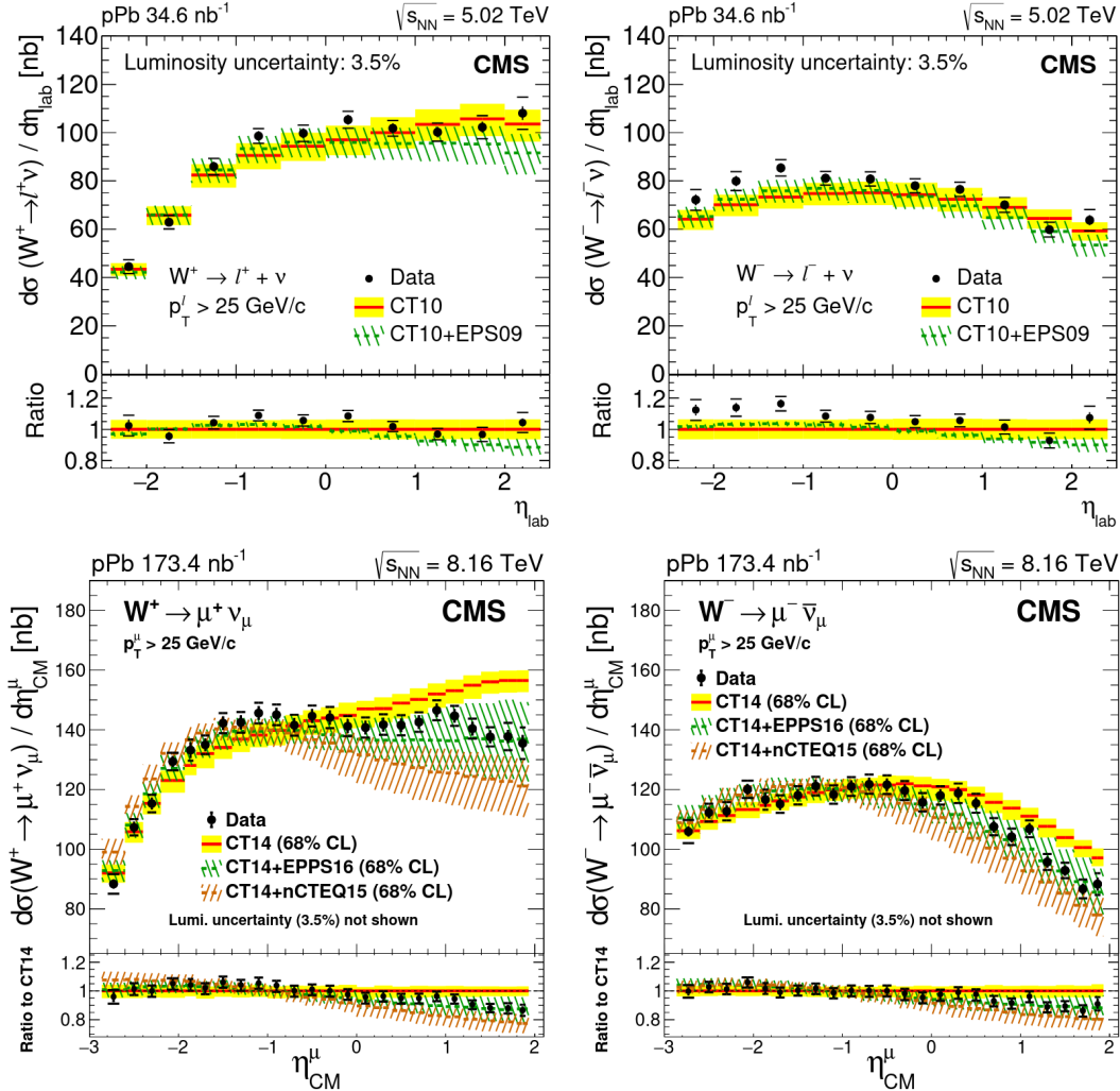
Figure 3.12: Production cross section of W^+ (left) and W^- (right), as a function of the lepton pseudorapidity, in p–Pb collisions at \sqrt{s_{\text{NN}}} = 5.02 TeV (top) and 8.16 TeV (bottom) measured by the CMS Collaboration. The error bars represent the statistical uncertainty, while brackets show the statistical and systematic uncertainties summed in quadrature. The free-nucleon predictions from CT10 [176] and CT14 [63] are shown as full bands, the predictions including the nuclear corrections are displayed as dashed lines. They rely on the EPS09 [98], EPPS16 [54] or nCTEQ15 [55] parametrisation of the nPDFs. The bottom panels show the ratio of the data and nPDF calculations to that of the free-nucleon ones. Figures taken from [166, 167].
