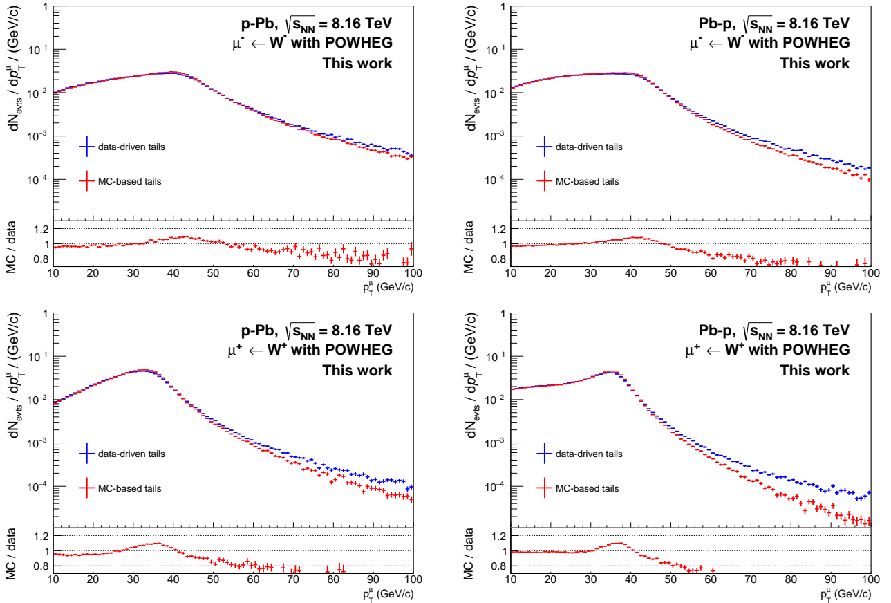
Figure 8.12: p_T distribution of negative (top) and positive (bottom) muon from W^{\pm} decays in p-Pb (left) and Pb-p (right) collisions simulated with the nominal (data-based) and alternative (MC-tuned) sets of parameters for the cluster resolution correction. The bottom panel in each plot shows the ratio of the distribution obtained with the alternative set to that with the nominal one.
