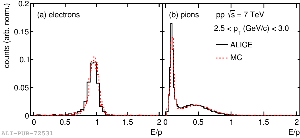
Figure 4.14: E/p distribution for electrons (left) and pions (right) in the EMCAL, in pp collisions at \sqrt{s} = 7 TeV. The samples of identified electrons and pions are obtained from \gamma conversion and \Lambda/K_S^0 decays respectively. The dotted lines correspond to Pythia simulations of each processes, with realistic detector configuration and full reconstruction. Figure taken from Ref. [185].
