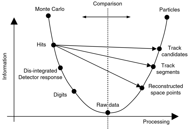
Figure 6.11: Schematic depiction of the data processing framework in AliRoot. The vertical dashed line separates the simulation part (left) from the reconstruction one (right). The curve follows the full simulation and reconstruction chain, the arrows indicate the possibilities for fast simulations (see text for details). Figure taken from Ref. [188].
