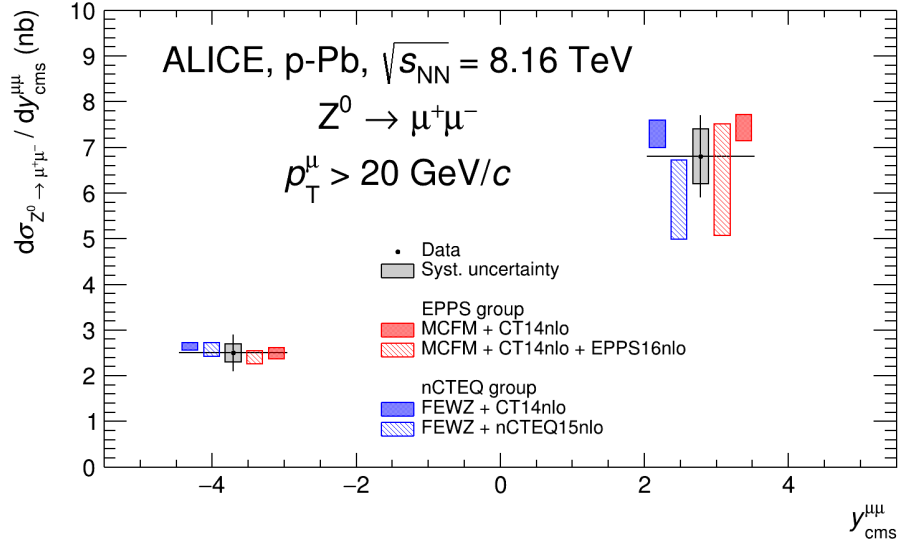
Figure 9.3: Production cross section of the Z^0 \rightarrow \mu^+\mu^- process in p–Pb collisions at \sqrt{s_{\text{NN}}} = 8.16 \text{ TeV} , compared with theoretical predictions with the EPPS16 [54] and nCTEQ15 [55] nPDF sets, as well as the free-nucleon CT14 PDF [63], accounting for the isospin effect but without nuclear modification of the PDF. The bars and boxes around the data points correspond to the statistical and systematic uncertainties. The theory points are horizontally shifted for better readability.
