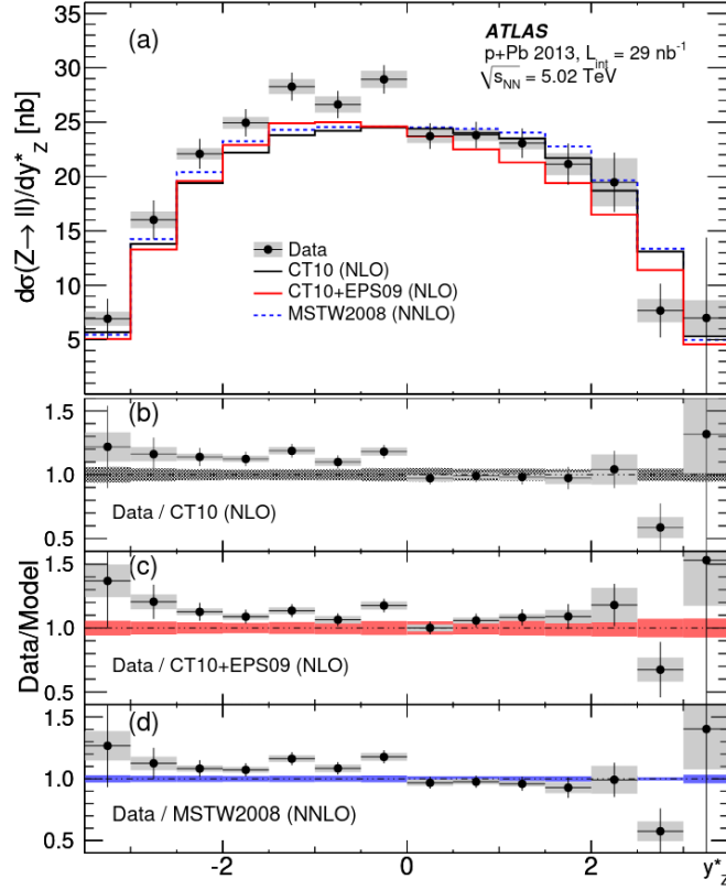
Figure 3.11: Rapidity-differential cross section of the Z^0 detected in the leptonic decay channel ( e + \mu ) in p-Pb collisions at \sqrt{s_{NN}} = 5.02 TeV with the ATLAS detector. The bars and boxes indicate the statistical and systematic uncertainties, respectively. The measurements are compared with calculations with the CT10 [176] and MSTW2008 [177] free-nucleon PDF, and with the EPS09 [98] nPDF set, using CT10 as baseline. The bottom panels shows the ratio of the data to the various models. Figure taken from [160].
