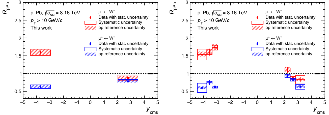
Figure 9.8: Nuclear modification factor R_{pPb} of muons from W^\pm decays measured in p–Pb collisions at \sqrt{s_{NN}} = 8.16 TeV, in the full acceptance of the muon spectrometer (left) and in various rapidity bins (right). The reference pp cross section is taken from calculations with the CT10 [176] proton PDF. The bars and open boxes indicate the statistical and systematic uncertainties on the cross section in p–Pb, respectively. The hashed boxes represent the uncertainty on the reference cross section. The systematic uncertainty on the luminosity is shown as a black box around the line R_{pPb} = 1 .
