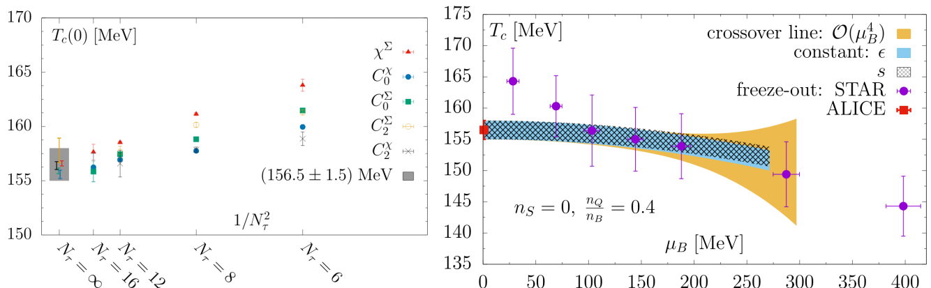
Figure 1.4: Left: pseudo-critical temperature T_c(0) as a function of the lattice volume N_\tau using several parametrisation of the chiral order parameter C^\Sigma , the disconnected chiral susceptibility C^X and the susceptibility of the chiral order parameter \chi^\Sigma . The solid grey band depicts the continuum extrapolated value. Right: phase boundary of 2 + 1 flavour QCD compared with the line of constant energy density \epsilon = (0.42 \pm 0.06) GeV/fm 3 and the line of constant entropy s = (3.7 \pm 0.5) fm -3 in the T - \mu_B plane. It is also compared with the chemical freeze-out parameters extracted from grand canonical ensemble based fits to hadron yields within 0–10% centrality class from ALICE and 0–5% centrality class from STAR. Figures taken from Ref. [29] where more details can be found.
