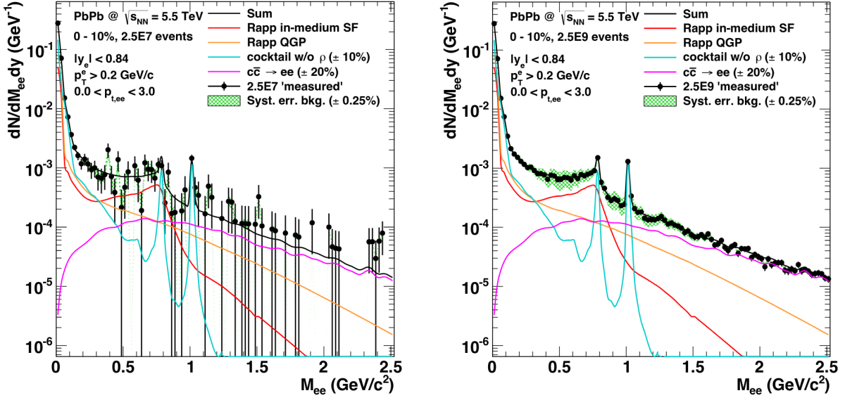
Figure 7.3: Simulations of the inclusive e^+ e^- invariant mass spectrum for the 10% most central events in Pb–Pb collisions at \sqrt{s_{\text{NN}}} = 5.5 TeV, assuming 2.5 \times 10^7 events (left) and 2.5 \times 10^9 events (right) corresponding to the collected data with the current and upgraded TPC, respectively. Figures taken from Ref. [247].
