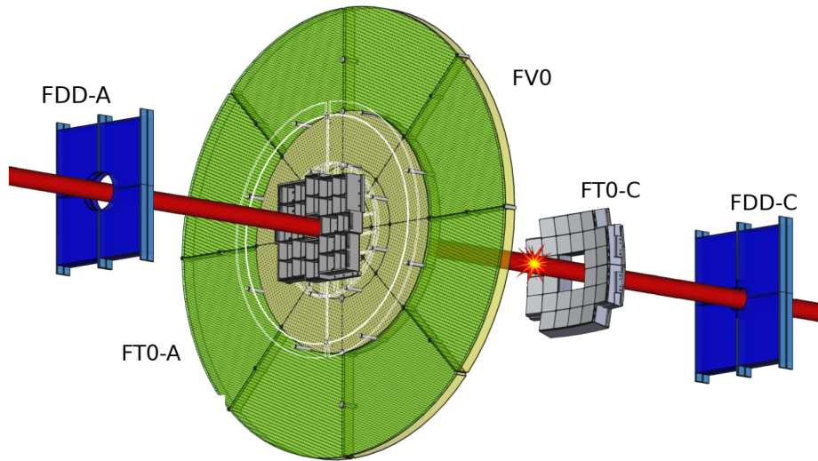
Figure 7.5: Schematics of the FIT layout, with the relative locations of the FV0, FT0 and FDD arrays (not to scale). Figure taken from Ref. [253].
