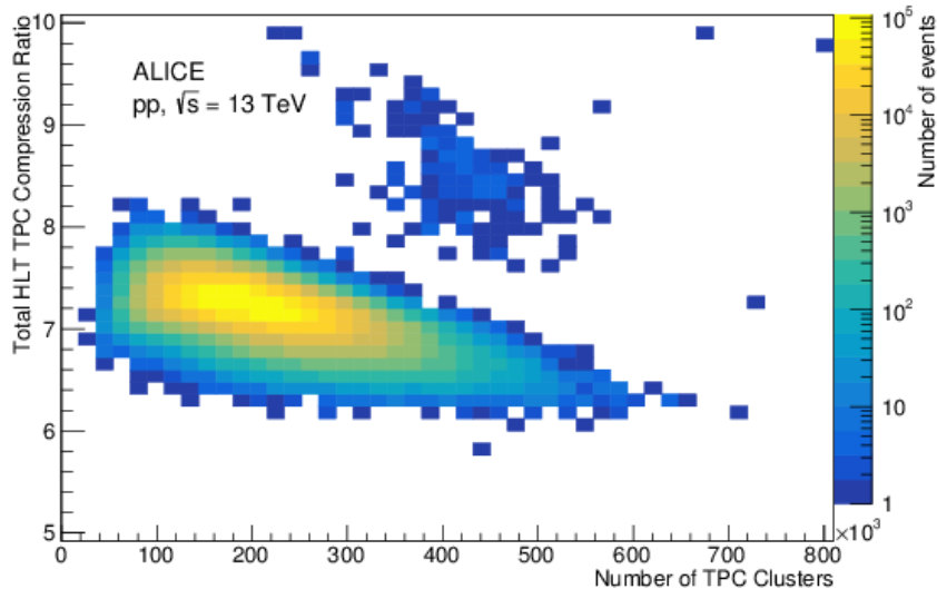
Figure 6.6: HLT compression factor achieved for TPC data, as a function of the input data size expressed in terms of the number of TPC clusters, in pp collisions at \sqrt{s_{\text{NN}}} = 13 TeV in 2017. The average compression factor over the whole period amounts to 7.3. Figure taken from Ref. [234].
