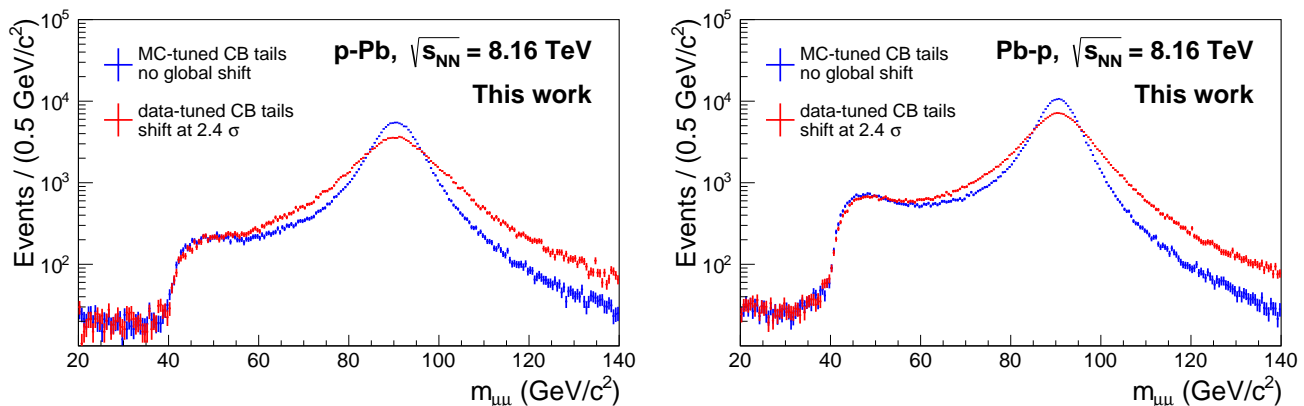
Figure 8.15: Invariant mass distribution of dimuons from Z^0 decays.
