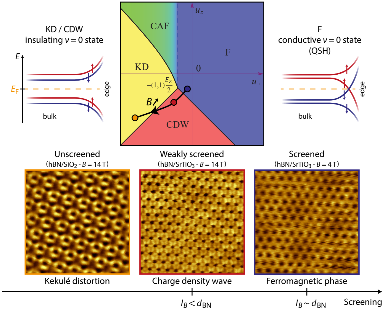
Figure 7.30: Model of a screening-induced quantum phase transition in charge-neutral graphene. For sample on hBN/SrTiO 3 , increasing the magnetic field lowers the efficiency of the substrate-screening of the Coulomb interaction. At low magnetic fields (strong screening), the conductive F phase appears as the usual honeycomb lattice. At high magnetic fields (weak screening), a charge-density wave emerges and charge-neutral graphene becomes weakly insulating. At very high magnetic fields (no screening), the \nu = 0 ground state transits to a Kekulé distortion of the honeycomb lattice with a strong insulating behavior.
