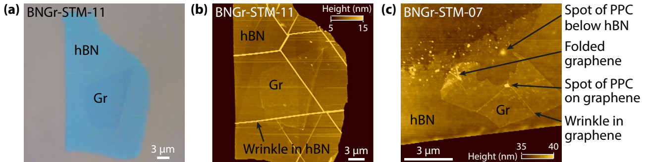
Figure B.12: BNGr stacks on \text{SiO}_2 after burning the PPC film. (a,b) Stack observed with an optical microscope (a) and with an AFM (b). The hBN flake is thin enough to see the graphene with the eye. The AFM reveals wrinkles in the hBN flake due to the annealing, but graphene is mostly clean. (c) Another stack observed with AFM, which unveils many defects, the main one being that the (originally rectangular) graphene flake has been torn apart and folded during the annealing. Many spots of PPC are also observable. The scale bar is the same in the three figures : 3 \mu\text{m} .
