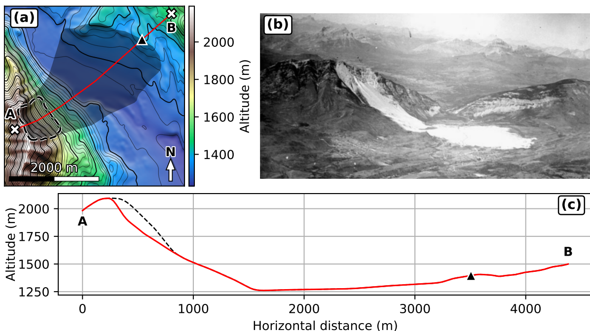
Figure 5.4: Frank Slide rock avalanche. (a) Post collapse topography with deposits removed, 20 m DEM. Black dashed outline: landslide scar. Dark area: observed landslide extent. Bold contour interval is 100 m. Red line: cross-section along which travel distances are measured. Black triangle: Observed travel distance. (b) Picture of the Frank Slide, taken in 1922 (Canada. Dept. of National Defence / Library and Archives Canada / PA-052095). (c) Cross-section along red line in (a). Red line: Post-collapse topography with deposits removed. Black dashed line: Reconstructed pre-collapse topography. Black triangle: observed deposit extent.
