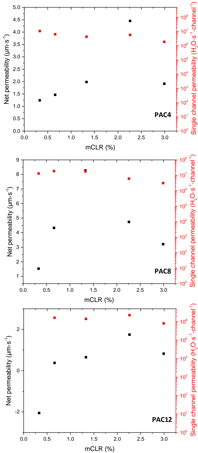
Figure S6. Net permeability and Single channel permeability of PAD4 , PAD8 , PAD12 channels at 200 mOsm osmolarity gradient
