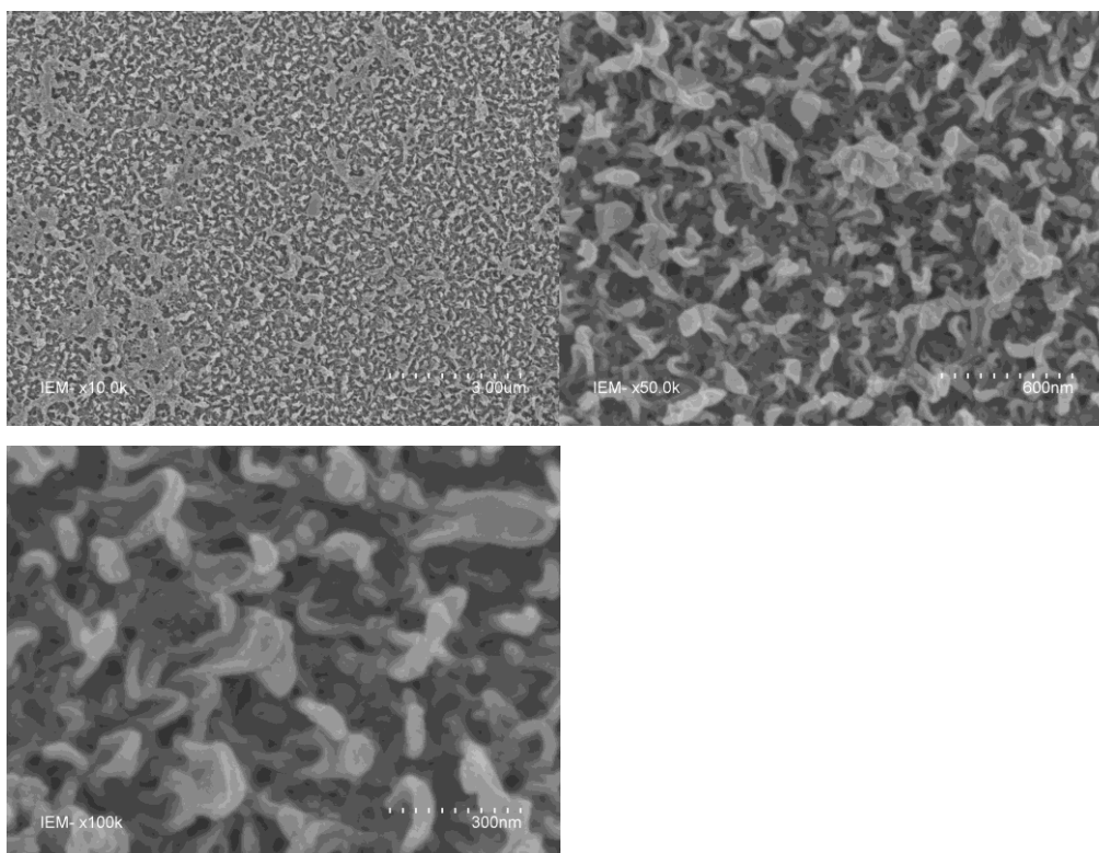
Figure S16. Surface SEM micrographs of PA-PA[5] membrane prepared using MPD-PA[5] 0.5% solution with Ethanol/Water ratio 1:2 (Membrane composition MPD 1.2 w/w %, TMC 0.1w/w %)
