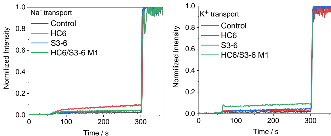
Figure S21. Comparison of cation transport activity expressed as normalized fluorescence intensity of 5 mM / 5 mM HC6/S3-6 system and individual compounds in the extra-vesicular medium containing 100 mM NaCl(left) or KCl (right).
