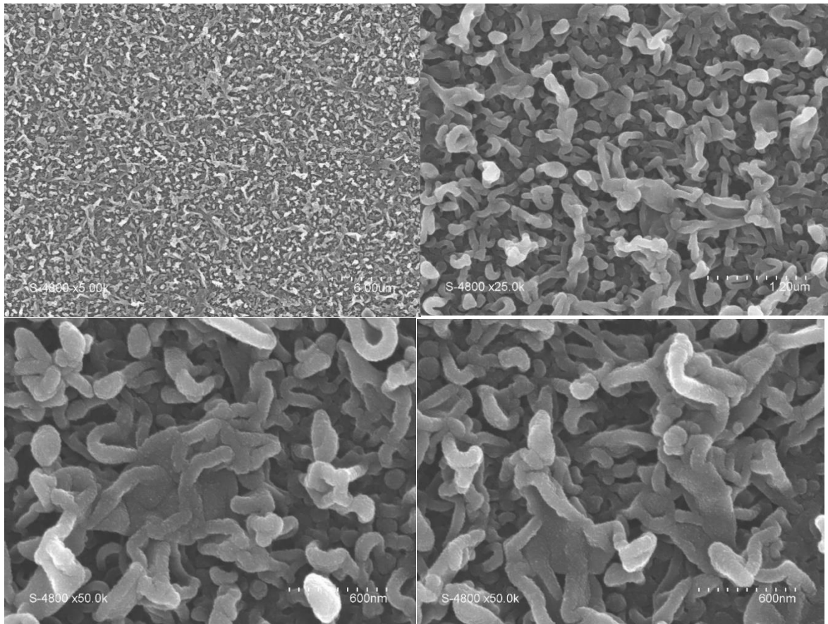
Figure S8. Surface SEM micrographs of PA-PA[5] membrane prepared using PA[5] 0.025% solution (membrane composition MPD 1.2 w/w % and TMC 0.1w/w %).
