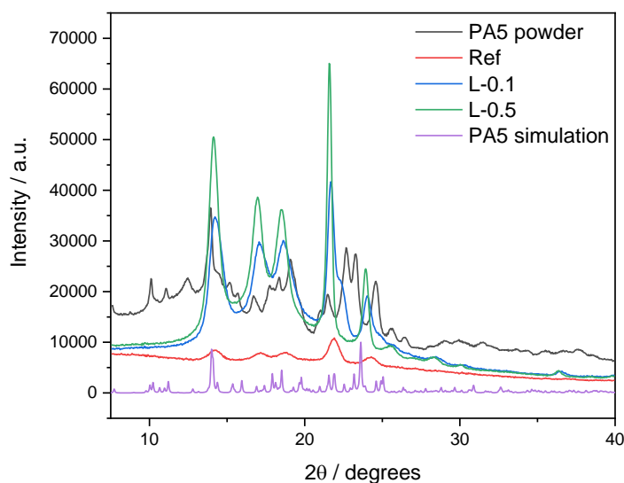
Figure S19. X-Ray diffraction comparison of PA5 powder, Reference TFC membrane, L-0.1 and L-0.5 membranes prepared using 0.1 w/w % and 0.5 w/w % PA5 solutions respectively.
