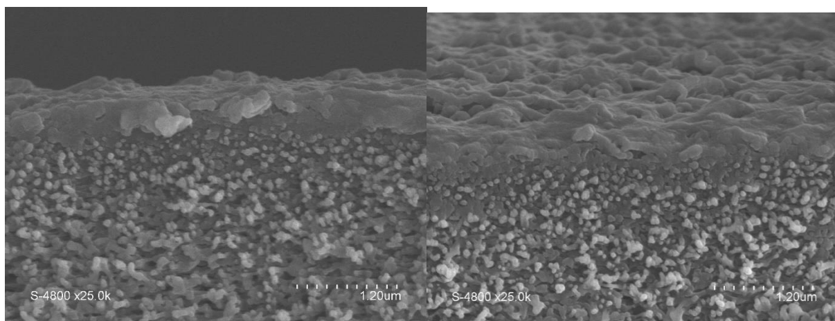
Figure S9. Cross-section SEM micrographs of PA-PA[5] membrane prepared using PA[5] 0.025% solution (membrane composition MPD 1.2 w/w % and TMC 0.1w/w %).
