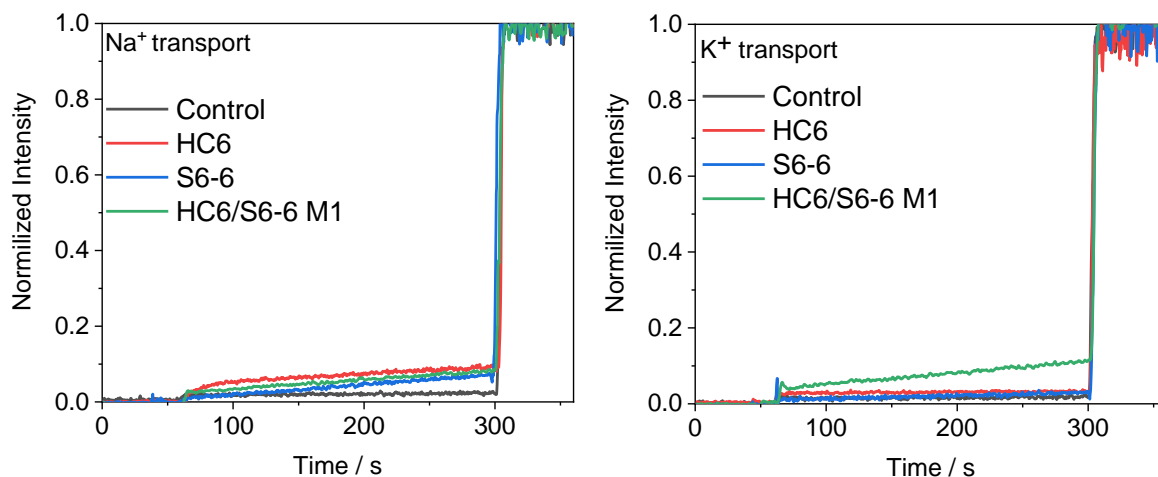
Figure S23. Comparison of cation transport activity expressed as normalized fluorescence intensity of 5 mM / 5 mM HC6/S6-6 system and individual compounds in the extra-vesicular medium containing 100 mM NaCl(left) or KCl (right).
