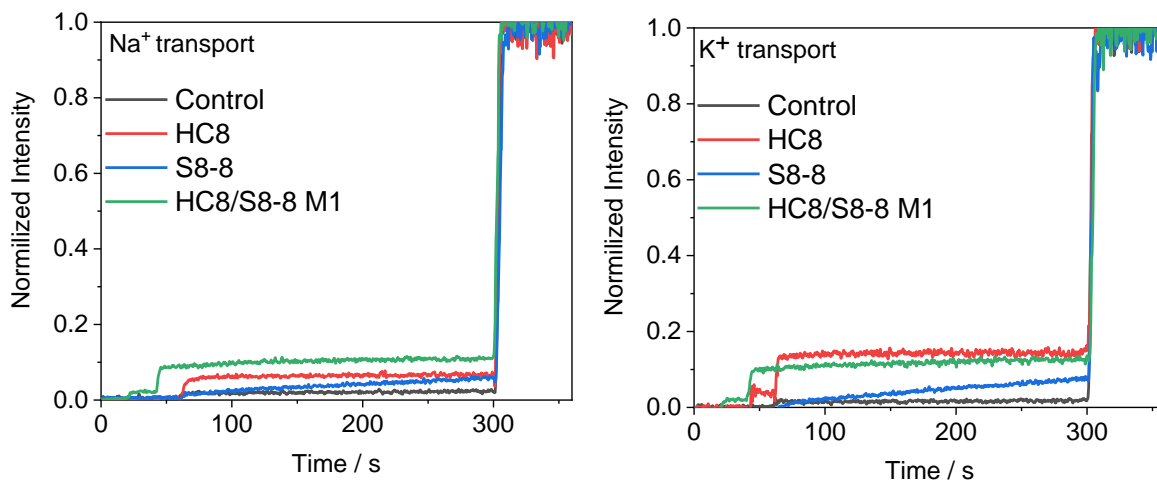
Figure 28. Comparison of cation transport activity expressed as normalized fluorescence intensity of 5 mM / 5 mM HC8/S8-8 system and individual compounds in the extra-vesicular medium containing 100 mM NaCl(left) or KCl (right).
