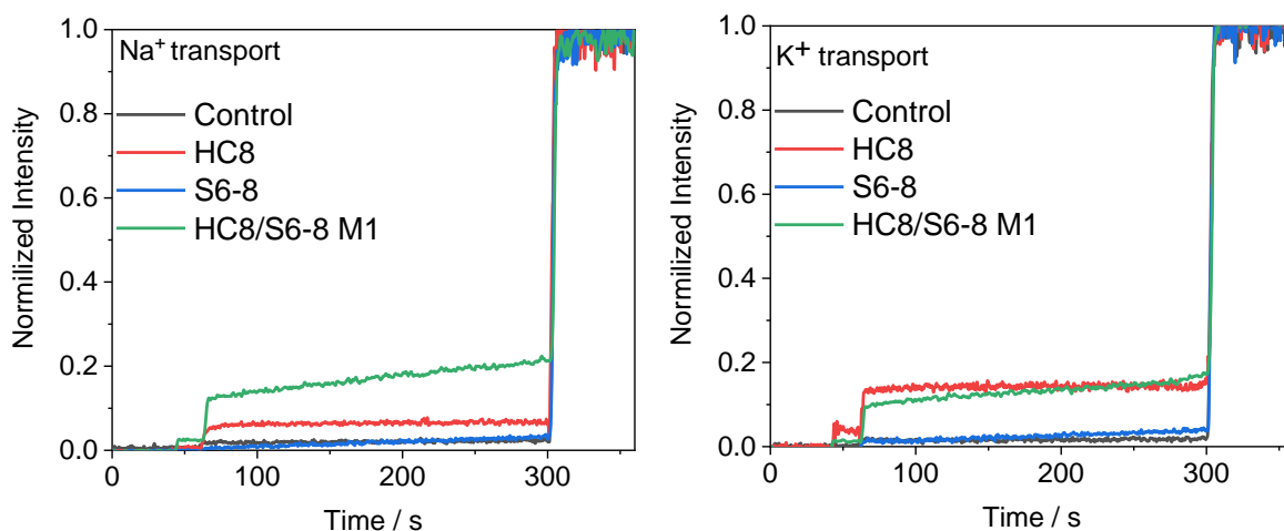
Figure 26. Comparison of cation transport activity expressed as normalized fluorescence intensity of 5 mM / 5 mM HC8/S6-8 system and individual compounds in the extra-vesicular medium containing 100 mM NaCl(left) or KCl (right).
