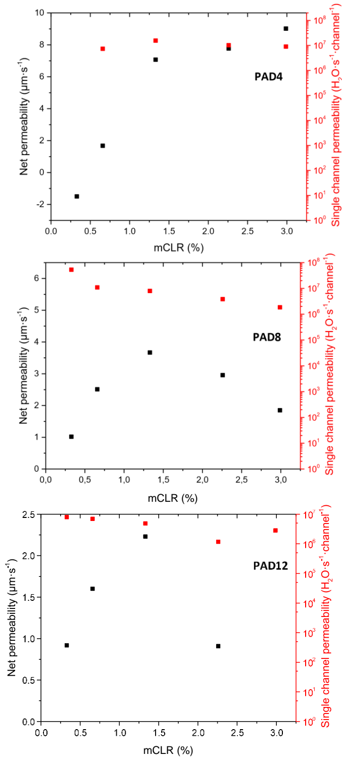
Figure S5. Net permeability versus Single channel permeability of PAD4 , PAD8 , PAD12 channels at 100 mOsm osmolarity gradient
