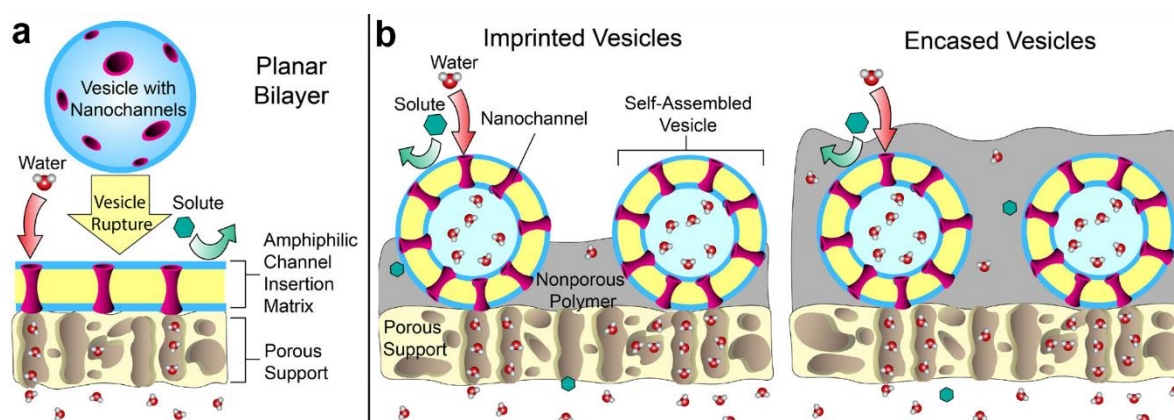
Figure 13. Design considerations for common biomimetic membrane formation strategies. (a) Pore-spanning planar layer format. (b) Vesicle-encapsulated mixed-matrix formats. Image adapted from reference [76].
