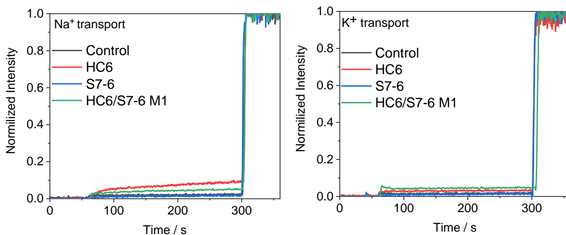
Figure S24. Comparison of cation transport activity expressed as normalized fluorescence intensity of 5 mM / 5 mM HC6/S7-6 system and individual compounds in the extra-vesicular medium containing 100 mM NaCl(left) or KCl (right).
