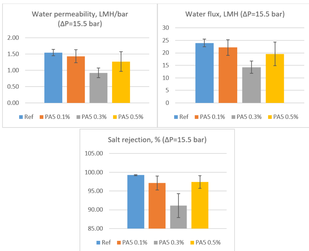
Figure S20. Water permeability, flux and salt rejection for the reference membrane REF and PA5 membranes prepared with 0.1%, 0.3% and 0.5% Pillar[5]arene solutions (w/w); membrane composition MPD 1.5 w/w % and TCM 0.15 w/w %.
