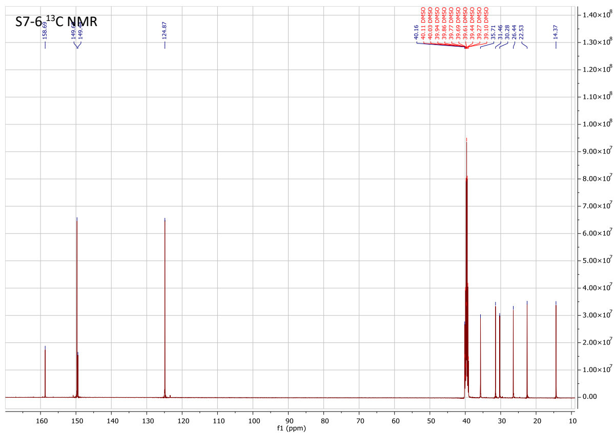
Figure S13. 1 H NMR (top) and 13 C NMR (bottom) spectra of S7-6
