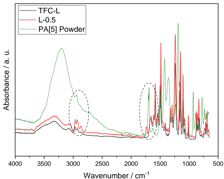
Figure S3. Comparison of FTIR-ATR spectra of PA[5] membrane with 0.5% PA[5] and the reference TFC membrane (membrane composition MPD 1.2 w/w % and TMC 0.1w/w %).
