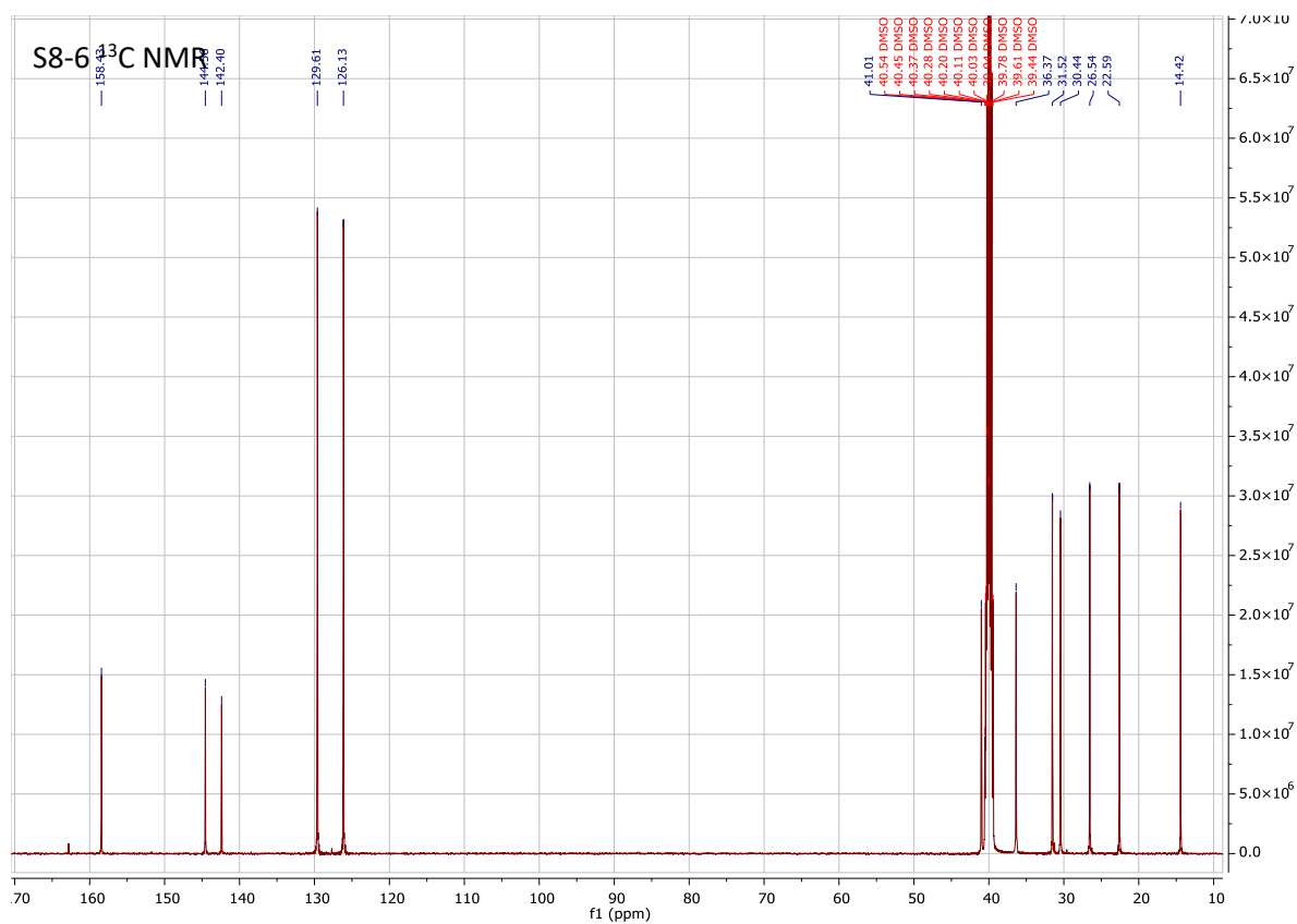
Figure S15. ^1\text{H} NMR (top) and ^{13}\text{C} NMR (bottom) spectra of S8-6
