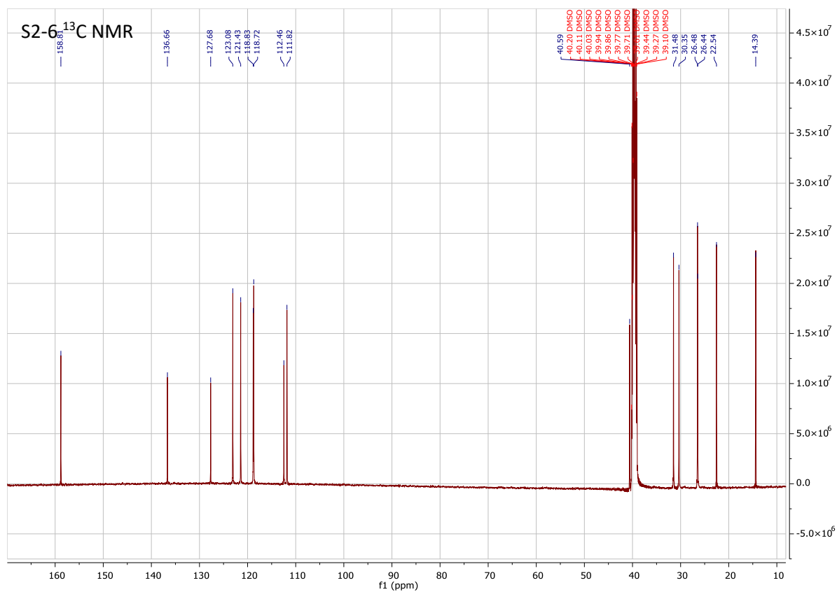
Figure S3. 1 H NMR (top) and 13 C NMR (bottom) spectra of S2-6
