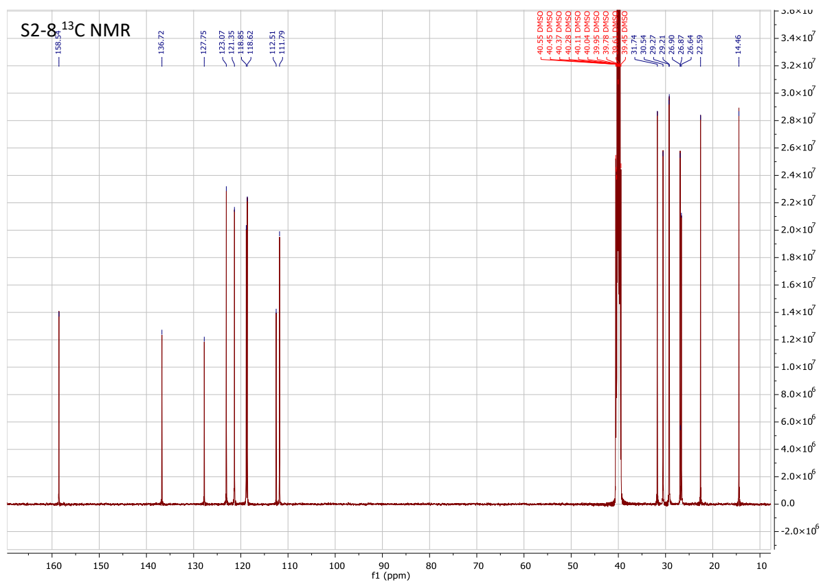
Figure S4. 1 H NMR (top) and 13 C NMR (bottom) spectra of S2-8
