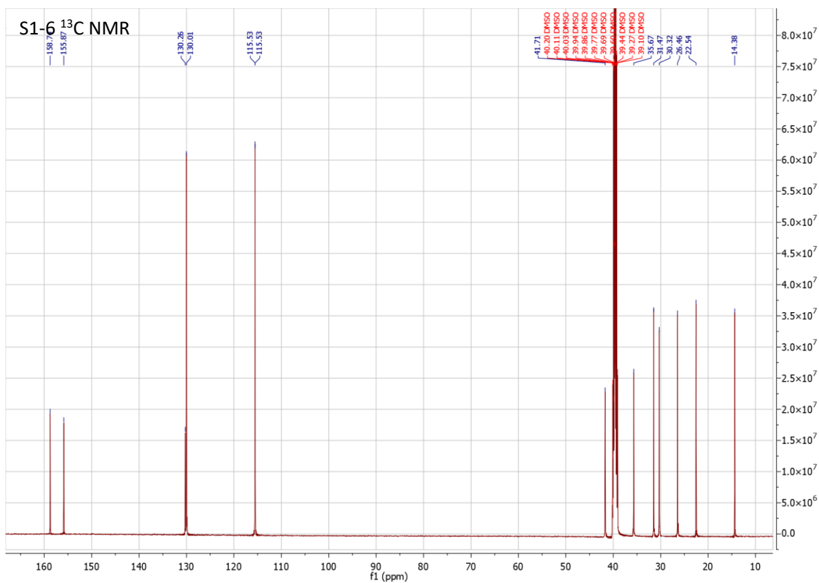
Figure S1. 1 H NMR (top) and 13 C NMR (bottom) spectra of S1-6
