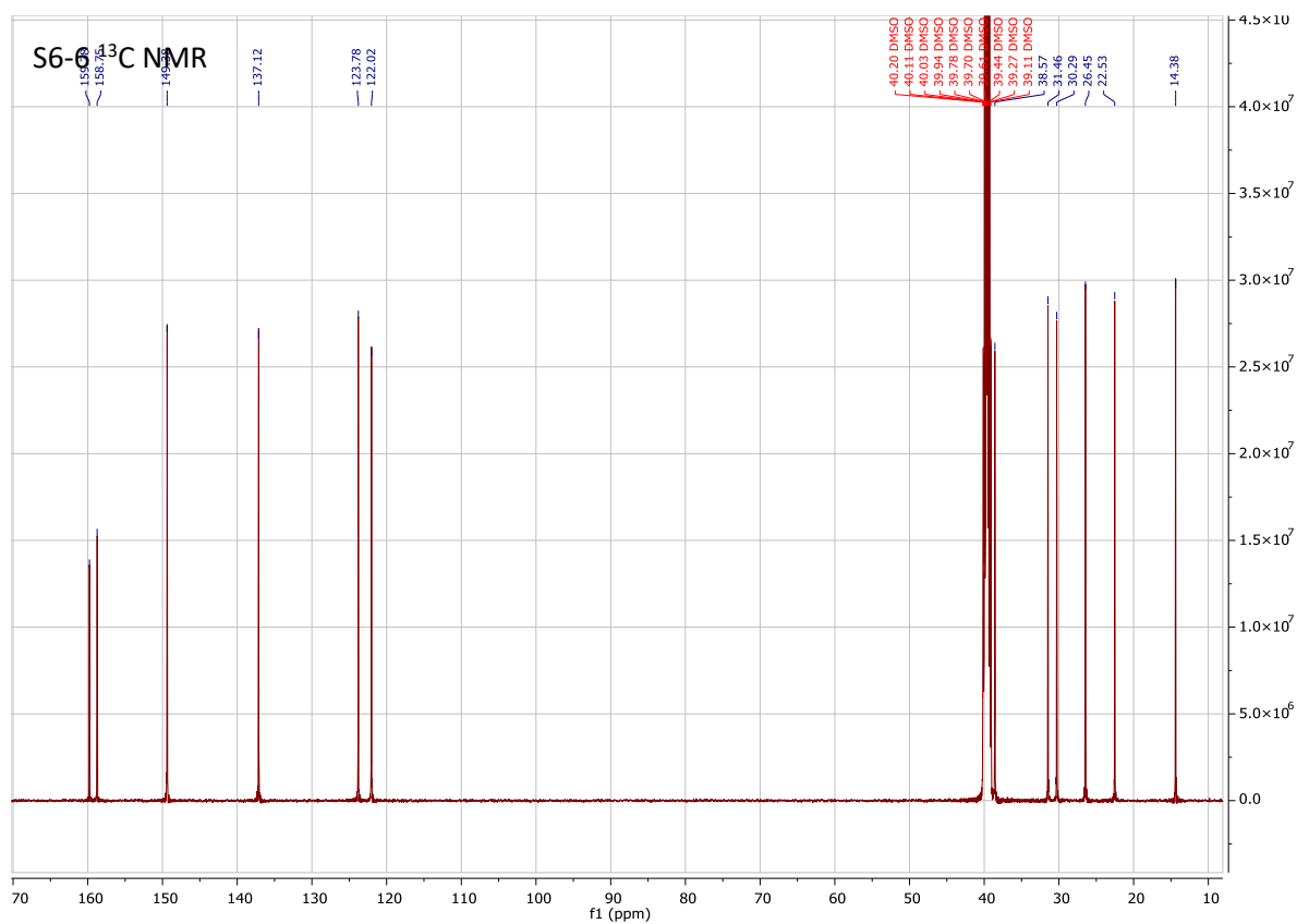
Figure S11. 1 H NMR (top) and 13 C NMR (bottom) spectra of S6-6
