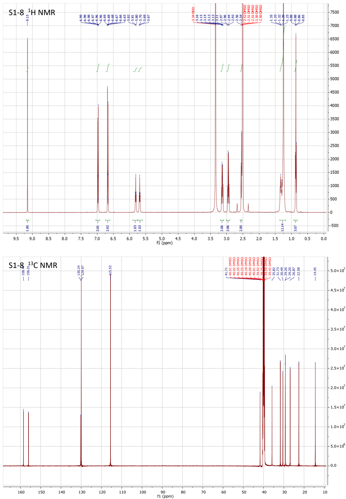
Figure S 1. 1 H NMR (top) and 13 C NMR (bottom) spectra of S1-8
