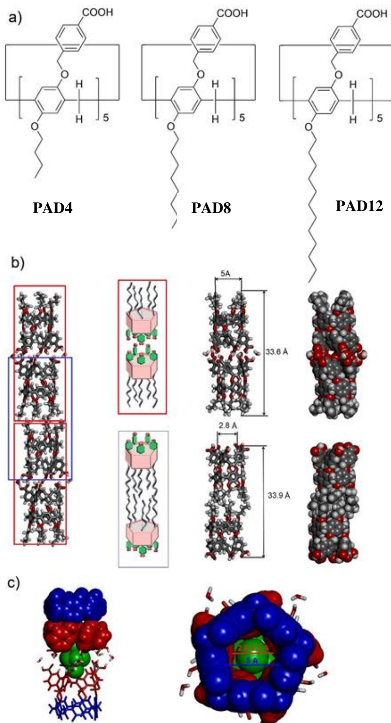
Figure 1. a) Structures of peralkylcarboxylate-pillar[5]arenes PAD4 , PAD8 and PAD12 and b) X-ray single crystal structure of PAD4. 29 Crystal packing along c-axis emphasizing self-assembled tubular carboxylate H-bonding (b, red) and bilayer hydrophobic (b, blue) dimers in stick and CPK representations. Crystalline solid state structures show dimeric structures of 34 Å length and c) a variable pore geometry composed of Pillar[5]arene platform (blue) of 5 Å diameter and of narrowest twisted carboxy-phenyl pore of 2.8 Å diameter (red). Green CHCl 3 molecules in CPK representation are perfectly positioning a Cl atom fitting the narrowest carboxy-phenyl pore, while the other atoms are disordered in the larger junction formed via hydrogen bonding of the carboxylate groups.
