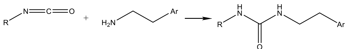
Scheme S1. General synthesis of alkylureido derivatives.
