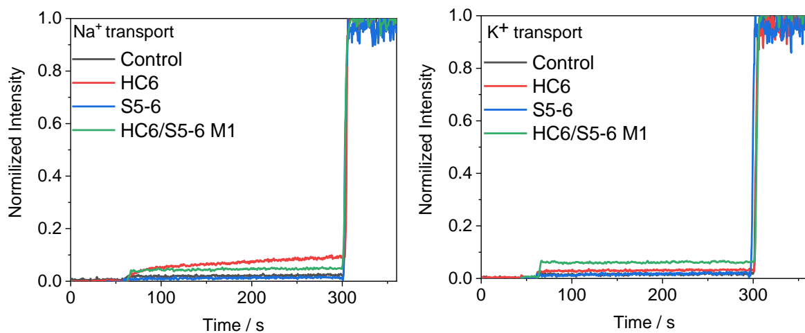
Figure S22. Comparison of cation transport activity expressed as normalized fluorescence intensity of 5 mM / 5 mM HC6/S5-6 system and individual compounds in the extra-vesicular medium containing 100 mM NaCl(left) or KCl (right).
