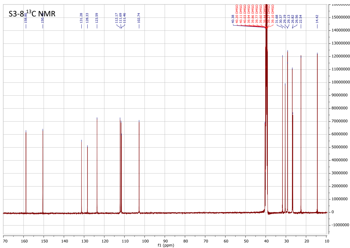
Figure S6. 1 H NMR (top) and 13 C NMR (bottom) spectra of S3-8
