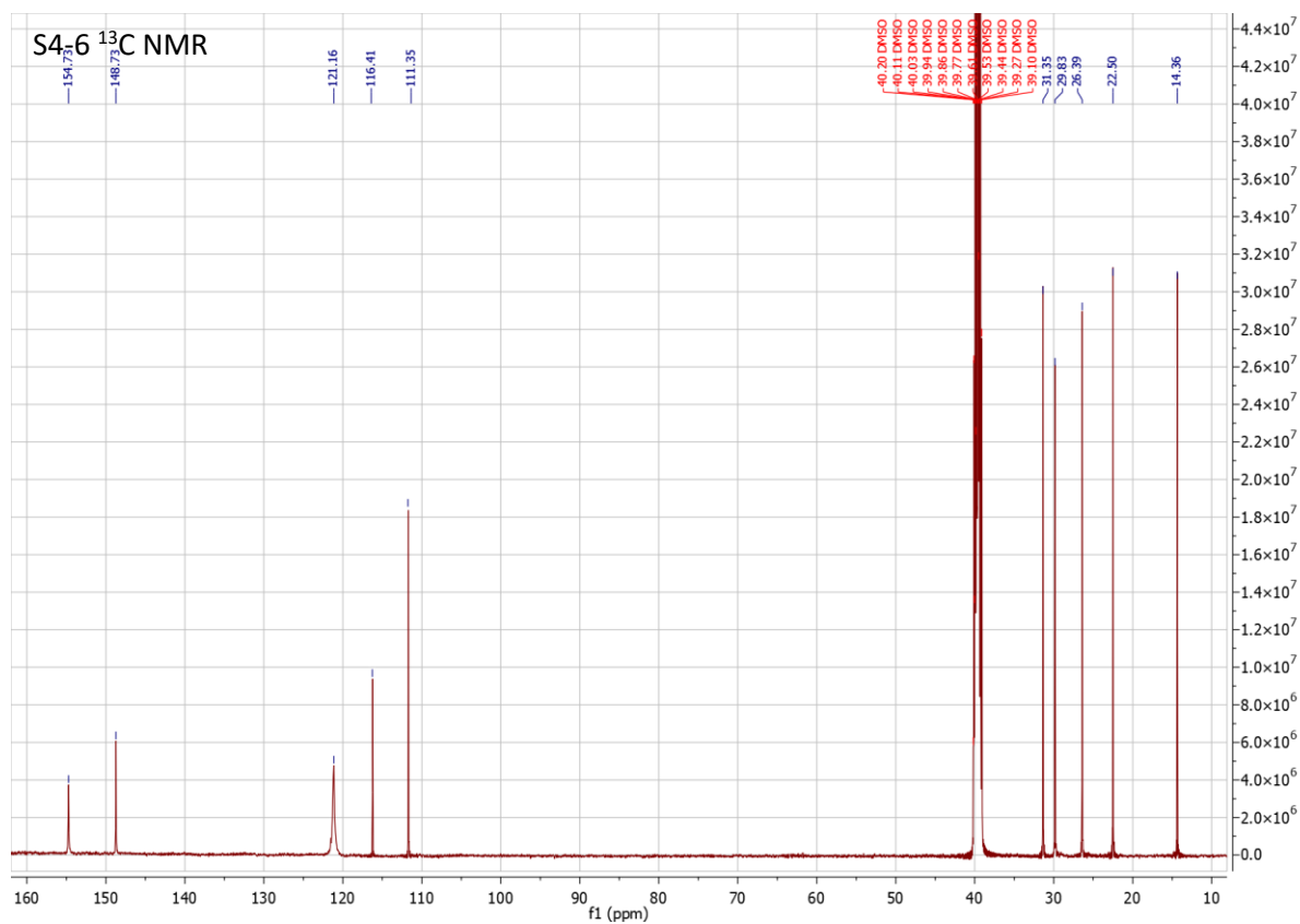
Figure S7. 1 H NMR (top) and 13 C NMR (bottom) spectra of S4-6
