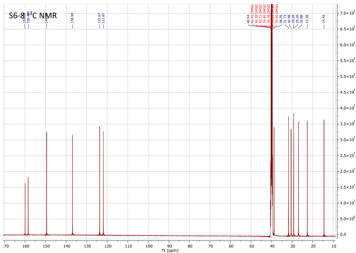
Figure S12. 1 H NMR (top) and 13 C NMR (bottom) spectra of S6-8
