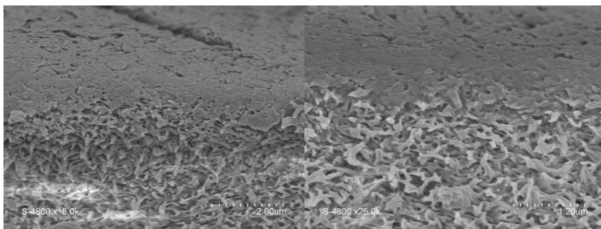
Figure S7. Cross-section SEM micrographs of PA-PA[5] membrane prepared using PA[5] 0.01% solution (membrane composition MPD 1.2 w/w % and TMC 0.1w/w %)
