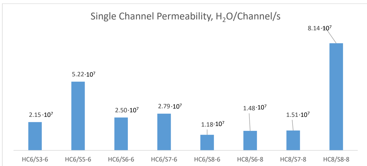
Figure S18. Comparison of single channel permeabilities of combined systems.
