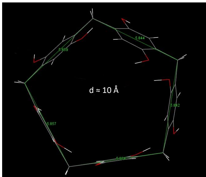
Figure S4. Crystal structure of Pillar[5]arene core. [S1] The cross-sectional surface of this molecule was calculated as 0.786 \text{ nm}^2 based on its diameter. The value of cross-sectional surface was used for calculation of single channel permeability of Pillar[5]arenes dimers since pillar[5]arene is the core of these channels.
