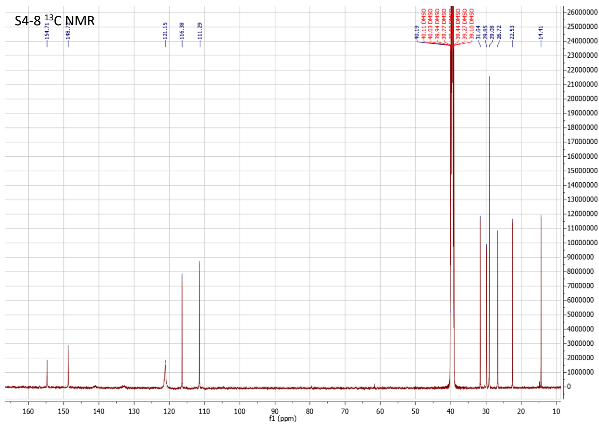
Figure S8. ^1\text{H} NMR (top) and ^{13}\text{C} NMR (bottom) spectra of S4-8
