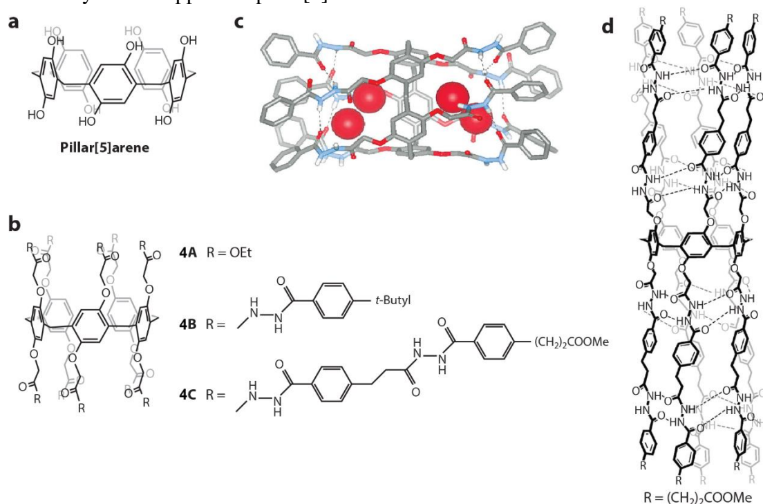
Figure 8. Hydrazide-appended pillar[5]arenes (PAH5). a) Crystal structure of pillar[5]arene. b) A series of PAH5. c) Chemical structure of 4B . d) Schematic tubular conformation of 4C . Image adapted from reference [61].
