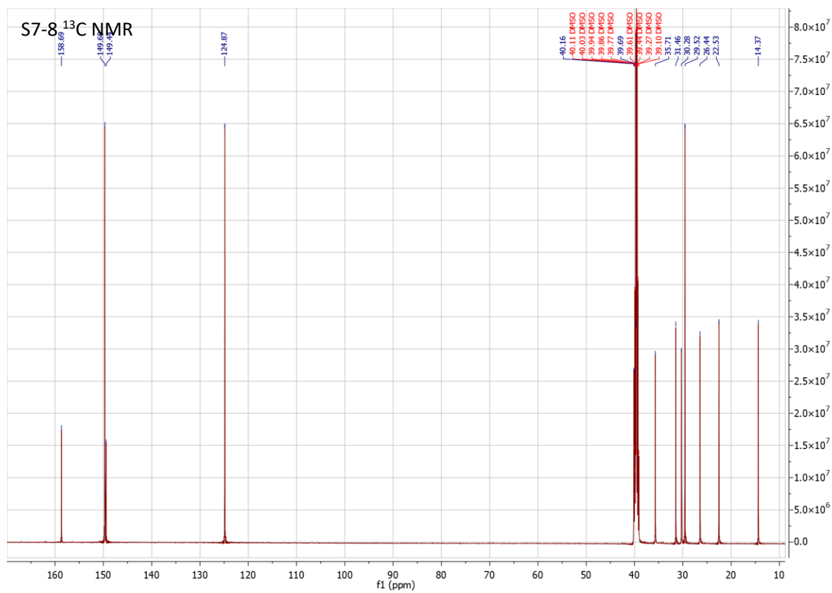
Figure S14. 1 H NMR (top) and 13 C NMR (bottom) spectra of S7-8
