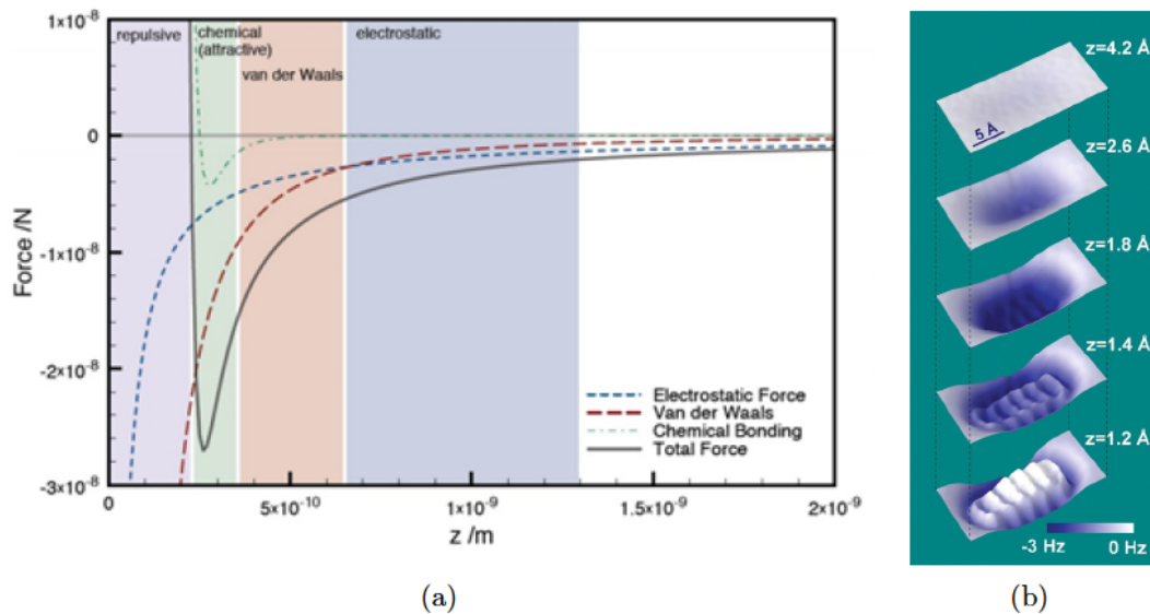
Figure 1.6: a) Different force contribution detected in AFM plotted in tip-sample distance, extracted from [49] b) Maps of frequency shift above the pentacene molecule for different tip-sample separation [9]
