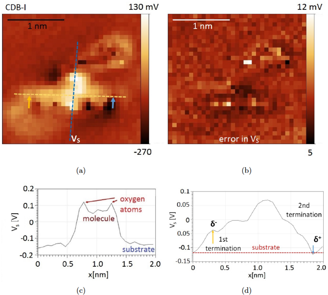
Figure 3.9: a) Surface potential map of CDB-I molecule presented in the Figure 3.8, b) uncertainty in surface potential. Two cross sections of V_s indicated with intermittent lines in the image a) and are presented in c) cross section of the central phenyl with oxygen atoms (blue colour) and d) cross section through three-phenyl core (yellow colour).
