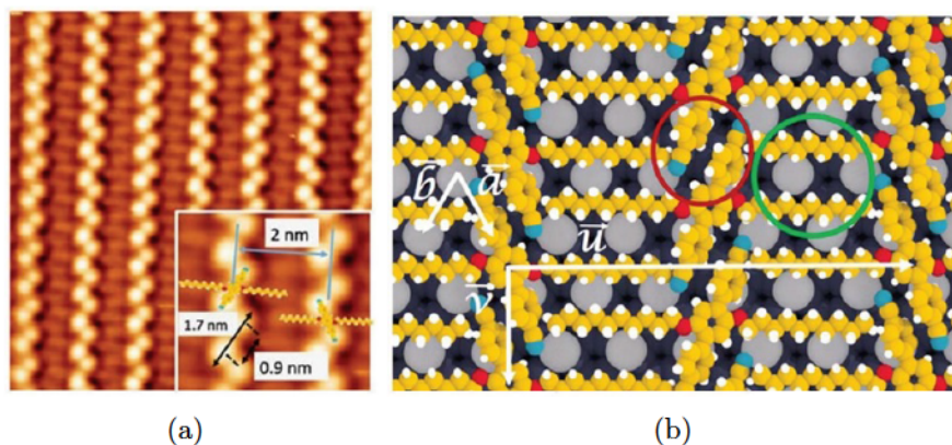
Figure 4.3: a) STM image of CDB network on Si:B surface ( V_{bias} = 1.7 V, I_t = 10 pA), in the inset molecules position with characteristic dimensions are indicated. b) Model of adsorption of molecule on Si:B surface, \pi - \pi stacking between molecules are indicated with red circle, chain interdigitation is indicated with green circle. Extracted from [78].
