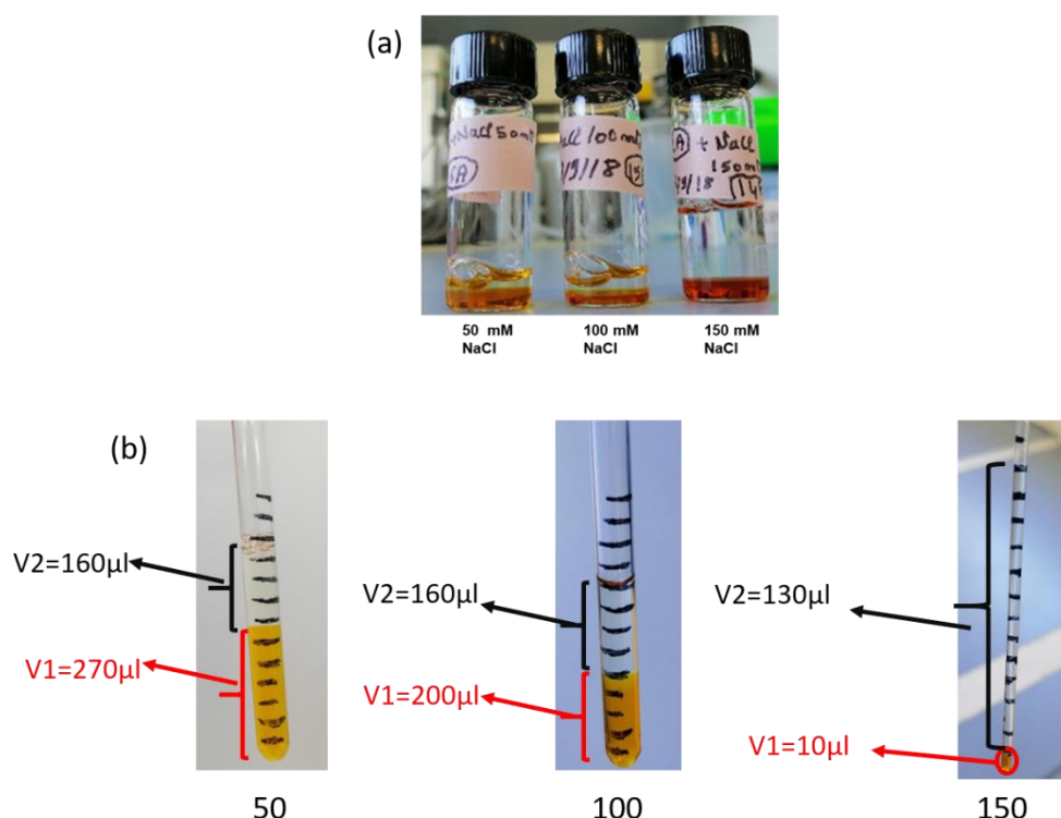
Figure 20. Three solutions of C8G1 150 mM in the presence of NaCOSAN 30 mM and [\text{NaCl}] = 50, 100 and 150 mM. The same solutions prepared in capillaries in order to determine the volume ratio between the lower and upper phases.
