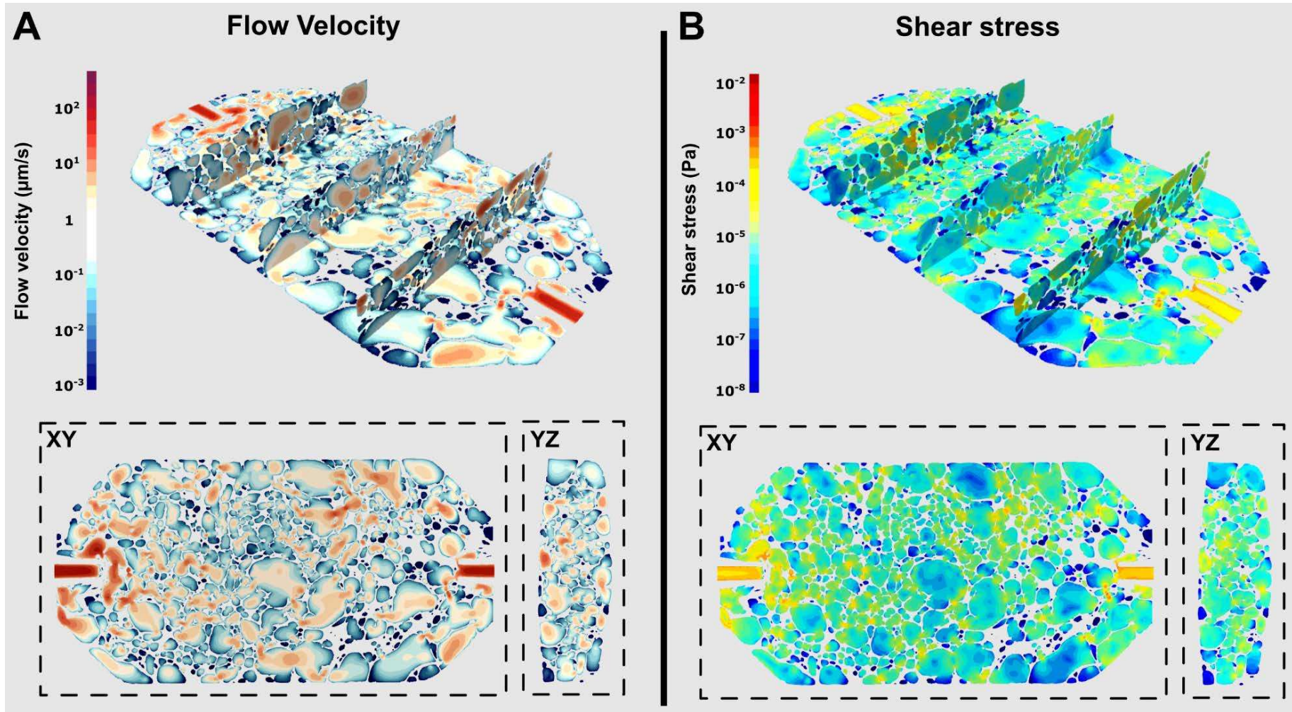
Figure 4.18. Solutions of the incompressible Navier-Stokes equations within the microfluidic device for a flow rate at 100 \mu\text{L}/\text{h} . (a) 3D crosscut colormap of the flow velocity within the device. Beneath a cross-sectional representation along the planes xy and yz . Colormap scale is logarithmic. (b) 3D colormap of the shear stress within the device. Beneath a cross-sectional representation along the planes xy and yz . Colormap is in logarithmic scale.
