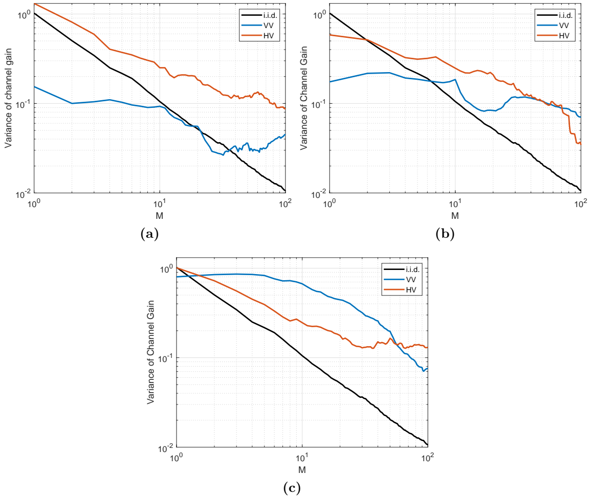
Figure 3.11: Channel hardening effect using \frac{\mathbb{V}\{\|\mathbf{h}_k\|^2\}}{(\mathbb{E}\{\|\mathbf{h}_k\|^2\})^2} for (a) LOS UE1, (b) OLOS UE 3 and (c) NLOS UE 11, as a function of M .
