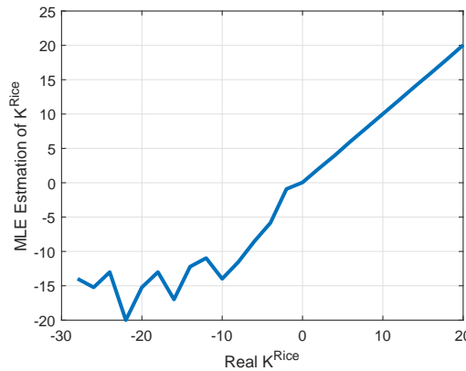
Figure C.1: Convergence of the MLE estimator for different K^{Rice} values.
