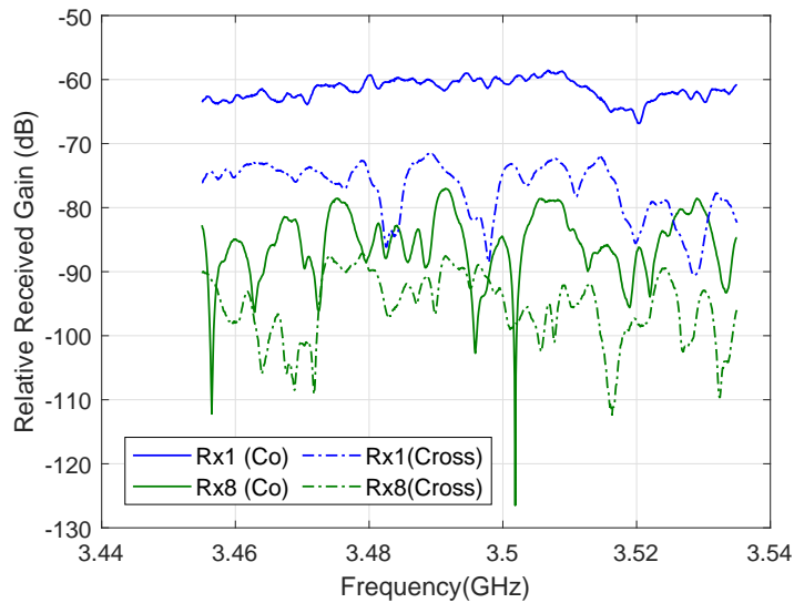
Figure 3.6: |\mathbf{h}_{1,50,\psi}(f)|^2 and |\mathbf{h}_{8,50,\psi}(f)|^2 for co- and cross-polarization links.
