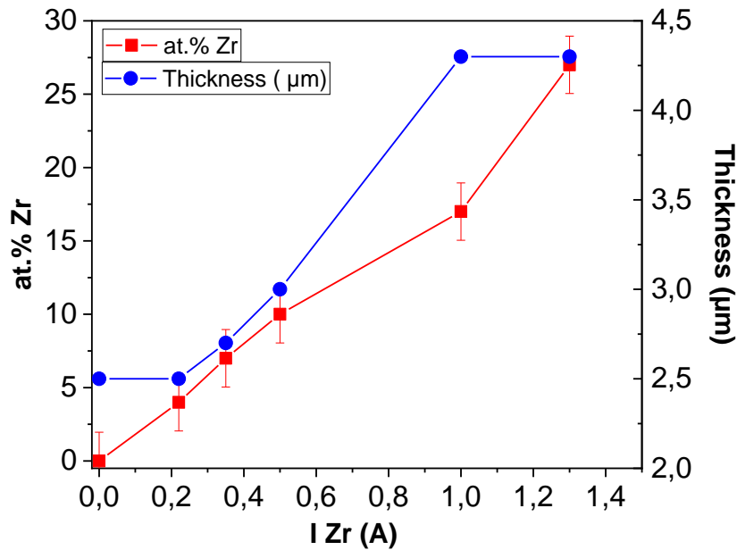
Figure II- 5. Evolution of thickness and Zr content in films as a function of the intensity of current applied to Zr target ( I_{Al} = 2 \text{ A} ).
