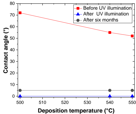
Figure IV- 12. Water contact angles as a function of TiO 2 deposition temperature for HSS/Al-Zr/TiO 2 bilayer films before UV illumination, after UV illumination and after six months without UV illumination.
