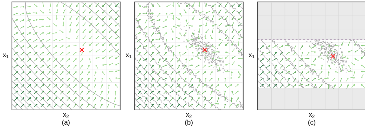
Figure 3.1: Contour plots and direction of greatest descent -\nabla f(\mathbf{x}) , for search spaces defined by variations of the Booth function. Panels (a), (b), and (c) correspond to Equations 2.3, 2.4, and 2.5 respectively. The global optimum is marked with a \times . To aid visualization, vector magnitude was encoded by color intensity, so that darker vectors have larger magnitude. The gradient along the function's basin is near zero.
