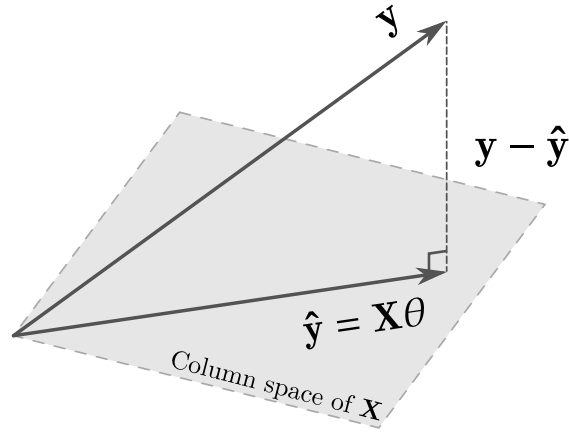
Figure 4.1: In Linear Regression, the prediction vector \hat{\mathbf{y}} is the projection of the observations vector \mathbf{y} into the vector space spanned by the columns of \mathbf{X} . The vector \boldsymbol{\varepsilon} = \mathbf{y} - \hat{\mathbf{y}} is the model error, and is minimized when we ensure it is orthogonal to \mathbf{X}\boldsymbol{\theta}
