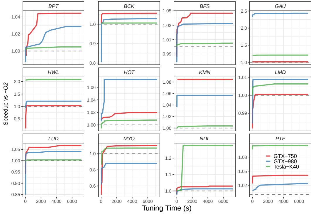
Figure 9.5: Mean speedup over 30 repetitions of the tuned solutions for Rodinia kernels versus the opt-level = 2 baseline, across two hours of tuning. Notice the difference in the y -axis scales for each panel
