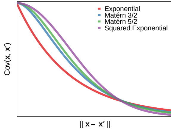
Figure 4.5: Covariance of points (\mathbf{x}, \mathbf{x}') according to four covariance functions based on the distance \|\mathbf{x} - \mathbf{x}'\| . Expressions for each kernel are shown in Table 4.1, and Matérn kernels use parameters v_1, v_2 = \{\frac{3}{2}, \frac{5}{2}\}
