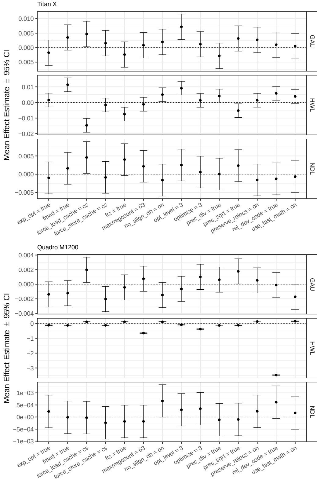
Figure 9.7: Main effects estimates and 95% confidence intervals for the high level of the 15 factors in the Plackett-Burman design, for target kernels measured on the Titan X and Quadro M1200 GPUs
