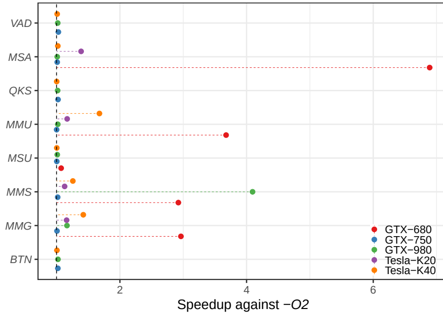
Figure 9.4: Mean speedup over 30 repetitions of the tuned solutions for kernels we implemented versus the opt-level = 2 baseline
