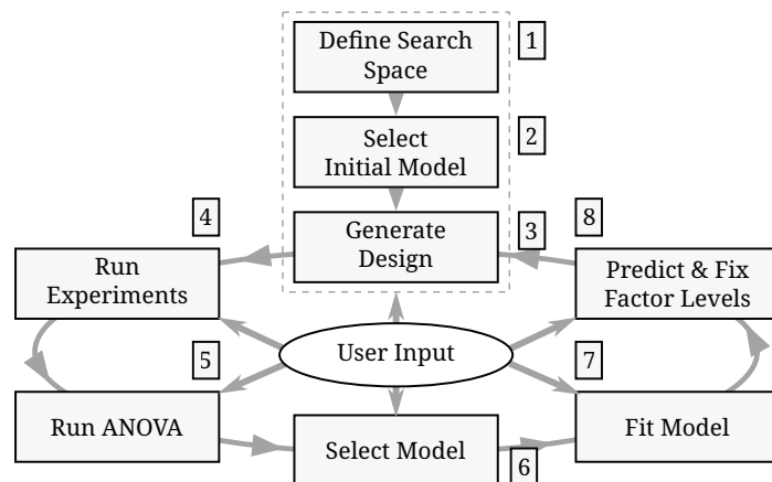
Figure 11.5: Overview of the DoE approach to autotuning we implemented
