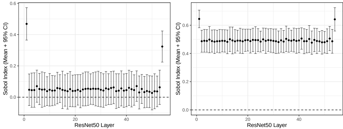
Figure 13.11: Sobol indices computed for the impact on Top5 accuracy of the quantization of each ResNet50 layer using only Sobol samples, in the left panel, and Sobol samples plus the search spaces explored by GPR, in the right panel
