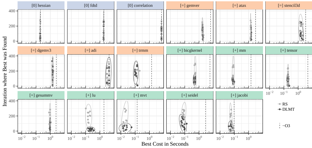
Figure 12.1: Cost of best points found on each run, and the iteration where they were found. RS and DLMT found no speedups with similar budgets for kernels marked with “[0]” and blue headers, and similar speedups with similar budgets for kernels marked with “[=]” and orange headers. DLMT found similar speedups using smaller budgets for kernels marked with “[+]” green headers. Ellipses delimit an estimate of where 95% of the underlying distribution lies
