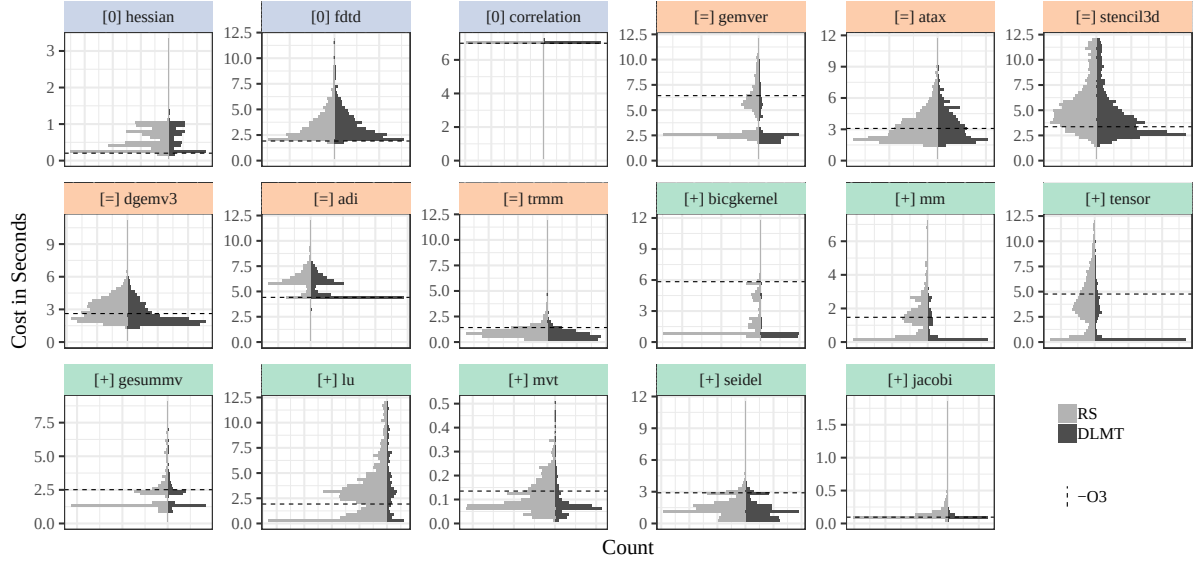
Figure 12.2: Histograms of explored search spaces, showing the real count of measured configurations. Kernels are grouped in the same way as in Figure 12.1. DLMT spent fewer measurements than RS in configurations with smaller speedups or with slowdowns, even for kernels in the orange group. DLMT also spent more time exploring configurations with larger speedups
