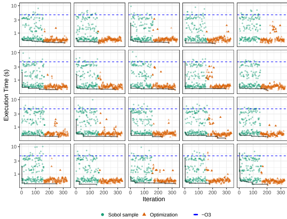
Figure 12.10: Execution time of points measured by GPR along iterations, with pareto border in red
