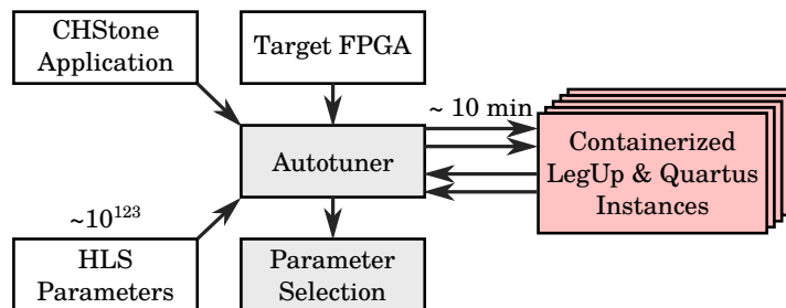
Figure 10.4: Autotuner Setup
