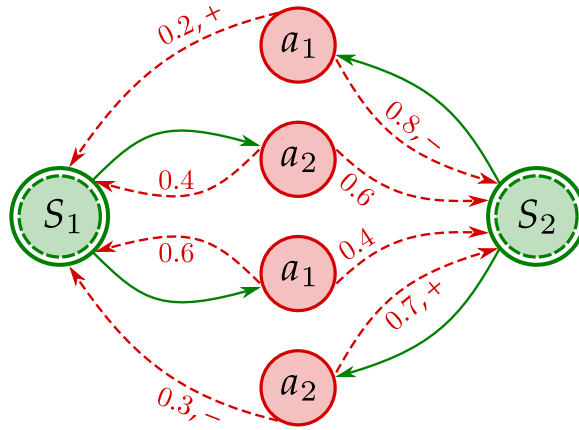
Figure 6.1: A Markov Decision Process with state set S = \{S_1, S_2\} , and action set A = \{a_1, a_2\} . The transition probabilities of each action are shown near the corresponding dashed red arrows. Rewards are either + , - , or zero, in which case no value is shown. The objective is to maximize the cumulative reward over a time period by finding a policy to choose which action, represented by the green arrows, should be taken in each state
