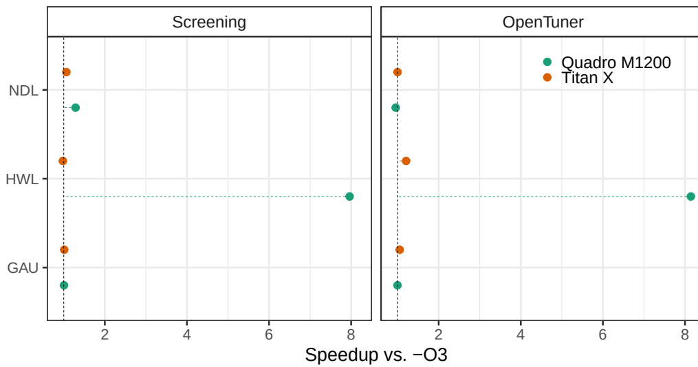
Figure 9.9: Mean speedups found using the predictions of the screening model and OpenTuner, for three Rodinia kernels on the Titan X and Quadro M1200 GPUs. The vertical dashed lines mark the PTX-stage opt-level=3 comparison baseline
