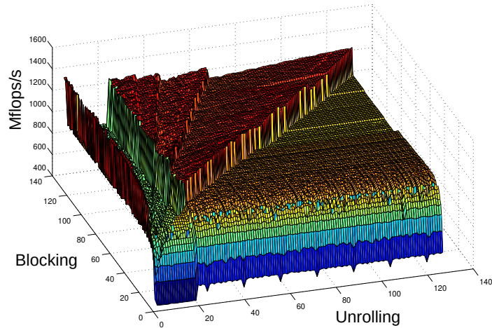
Figure 1.7: An exhaustively measured search space, defined by loop blocking and unrolling parameters, for a sequential GEMM kernel. Reproduced from Seymour et al. [164]
