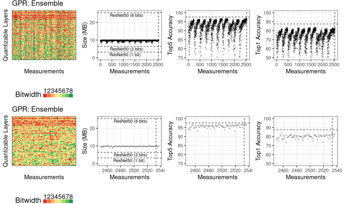
Figure 13.12: Running GPR with the gathered ensemble of GPR experiments. The bottom row shows only the new measurements performed after fitting a Gaussian Process with the ensemble of experiments, and the top row shows all the data that were used
