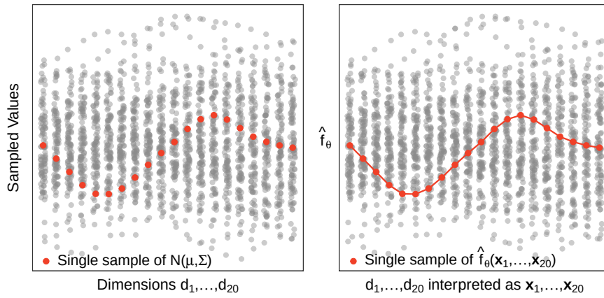
Figure 4.4: Reinterpreting the unrolled dimensions of 100 samples of a 20 dimension multi-variate normal, on the left panel, to obtain 100 samples of functions evaluated on 20 different input points, on the right panel
