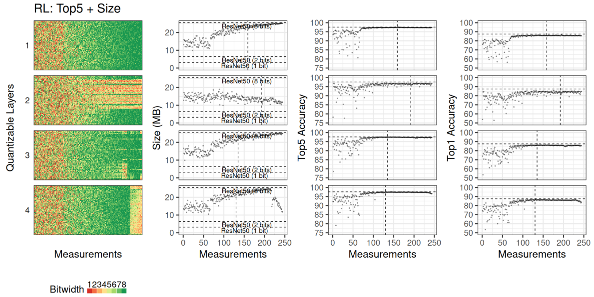
Figure 13.13: Optimizing accuracy and weight with the modified baseline Reinforcement Learning method
