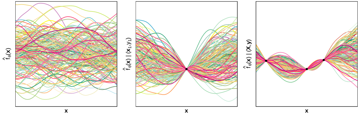
Figure 4.6: Fitting a Gaussian Process to three noise-free observations. The left panel shows 300 samples from a Gaussian prior, using the Matérn kernel to compute the covariance matrix. The center and right panels show 300 samples from the posterior distributions conditioned by one, then two more, successive noise-free observations
