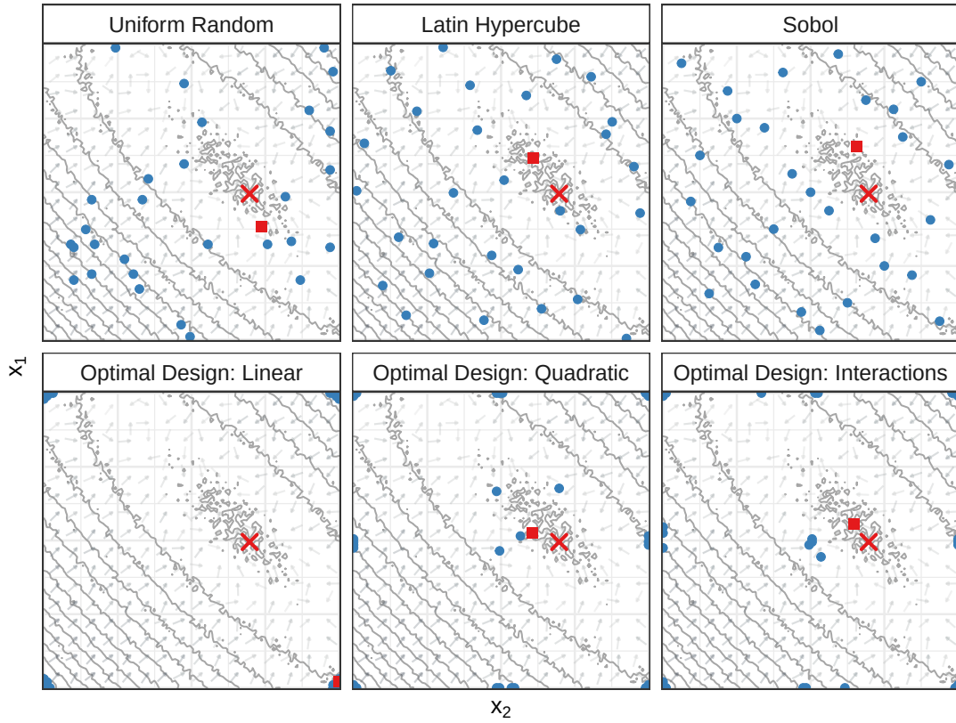
Figure 5.5: Exploring the search space for Booth's function with different methods, using a fixed budget of 30 measurements. A \times marks the global optimum, a \blacksquare marks the best point found by each strategy, and \bullet s mark measurements
