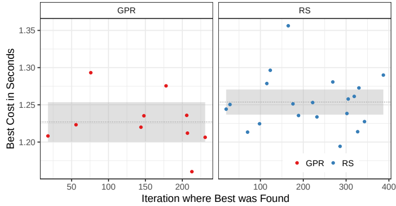
Figure 12.12: Best dgemv3 configurations and iterations that found them, for Gaussian Process Regression with Expected Improvement acquisition function (GPR), and uniform Random Sampling (RS), with a budget of 400 measurements.
