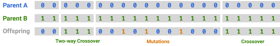
Figure 3.6: Some ways of producing offspring from two parents with binary chromosomes. Crossover splits parent chromosomes and combine the resulting pieces. In general, pieces from multiple splits can be combined. Mutations are introduced randomly and correspond to flipping bits on binary chromosomes.
