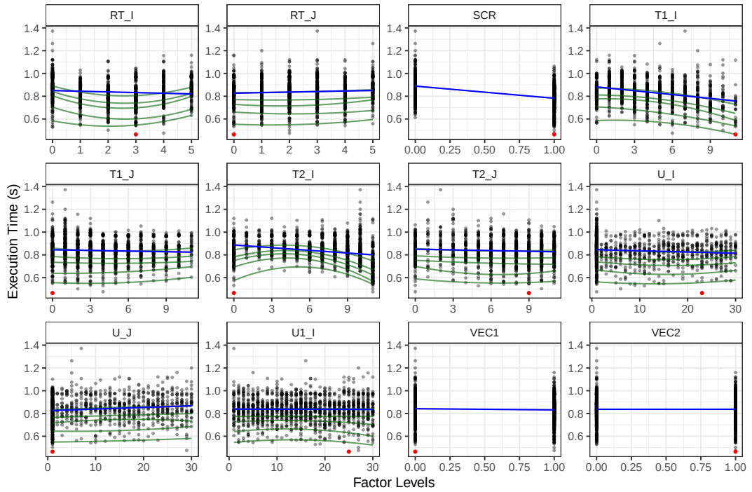
Figure 12.7: Same as above, for 10 uniform sampling runs with OMP fixed to on
