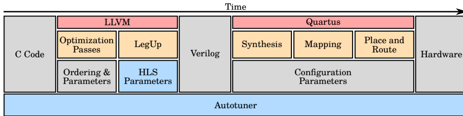
Figure 10.3: High-Level Synthesis compilation process. The autotuner search space at the HLS stage is highlighted in blue
