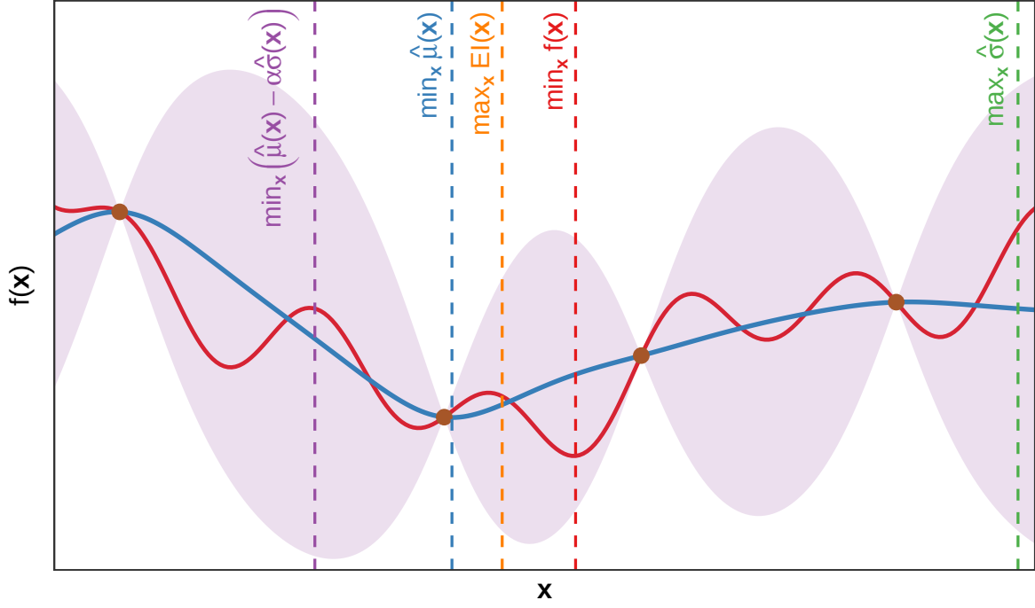
Figure 6.2: A surrogate Gaussian Process, whose mean is shown in blue , fit to four observations, shown in brown , of an objective function represented by the red line. The dashed vertical lines show which x would be chosen for the next observation if we followed the surrogate's minimum mean , its minimum mean minus its confidence interval lower bound, its maximum variance , or if we picked the x that maximizes its Expected Improvement
