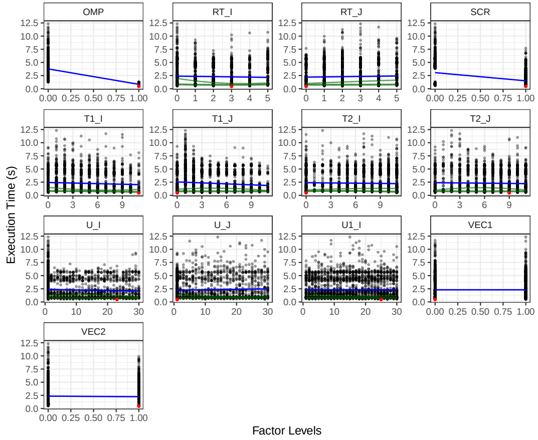
Figure 12.6: Fitting linear models and quadratic quantile regression, with \tau = 0.05, 0.25 , and 0.5 , to separate factors for 10 uniform random sampling runs
