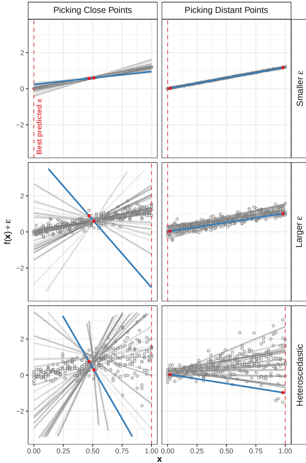
Figure 5.1: Fitting linear models using 30 distinct random sets of two measurements, in experimental settings with different properties of the error \varepsilon . One arbitrary model fit is highlighted to show the distance between the design points
