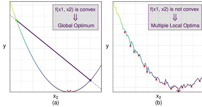
Figure 2.2: Illustrating the relationship between convexity of a function over a compact set and the presence of local minima. Panels (a) and (b) match the functions on the same panels of Figure 2.1
