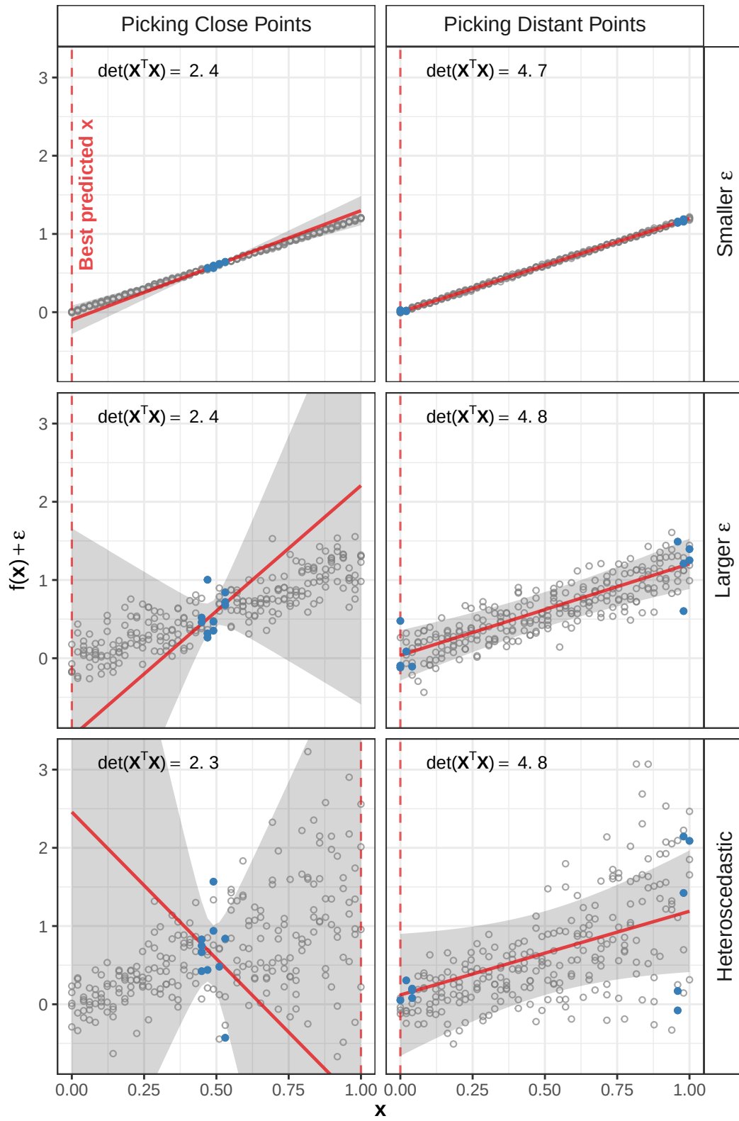
Figure 5.2: Modeling linear effects in different experimental settings
