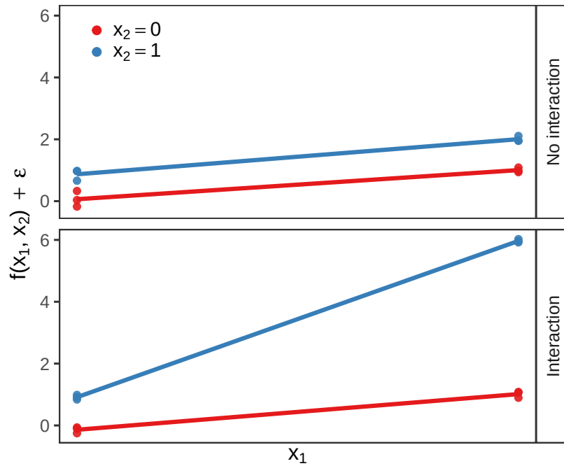
Figure 5.3: Effect of interactions in the slopes for extreme values of factors
