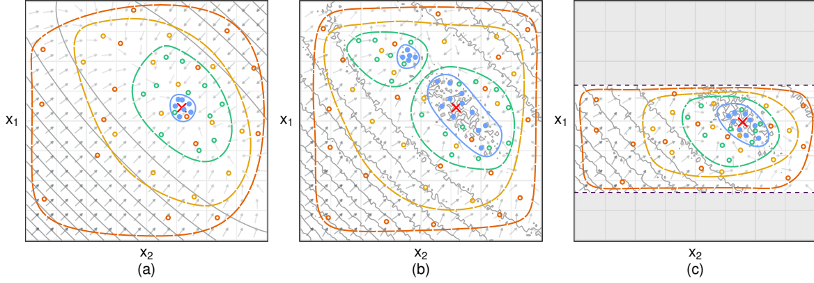
Figure 3.7: Color-coded generation snapshots of a Genetic Algorithm on the search spaces defined by variations of the Booth function. Hollow points and dashed lines mark members of previous populations and the regions they covered, while filled points and complete lines mark the final population. Panels (a), (b), and (c) correspond to Equations 2.3, 2.4, and 2.5 respectively. Contour plots and direction of greatest descent are also shown, and the global optimum is marked with a \times .
