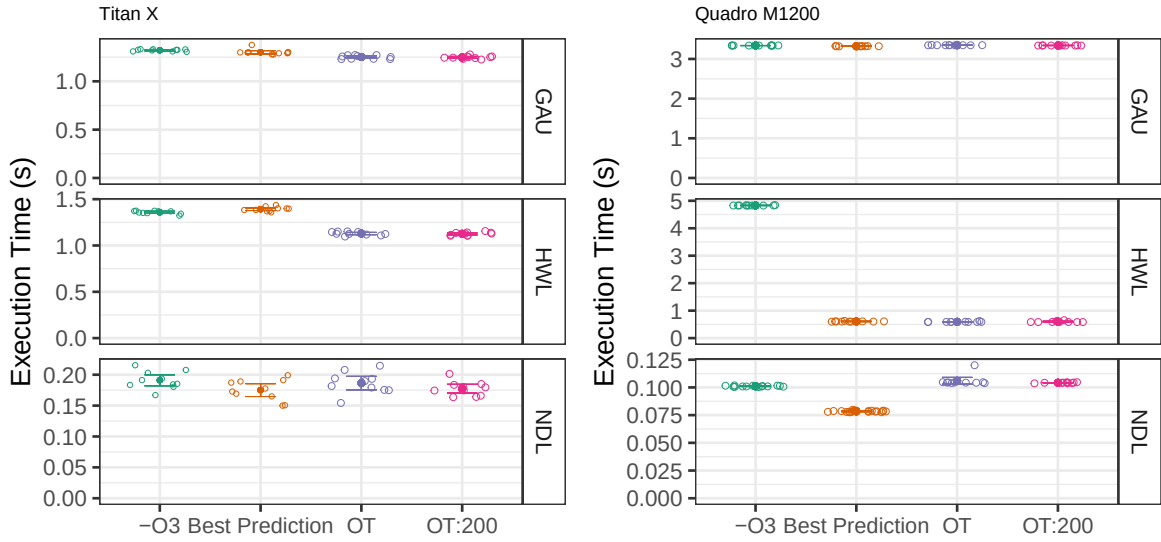
Figure 9.8: Execution time of baseline and model-predicted NVCC flag configurations for three Rodinia kernels on the Titan X and Quadro M1200 GPUs. Circles mark each of the 20 measurements of each flag configuration, filled dots and whiskers mark the mean and 95% confidence intervals. The experiments marked OT were made with OpenTuner using the same number of measurements used in screening, and experiments marked OT:200 used 200 measurements
