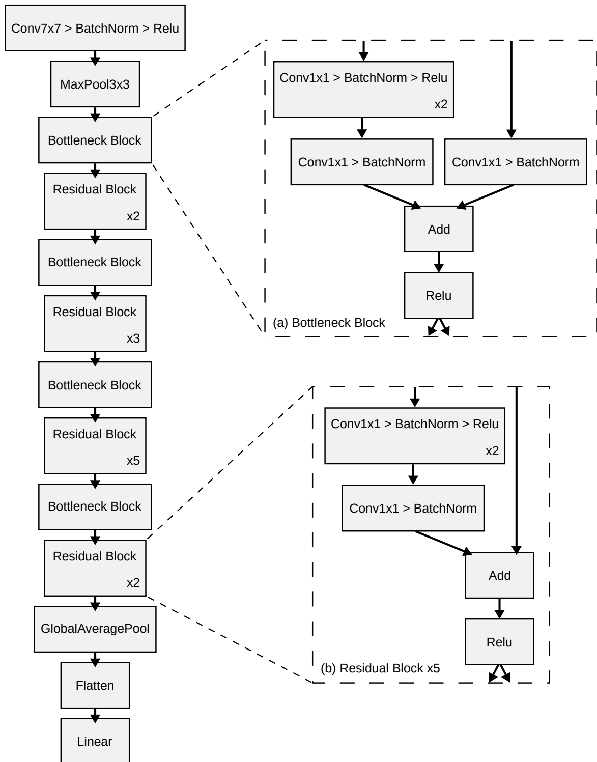
Figure 13.2: ResNet50 architecture, implemented in pytorch
