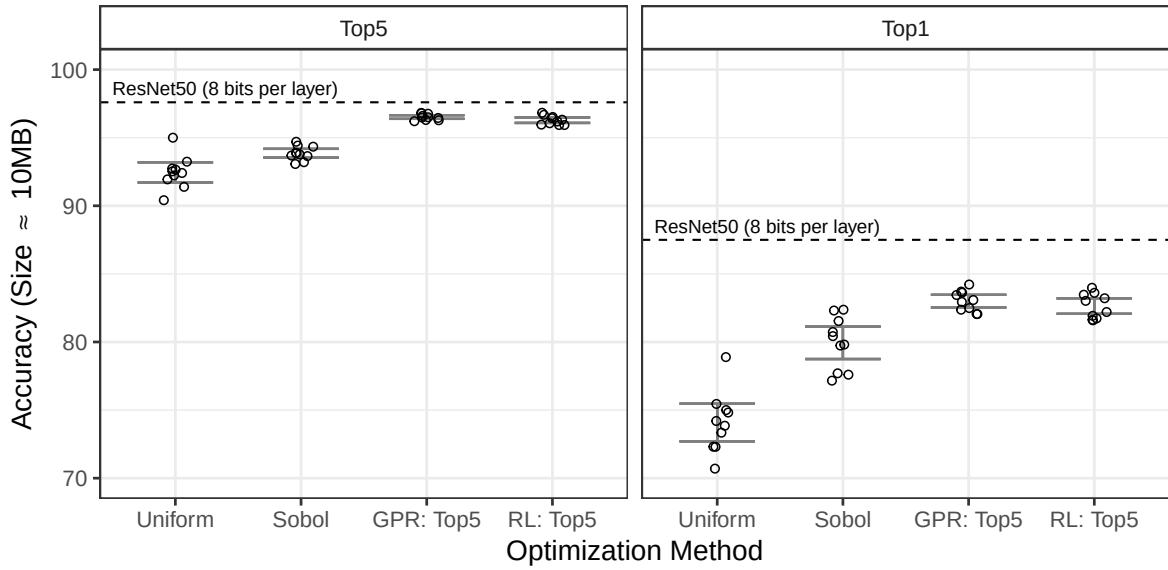
Figure 13.5: 10 repetitions of the 4 methods we compared, using a budget of 245 measurements, with 95% confidence intervals for estimates of the mean
