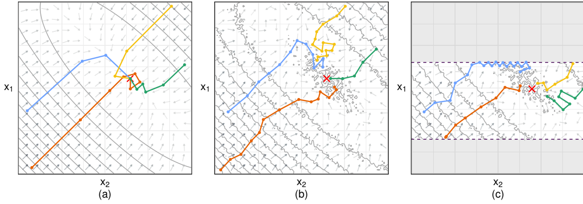
Figure 3.3: Representation of paths taken by the gradient descent method with 4 restarts, with adaptive choice of \alpha_k , on the search spaces defined by variations of the Booth function. Panels (a), (b), and (c) correspond to Equations 2.3, 2.4, and 2.5 respectively. Contour plots and direction of greatest descent -\nabla f(\mathbf{x}) are also shown, and the global optimum is marked with a \times .
