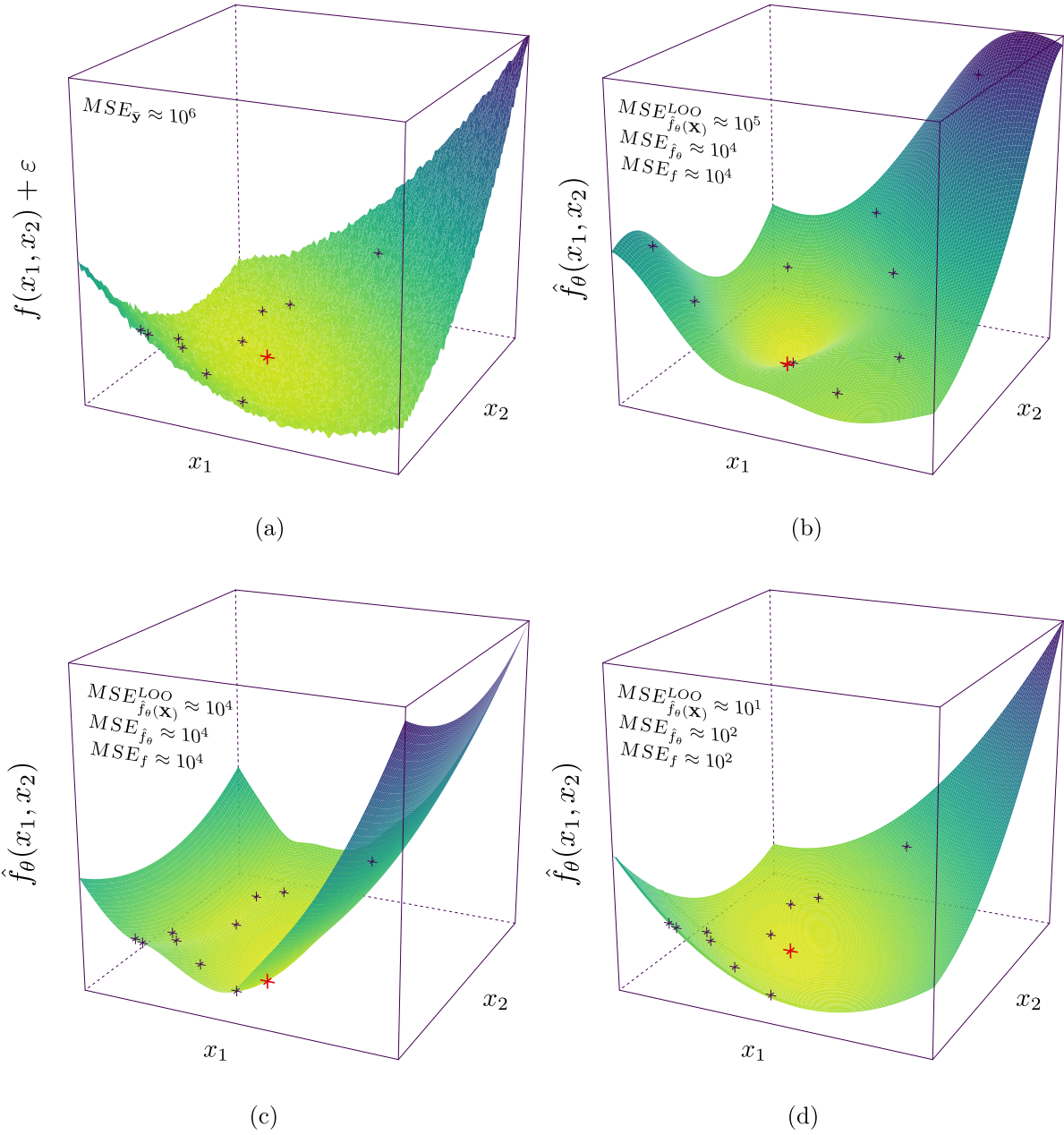
Figure 4.9: Three Gaussian Process Regression surrogates with noisy fits for the Booth function, with a \times marking the global optimum and best surrogate predictions. The fixed experimental design \mathbf{X} used to fit all surrogates is marked by \times s. Panel (a) shows noisy measurements of Booth's function, panels (b), (c), and (d) show surrogate predictions for models fit with linear, quadratic, and quadratic plus interactions trends, respectively
