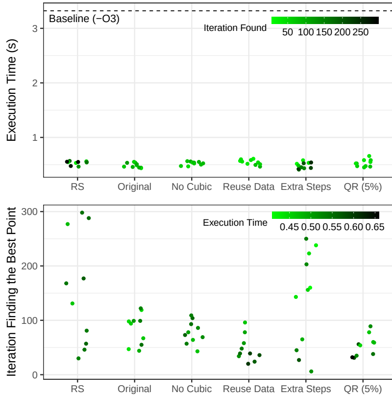
Figure 12.3: Summary of our DLMT results, compared to uniform Random Sampling (RS), showing the configurations with smallest speedups, found in 10 independent runs. The top panel compares execution time, with color-encoded iterations, and the bottom panel compares iterations where configurations were found, with color-encoded execution times.
