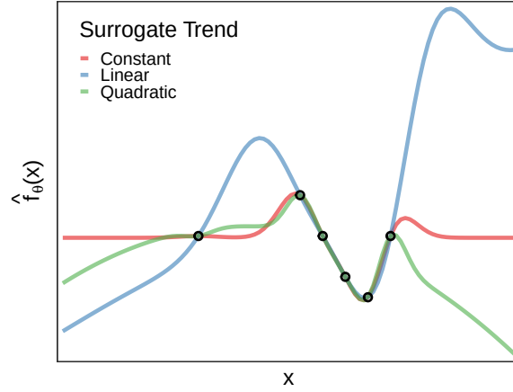
Figure 4.8: Gaussian Process surrogates using three different model trends, fit to six noise-free observations of a single-input objective function, marked with black circles
