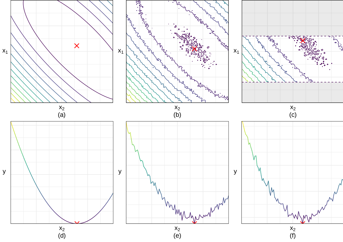
Figure 2.1: Contour plots and slices through the global optimum, marked with a \times , for search spaces defined by variations of the Booth function. Panels (a) and (d) correspond to Equation 2.3, panels (b) and (e) to Equation 2.4, and panels (c) and (f) to Equation 2.5.
