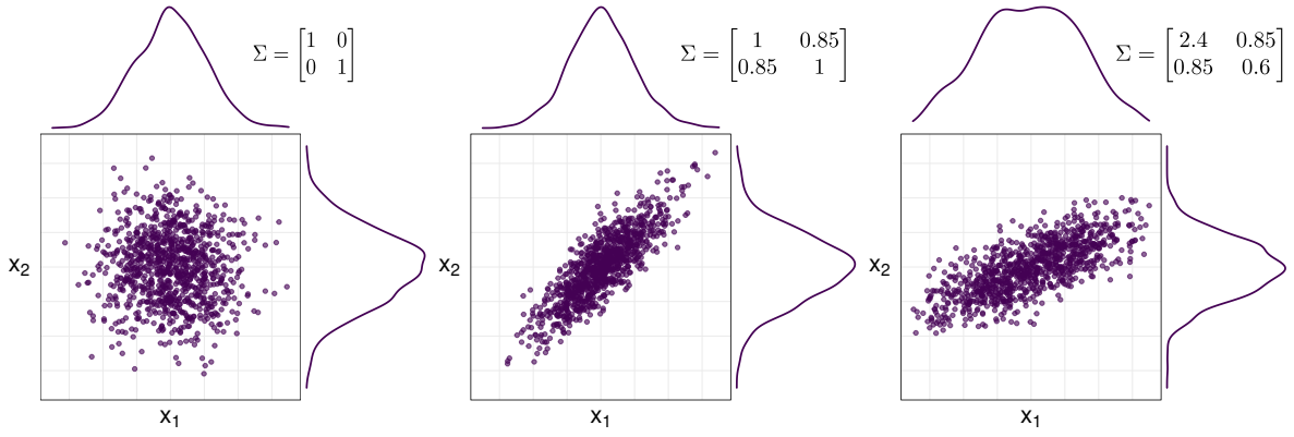
Figure 4.3: Effects of three covariance matrices on a multivariate normal distribution with mean vector \mu = [0 \ 0]^T and covariance matrix \Sigma as shown on the upper right corner of each plot
