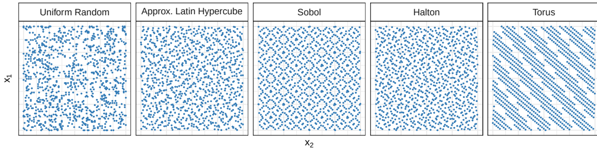
Figure 5.4: Comparison of 1000 samples obtained with different sampling methods. The Latin Hypercube design was produced with the DiceDesign R package [77], and was optimized after an initial sampling, with Simulated Annealing. Sobol, Halton, and Torus are low-discrepancy sequences from the randtoolbox R package [63].
