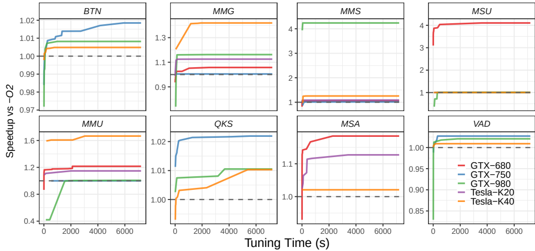
Figure 9.6: Mean speedup over 30 repetitions of the tuned solutions for the kernels we implemented versus the opt-level = 2 baseline, across two hours of tuning. Notice the difference in the y -axis scales for each panel
