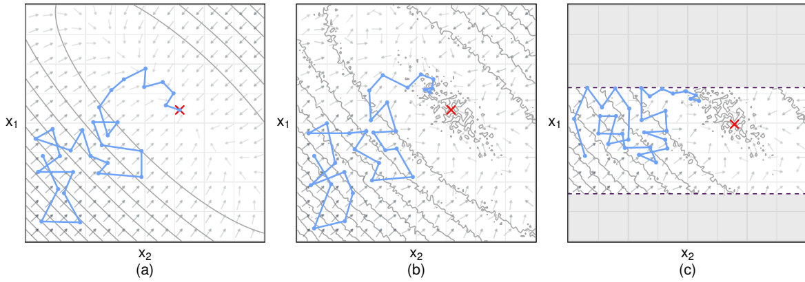
Figure 3.5: Representation of paths taken by the Simulated Annealing method on the search spaces defined by variations of the Booth function. Panels (a), (b), and (c) correspond to Equations 2.3, 2.4, and 2.5 respectively. Contour plots and direction of greatest descent are also shown, and the global optimum is marked with a \times .
