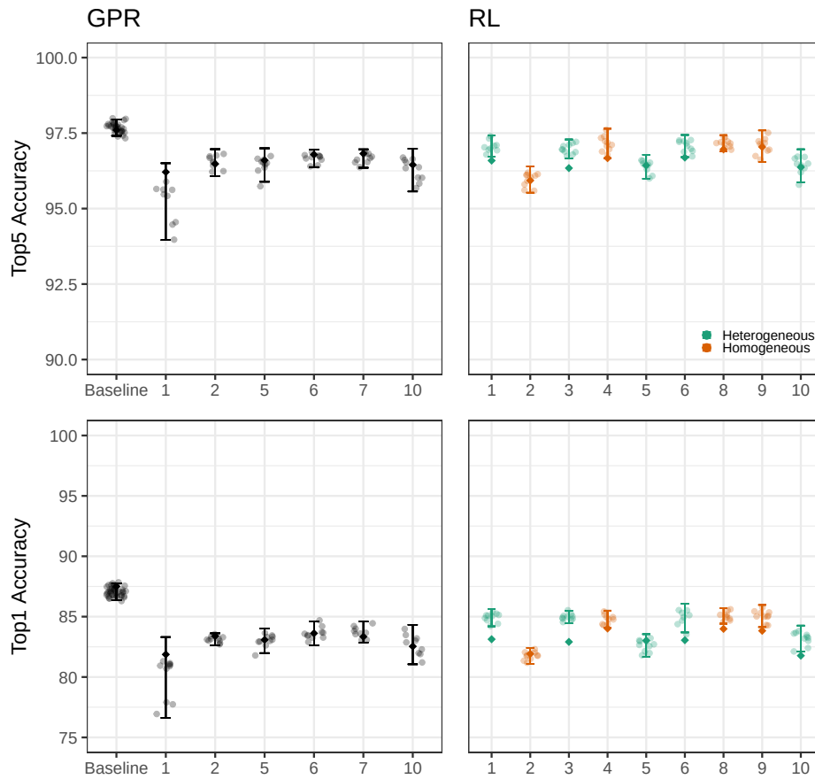
Figure 13.9: Running optimized quantization policies with new ImageNet samples, with 95% confidence intervals for the mean estimate. Diamond shapes mark the measured accuracy on the original sample. The baseline is the uniform 8-bit ResNet50 quantization
