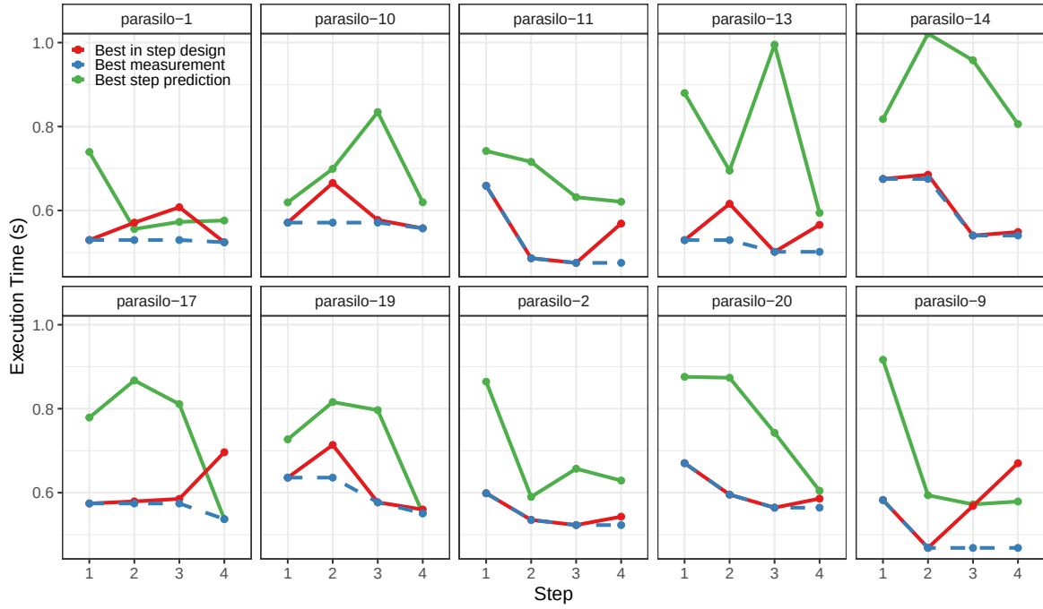
Figure 12.8: Performance of best points, step-by-step, by experiment
