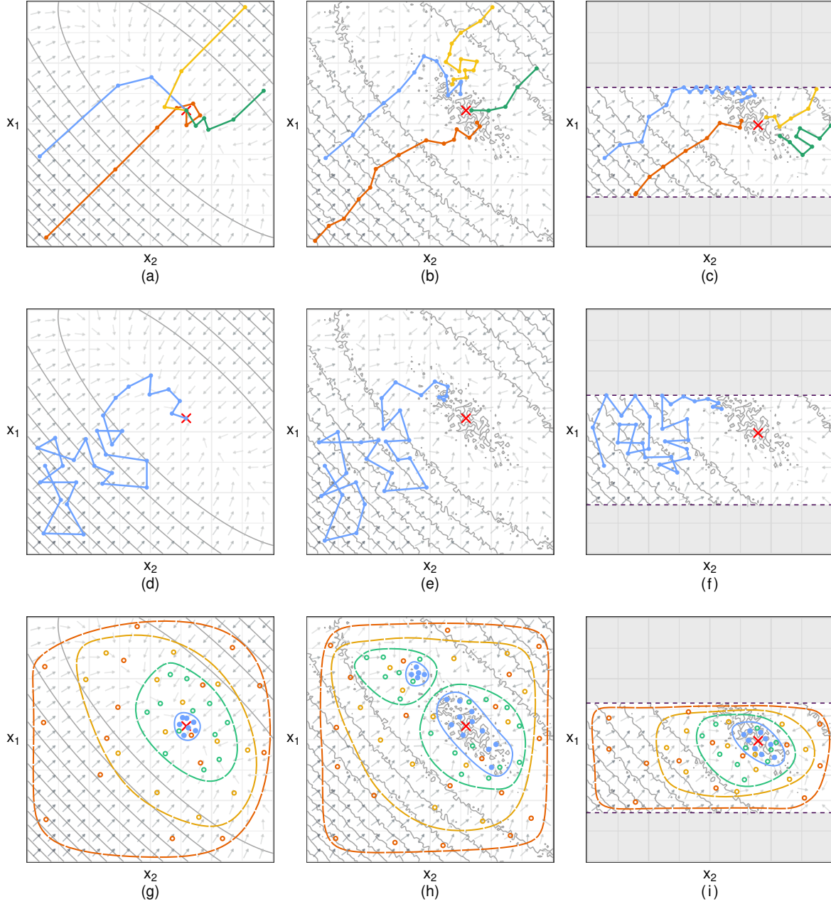
Figure 3.8: Representation of paths taken by the gradient descent method, with adaptive choice of \alpha_k , on the search spaces defined by variations of the Booth function. Panel groups (a,d,g), (b,e,h), and (c,f,i) correspond to Equations 2.3, 2.4, and 2.5 respectively. Panel groups (a,b,c), (d,e,f), and (g,h,i) correspond to Gradient Descent with restarts, Simulated Annealing, and a Genetic Algorithm, respectively. Contour plots and direction of greatest descent -\nabla f(\mathbf{x}) are also shown, and the global optimum is marked with a \times .
