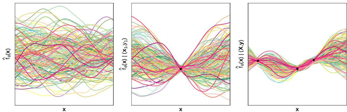
Figure 4.7: Fitting a Gaussian Process to three noisy observations, in the same conditions and with the same panel structure in Figure 4.6
