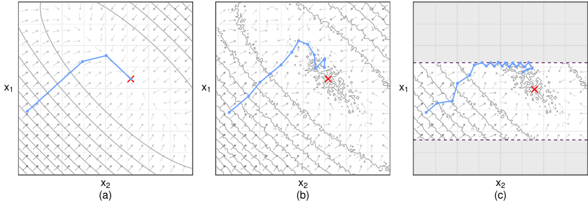
Figure 3.2: Representation of paths taken by the gradient descent method, with adaptive choice of \alpha_k , on the search spaces defined by variations of the Booth function. Panels (a), (b), and (c) correspond to Equations 2.3, 2.4, and 2.5 respectively. Contour plots and direction of greatest descent -\nabla f(\mathbf{x}) are also shown, and the global optimum is marked with a \times .
