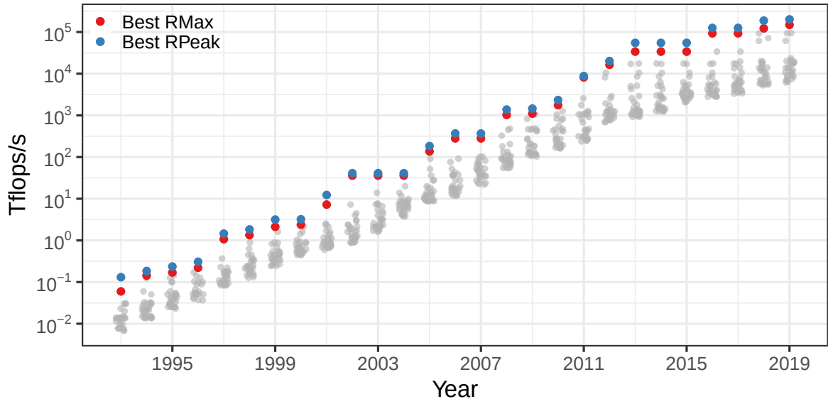
Figure 1.2: Sustained exponential increase of theoretical RPeak and achieved RMax performance, highlighted for the supercomputer ranked 1 st on TOP500 [175], and shown in gray for the other 30 ranks
