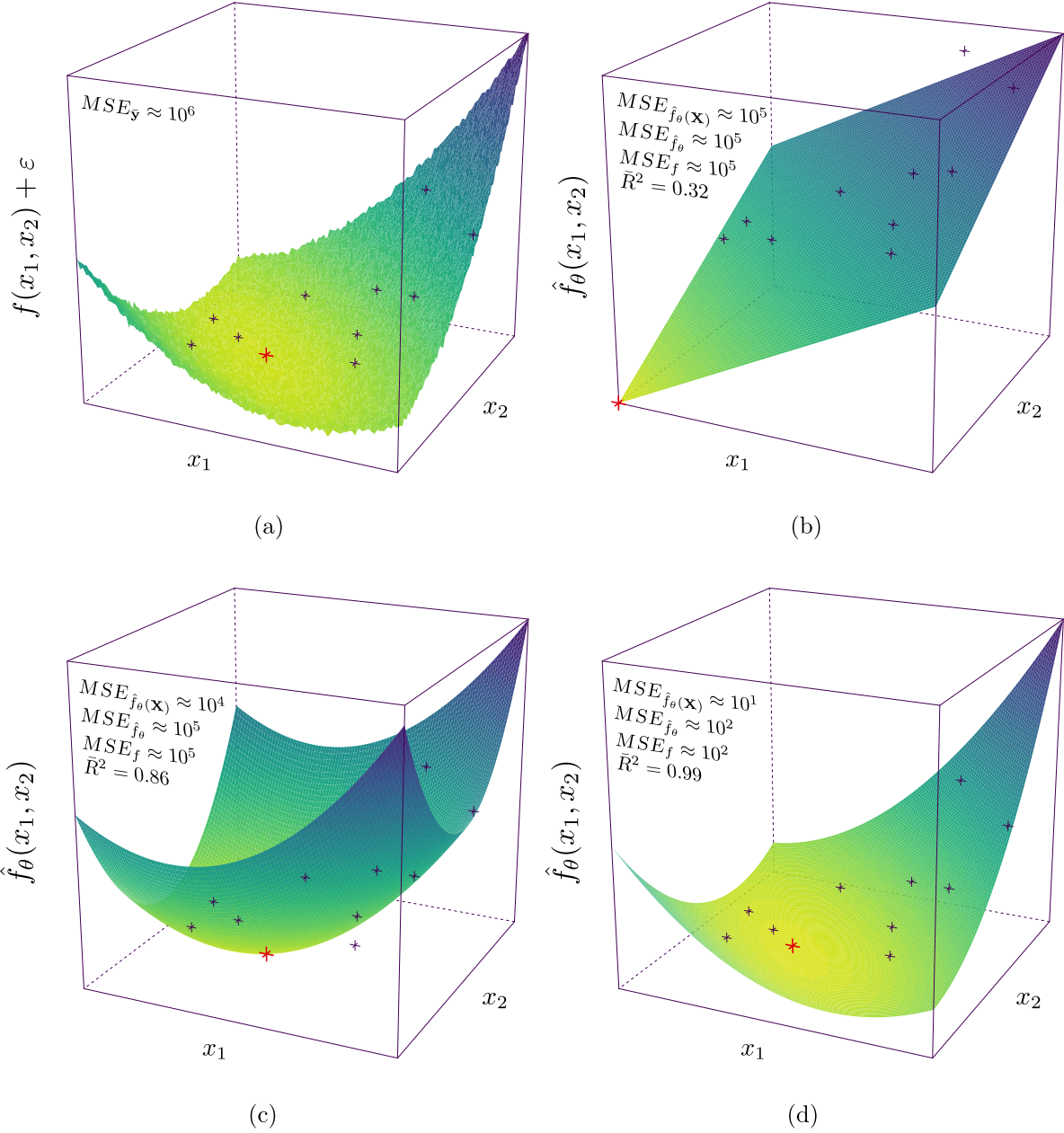
Figure 4.2: Three linear model surrogates for the Booth function, with a \times marking the global optimum and best surrogate predictions. The fixed experimental design \mathbf{X} used to fit all surrogates is marked by \times s. Panel (a) shows noisy measurements of Booth's function, panels (b), (c), and (d) show surrogate predictions for models fit with basis functions sets from Equations 4.11, 4.12, and 4.13, respectively
