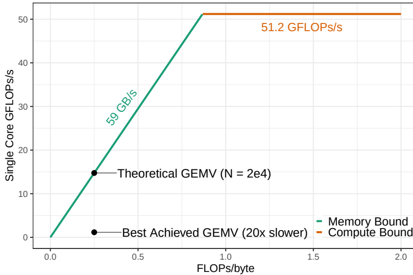
Figure 12.13: Theoretical Roofline graph for the Xeon E5-2630v3 processor [10, 116], showing the best point we found during all experiments with the memory-bound dgemv3 SPAPT kernel
