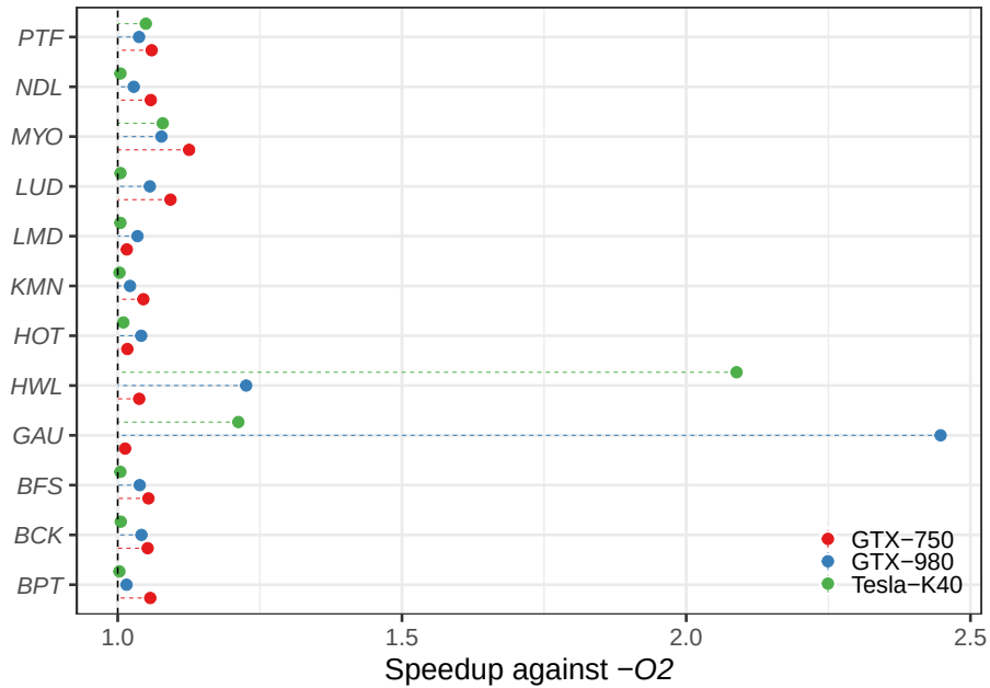
Figure 9.3: Mean speedup over 30 repetitions of the tuned solutions for Rodinia kernels versus the opt-level = 2 baseline
