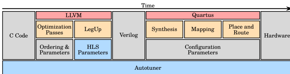
Figure 10.3: High-Level Synthesis compilation process. The autotuner search space at the HLS stage is highlighted in blue
