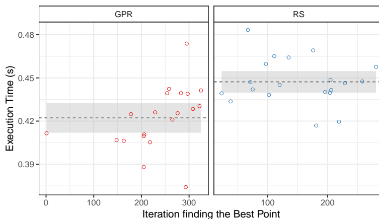
Figure 12.9: Best bicg configurations and iterations that found them, for Gaussian Process Regression with Expected Improvement acquisition function (GPR), and uniform Random Sampling (RS), with a budget of 400 measurements.
