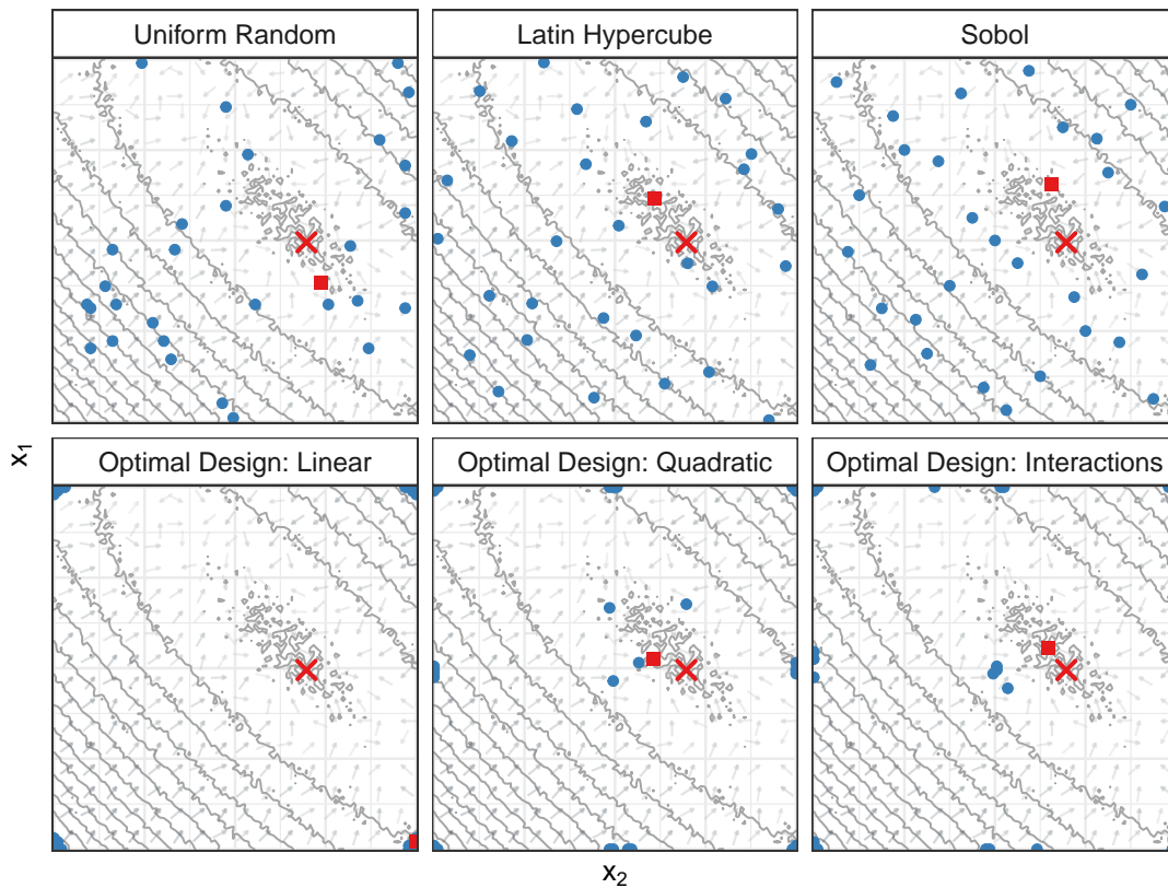
Figure 5.5: Exploring the search space for Booth's function with different methods, using a fixed budget of 30 measurements. A \times marks the global optimum, a \blacksquare marks the best point found by each strategy, and \bullet s mark measurements
