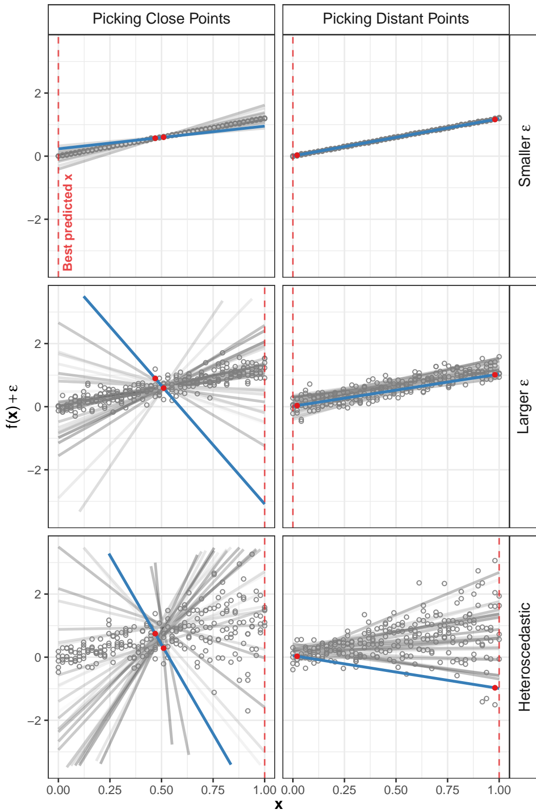
Figure 5.1: Fitting linear models using 30 distinct random sets of two measurements, in experimental settings with different properties of the error \epsilon . One arbitrary model fit is highlighted to show the distance between the design points
