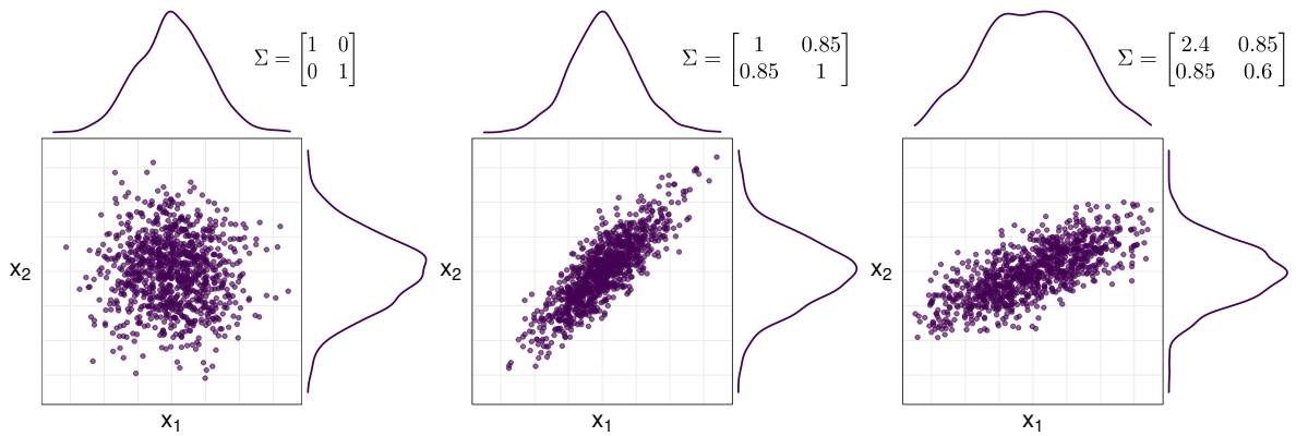
Figure 4.3: Effects of three covariance matrices on a multivariate normal distribution with mean vector \boldsymbol{\mu} = [0 \ 0]^T and covariance matrix \boldsymbol{\Sigma} as shown on the upper right corner of each plot
