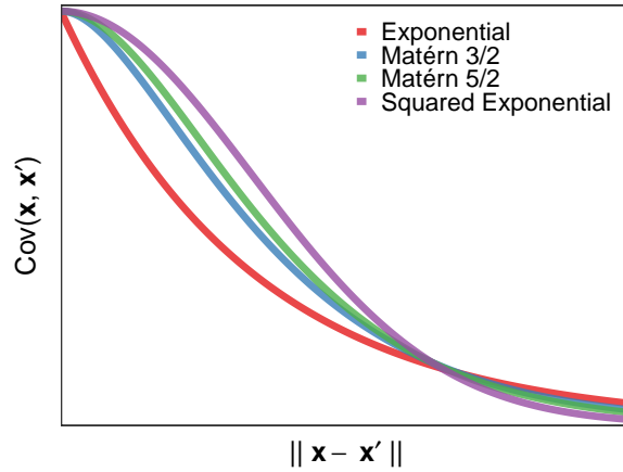
Figure 4.5: Covariance of points (\mathbf{x}, \mathbf{x}') according to four covariance functions based on the distance \|\mathbf{x} - \mathbf{x}'\| . Expressions for each kernel are shown in Table 4.1, and Matérn kernels use parameters \nu_1, \nu_2 = \{\frac{3}{2}, \frac{5}{2}\}
