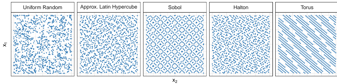
Figure 5.4: Comparison of 1000 samples obtained with different sampling methods. The Latin Hypercube design was produced with the DiceDesign R package [77], and was optimized after an initial sampling, with Simulated Annealing. Sobol, Halton, and Torus are low-discrepancy sequences from the randtoolbox R package [63].
