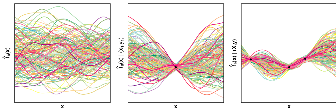
Figure 4.7: Fitting a Gaussian Process to three noisy observations, in the same conditions and with the same panel structure in Figure 4.6
