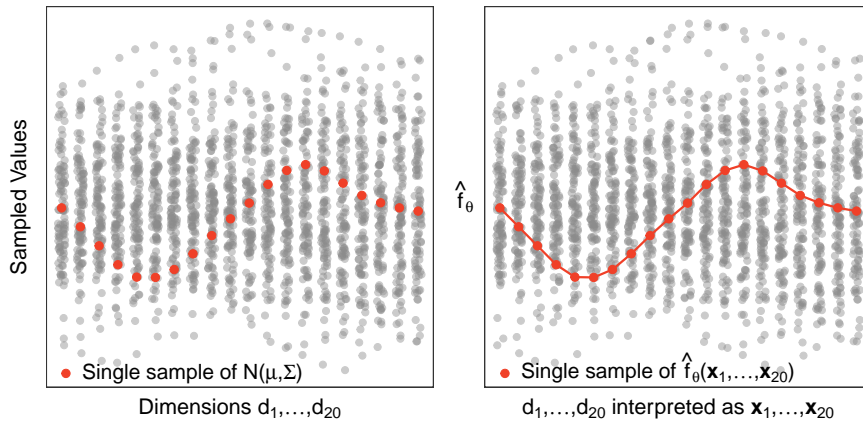
Figure 4.4: Reinterpreting the unrolled dimensions of 100 samples of a 20 dimension multivariate normal, on the left panel, to obtain 100 samples of functions evaluated on 20 different input points, on the right panel
