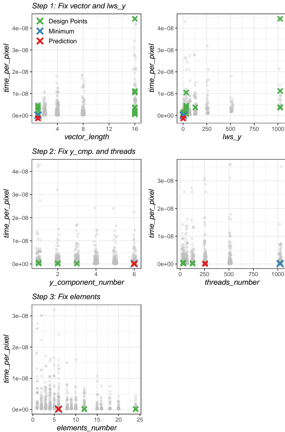
Figure 11.6: Overview of a single DLMT run. Each panel shows a view of the completely evaluated search space, from the perspective of one of the factors eliminated in a given step. A \times marks the predicted best level of each factor, a \times marks the factor level on the global optimum, \times s mark the design points measured at each step, and gray points mark the completely evaluated search space
