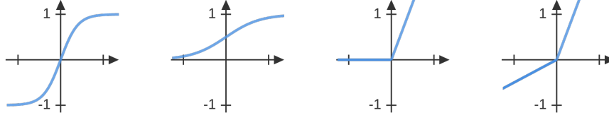
Figure 2.4: Commonly used activation functions. From left to right : hyperbolic tangent (tanh), sigmoid, Rectified Linear Unit (ReLU) and leaky ReLU.
