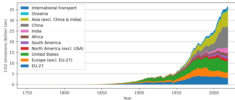
Figure 2: Global CO 2 emissions per year
