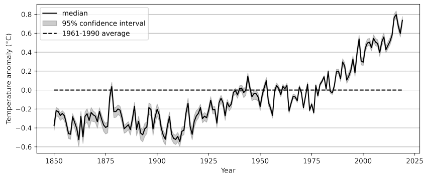
Figure 3: Temperature anomaly compared to the average of the 1961-1990 period
