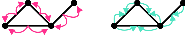
Figure 3.10: Message passing: first, vertices are updated depending on the latent variable of the edges to which they are connected (left), and then edges are updated depending on the latent variables of the vertices to which they are connected (right).
