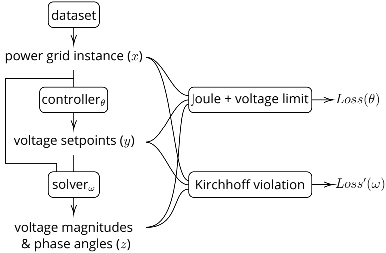
Figure 9.1: Voltage setpoint control. Two neural networks, namely \text{controller}_\theta and \text{solver}_\omega , are trained jointly.
