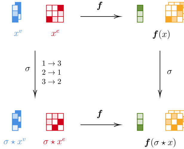
Figure 3.6: Permutation-equivariant mapping. The ordering of the output f(x) reflects the ordering of the input x . While the output of f is different when applied to x and \sigma \star x , the underlying graph is strictly identical, and the same permutation \sigma allows to switch from one output to the other.
