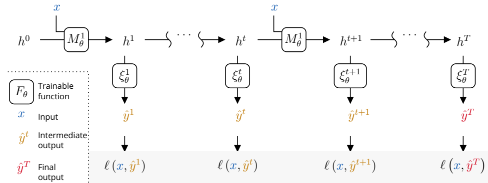
Figure 4.7: Previously used neural network architecture. The operator M_{\theta}^t encompasses all the message passing operations performed in lines (10-13) of Algorithm 3. All intermediate predictions appear in the loss of equation 4.19, while the current H2MGNN only penalizes the final prediction.
