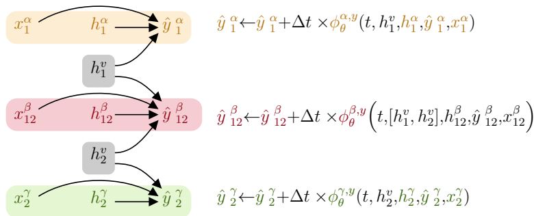
Figure 4.4: Updating hyper-edge latent variables.
