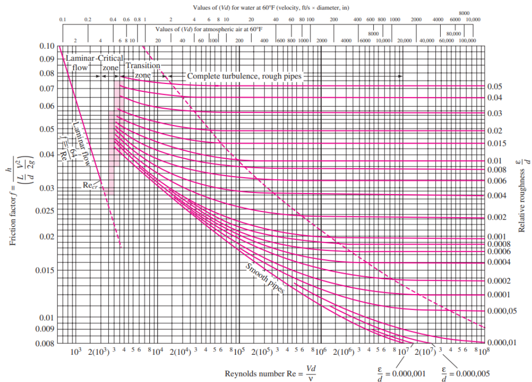
Figure 1.17 The Moody chart for pipe friction with smooth and rough walls.
