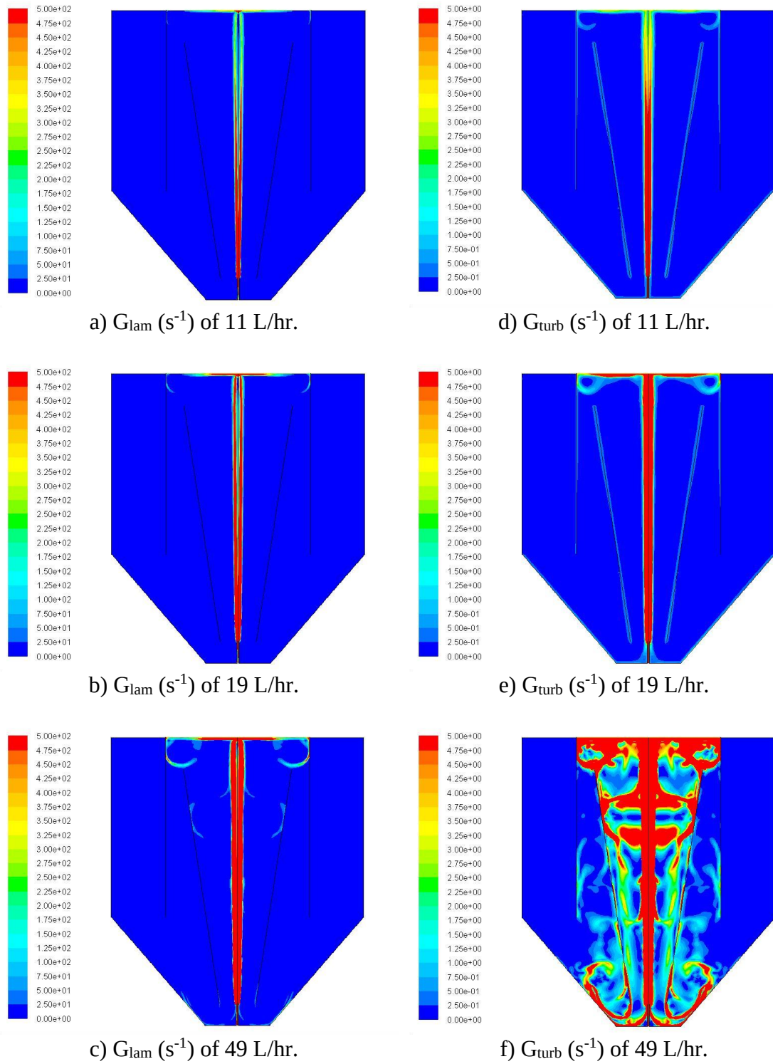
Figure 5.10 Contours of G_{\text{lam}} and G_{\text{turb}} of the SSP
