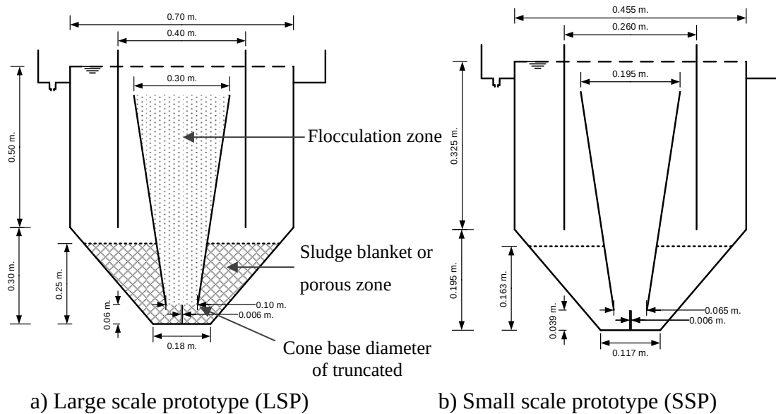
Figure 2.1 Scheme hydrodynamic diagram of jet clarifiers
