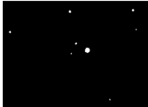
Figure 2.18 Binarized image
