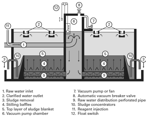
a) Sludge blanket clarifiers
