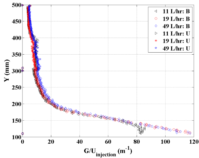
Figure 4.14 The vertical profile of velocity gradient ( G ) divided by the inlet velocity ( U_{injection} ) of 11 L/hr., 19 L/hr., and 49 L/hr. flow rates
