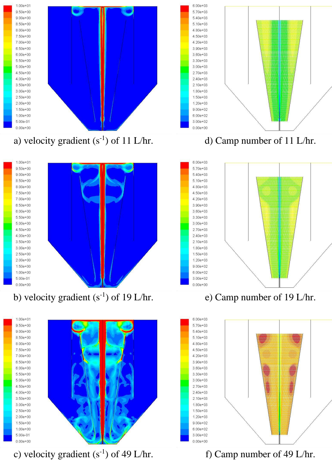
Figure 5.11 Contours of velocity gradient and Camp number of the SSP
