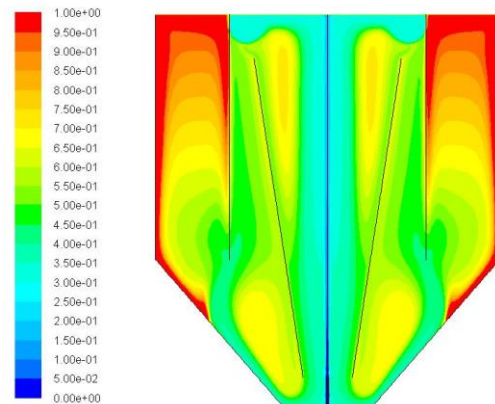
d) non-dimensional time ( \theta ), 11 L/hr.
