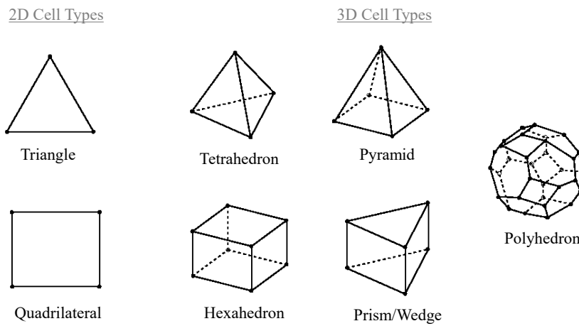
Figure 3.9: Mesh cell types
