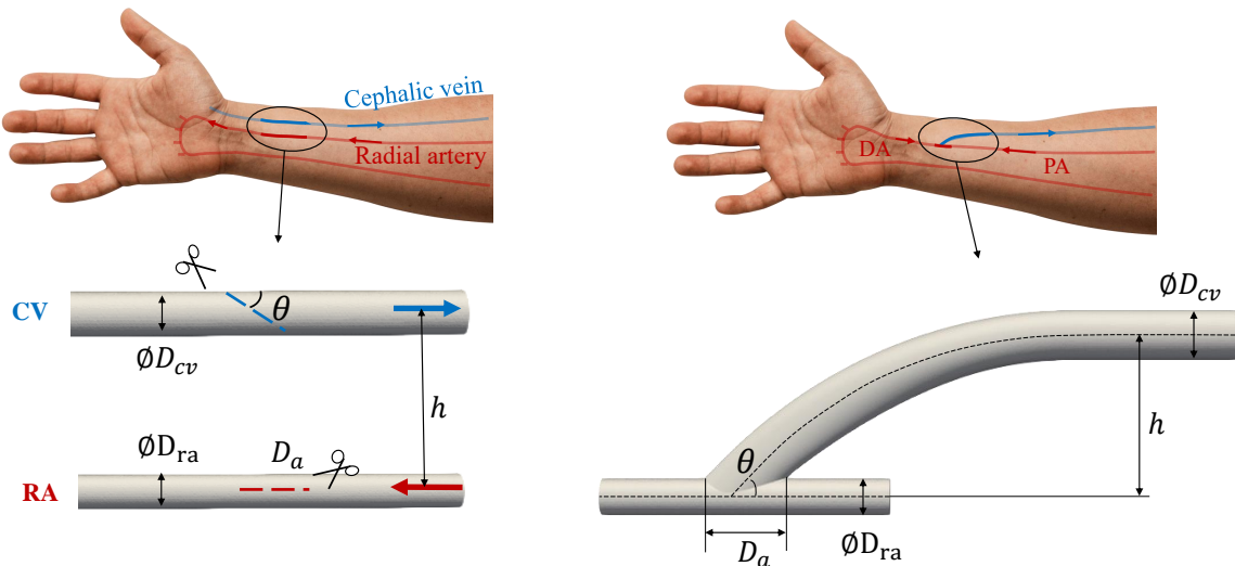
Figure 2.1: RCAVF geometric parameters
