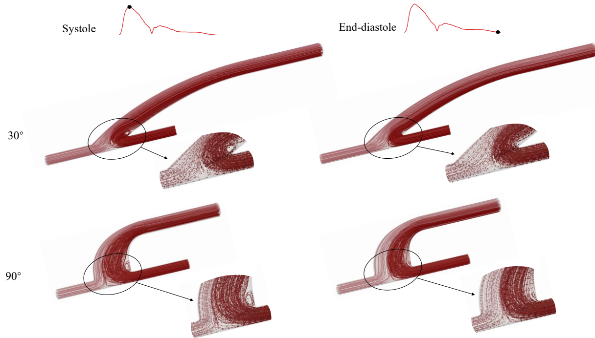
Figure 3.37: Streamlines in non-mature models ( \theta = 30^\circ and \theta = 90^\circ )
