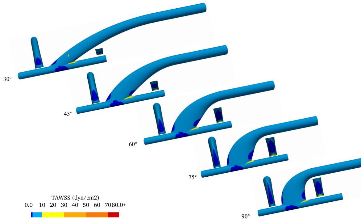
Figure 3.40: TAWSS distributions in non-mature models
