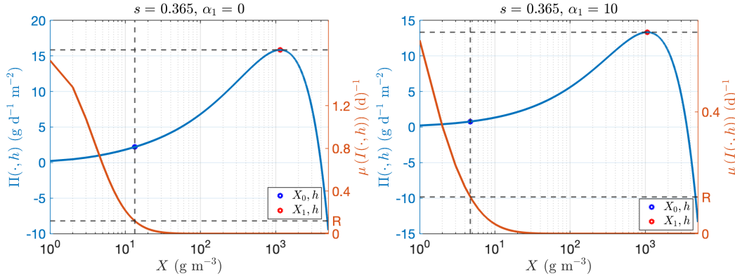
Figure 2.8: Productivity ( \Pi ) with respect to biomass concentration ( X ) for h = 0.15 m. Left: \alpha_1 = 0 m -1 . Right: \alpha_1 = 10 m -1 .
