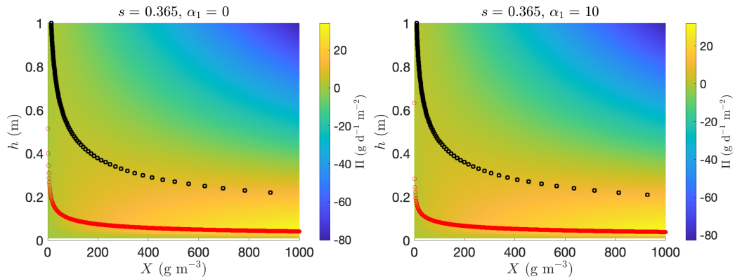
Figure 2.9: Global behaviour of productivity ( \Pi ) with respect to depth ( h ) and biomass concentration ( X ). Left: \alpha_1 = 0 \text{ m}^{-1} . Right: \alpha_1 = 10 \text{ m}^{-1} . The red circles represent the suboptimal couple (X, h) where \Pi finds its maximum in the direction of h for a given X . The black squares represent the suboptimal couple (X, h) where \Pi finds its maximum in the direction of X for a given h .
