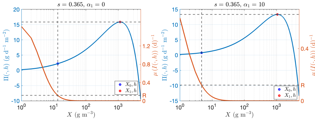
Figure 2.8: Productivity ( \Pi ) with respect to biomass concentration ( X ) for h = 0.15 m. Left: \alpha_1 = 0 m -1 . Right: \alpha_1 = 10 m -1 .
