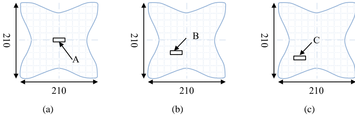
Figure 5-11 Schematic of: (a) In the centre location, (b) In the middle area and (c) In the locking area (dimensions in mm).
