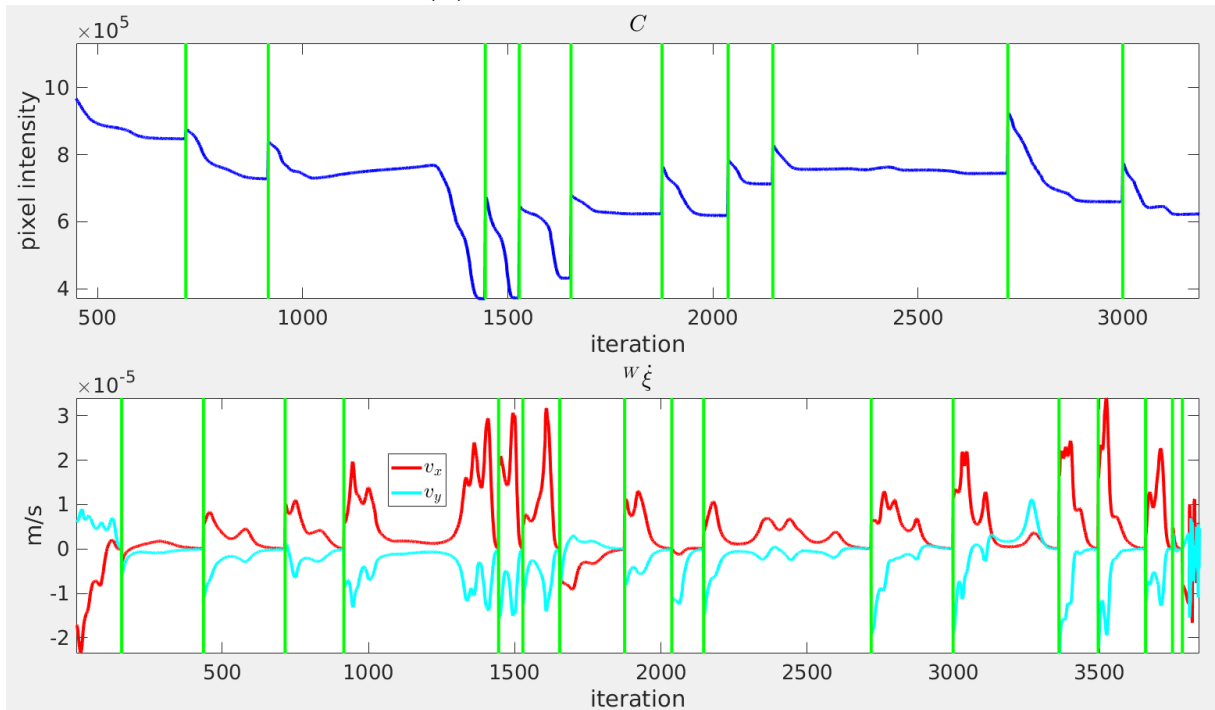
Figure 7.6: Cost C (top) and input velocity \mathbf{u} = W\dot{\xi} (bottom) evolution of the textureless zone and outdated mesh cases. Element update appears in green.
