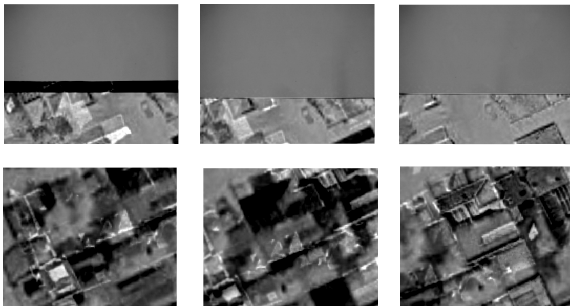
Figure 7.3: Dragging error corrected. Two rows of images of difference, between the onboard image {}^WI and the desired virtual image {}^VI^* , show the issue where the dragging error began (left column), was carried (central column) and corrected (right column).
