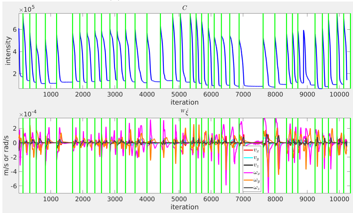
Figure 7.5: Cost C (top) and input velocity \mathbf{u} = W\dot{\xi} (bottom) evolution of the approximated cases. Element update appears in green.
