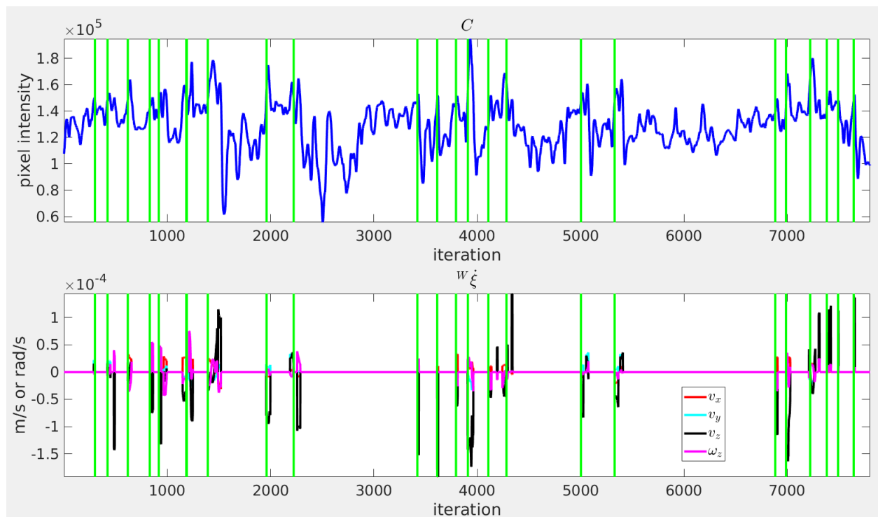
Figure 3.9: Cost \mathcal{C} and control input \bar{\mathbf{u}} evolution of the indoor hybrid servoing. Vertical lines indicate the memory update.
