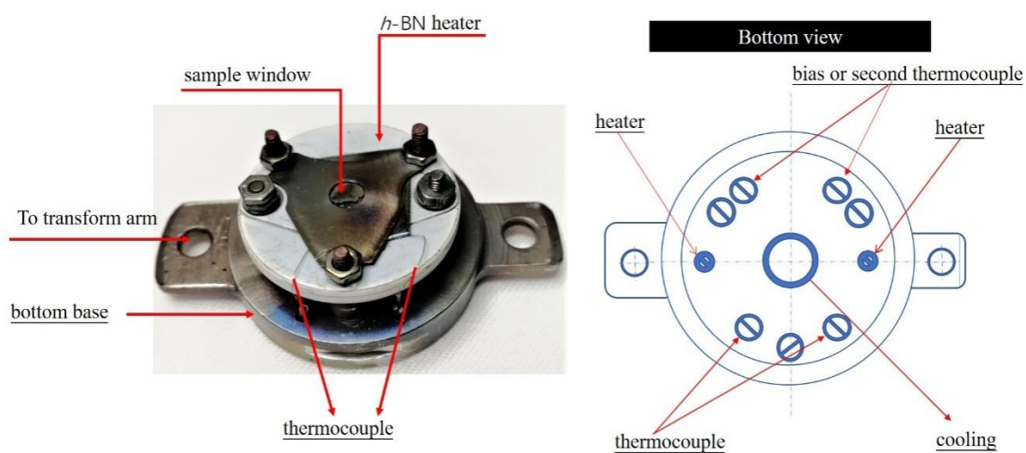
Sample holder for UHV-VPR-XPS system
