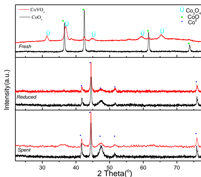
Figure 5-2. The ex situ XRD patterns of catalysts after different treatment, the spent samples were used for COPrOx test under atmospheric pressure.
