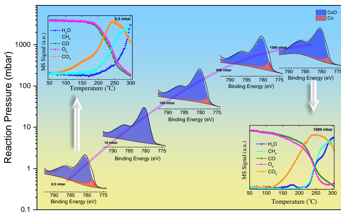
Figure 3-10. The XPS Co 2p 3/2 spectra of PreH 2 .Co measured after COPrOx reaction at 210 °C at various total pressures. The Co 2p 3/2 spectrum at 0.5 mbar is in situ NAP-XPS, while higher pressures Co 2p 3/2 spectra were recorded ex situ after 30 min reaction followed by reactants evacuation and transfer under vacuum to the XPS spectrometer. The inset graphs show the corresponding QMS data of the consumption of reactants and yields of products as a function of the reaction temperature recorded at 0.5 and 1000 mbar (the reaction temperature in these experiments was expanded up to 300 °C).
