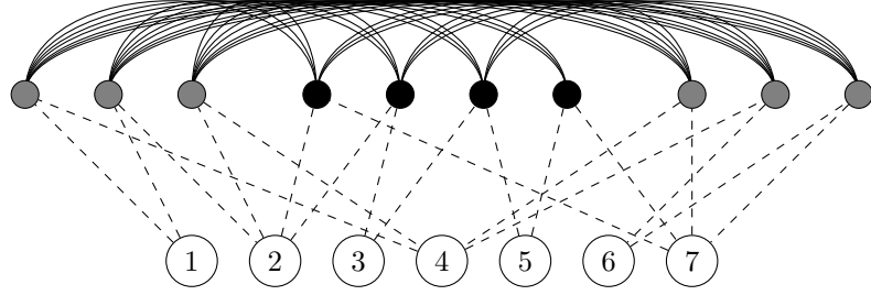
Figure 5.4 – Graph G_I on input I = (\{1, 2, 3, 4, 5, 6, 7\}, \{\{1, 2, 4\}, \{2, 3, 5, 7\}, \{4, 6, 7\}\}, k) . Note that I is a Yes -instance if k = 2 (a solution is e.g., X = \{2, 7\} ) but a No -Instance if k = 1 . Set U is represented in the white numbered nodes, and the other nodes in C_1, C_2 and C_3 in black and gray (the different colors are to help the recognition of the cycles in the figure). In this figure, only the cycles (and not the super-cycles) associated to the sets are represented. To represent the super-cycles, dashed edges must be replaced with a watermelon graph, with p = \lfloor \log(\text{poly}((nm)^2 - n)/(nm)) \rfloor . The nodes and edges incident to R , and the edges incident to the nodes in the dashed edges were omitted.
