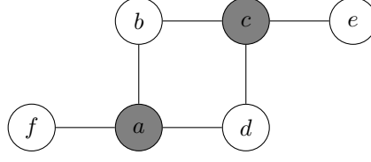
Figure 3.1 – Example a minimal separator, in this case the set \{a, c\} is a minimal b, d -separator. Note that the set \{c\} is also a minimal separator, e.g for pair e and b .
