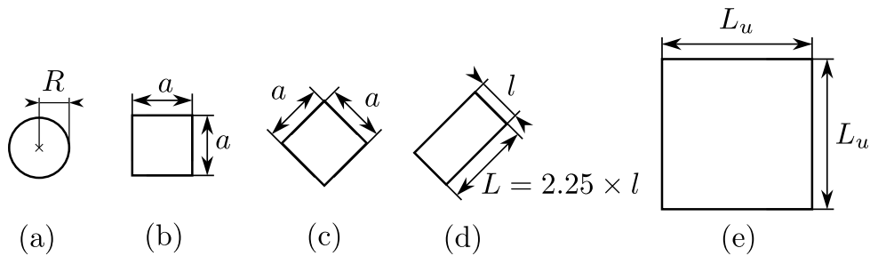
Figure 7.3 – Dimensions for the four inclusions, consisting of (a) a circle, (b) a square, (c) a diamond and (d) a rotated rectangle. The dimensions of the unit cell are also shown (e).
