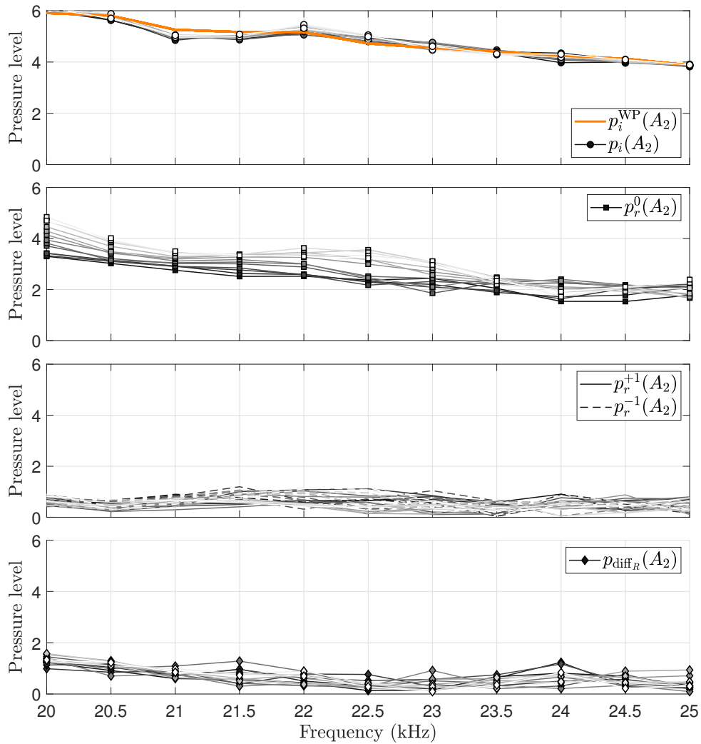
Figure 8.18 – Incident pressure ( p_i ), reflected pressure of the 0 th mode ( p_r^0 ) and of the diffracted modes \pm 1 ( p_r^{\pm 1} ) and edge-diffracted pressure ( p_{diff_R} ) at the central position A_2 on the reflection side. The incident pressure measured without the panel ( p_i^{WP} ) is also plotted. The graduation of grey represents the y -positions along the unit cell.
