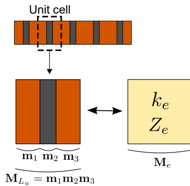
Figure 2.2 – Finite periodic multilayered medium characterised by a symmetric unit cell, for which a fluid effective medium is defined by an effective wavenumber and an effective impedance obtained using the transfer matrix M_{L_u} of the periodic unit.
