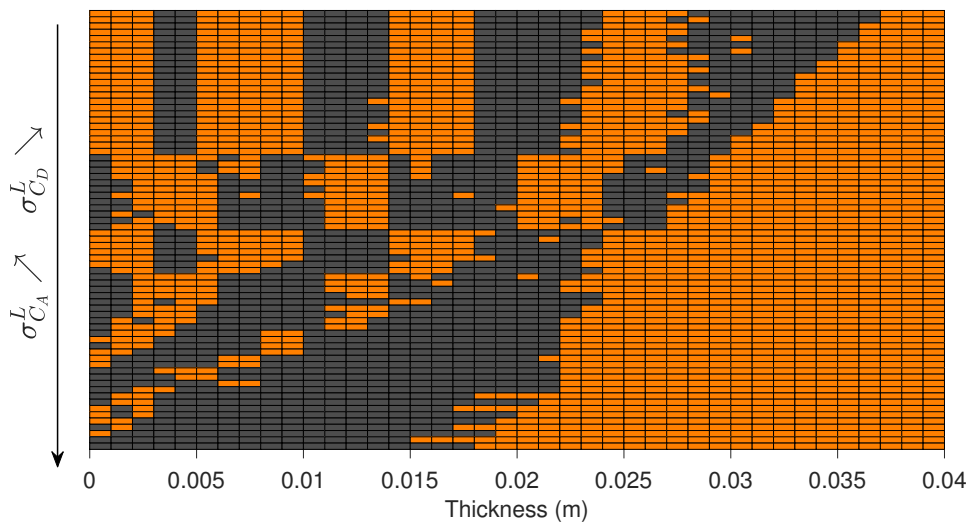
Figure 3.16 – Layer arrangements for all the solutions of the Pareto front, arranged according to decreasing \sigma_{C_D}^L , and thus increasing \sigma_{C_A}^L . The orange color represents the polyurethane while the dark grey color corresponds to the stainless steel.
