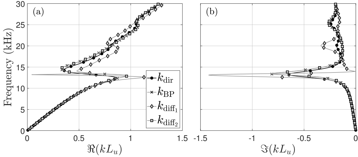
Figure 5.9 – Dispersion curves for the reduced wavenumber obtained with the direct inversion method ( k_{\text{dir}} ), with the Bianco and Parodi method ( k_{\text{BP}} ), with the differential method Version 1 ( k_{\text{diff}_1} ) and with the differential method Version 2 ( k_{\text{diff}_2} ).
