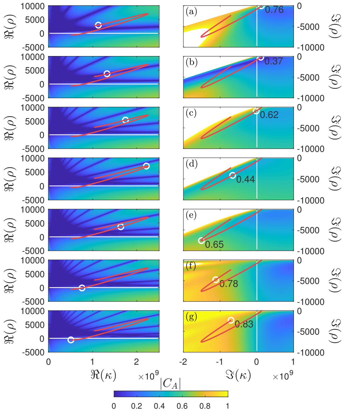
Figure E.17 – Frequency paths for a medium of length L = 3 \times L_u = 4.8 cm at the frequencies (a) 6 kHz, (b) 9.7 kHz, (c) 12.3 kHz, (d) 13.7 kHz, (e) 14.7 kHz, (f) 16.5 kHz and (g) 20 kHz. On the \Re -maps (left hand side), the white circle shows the values of \Re(\kappa) and \Re(\rho) obtained for the unit cell in Figure E.14. The red line represents the complete path. In the \Im -map obtained for these values (right hand side), the white circle shows the values of \Im(\kappa) and \Im(\rho) obtained for the unit cell and the value of the anechoism coefficient.
