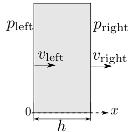
Figure 2.1 – Pressures and normal particle velocities at the inlet/outlet of a medium of thickness h , where the subscript left refers to the face on the left hand-side and the subscript right to the face on the right hand-side of the medium.
