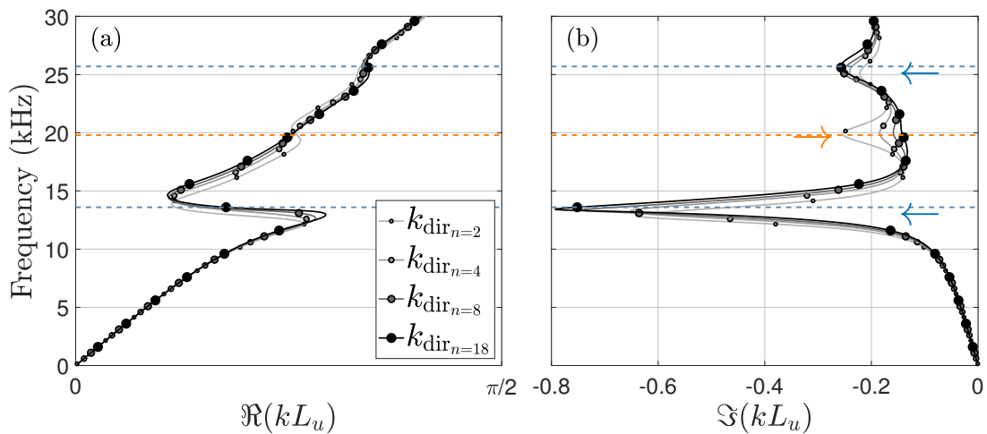
Figure 5.14 – Effective wavenumbers as a function of angular frequency obtained with the direct inversion method for media comprising 2, 4, 8 and 18 unit cells.
