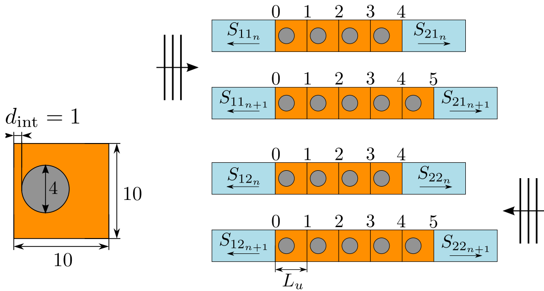
Figure 6.4 – Representation of the asymmetric locally resonant unit cell. Dimensions are in millimetres. The differential method is applied to the segmented media comprising of 4 and 5 unit cells for application of the differential method. The direct inversion method is applied to the first medium, containing 4 unit cells.
