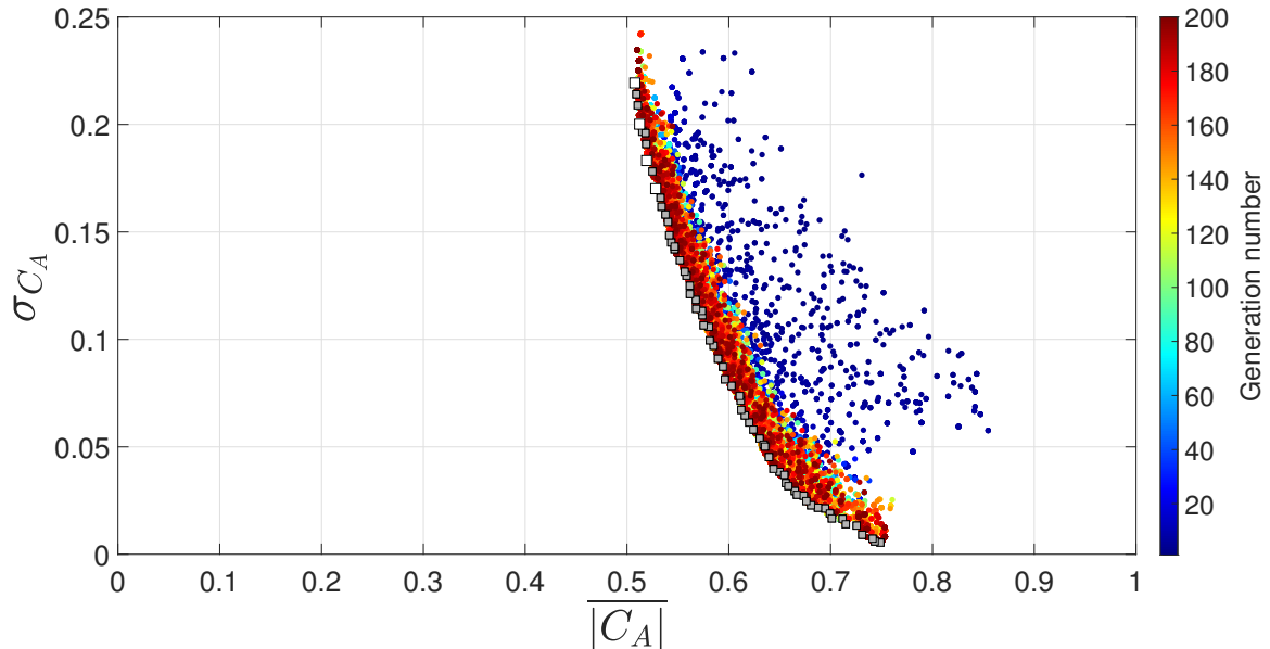
Figure 3.7 – Figures of merit for all individuals in the population, as a function of the generation number. Grey squares represent the Pareto front obtained at the last generation. White squares highlight the scores of 4 selected configurations.
