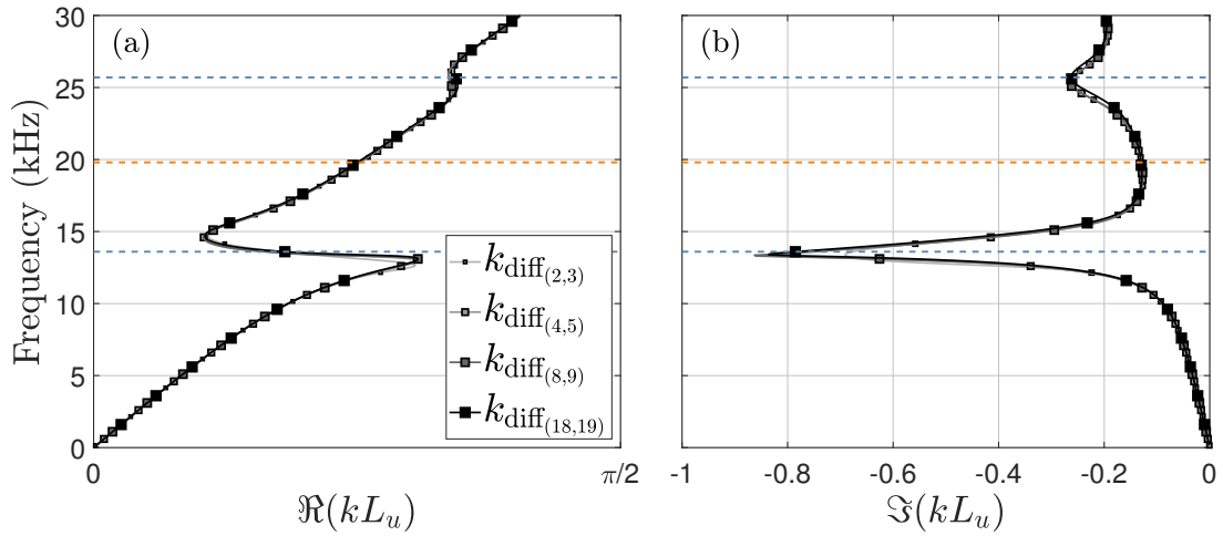
Figure 5.15 – Effective wavenumbers as a function of angular frequency obtained with the differential method for the unit combinations (2,3), (4,5), (8,9) and (18,19).
