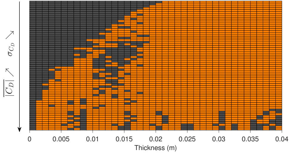
Figure 3.12 – Layer arrangement for all the solutions of the Pareto front, arranged according to decreasing \sigma_{C_D} , so increasing |C_D| . The orange color represents the polyurethane while the dark grey color corresponds to the stainless steel.
