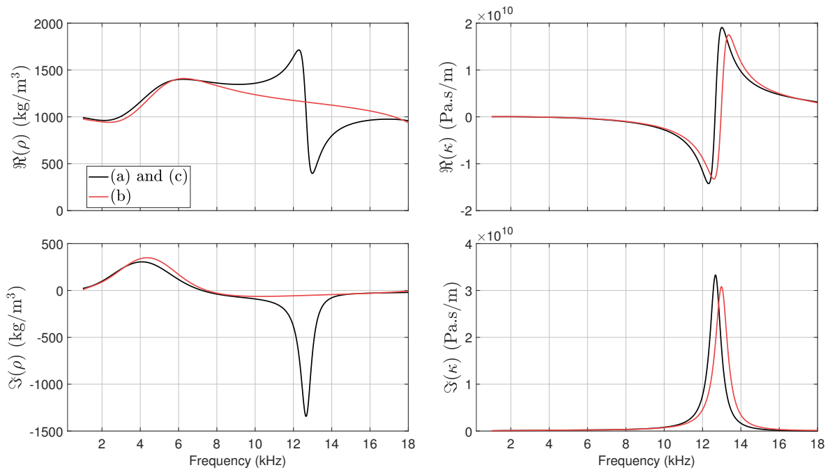
Figure 6.16 – Effective density and bulk modulus for the asymmetric layers presented in Figure 6.14.
