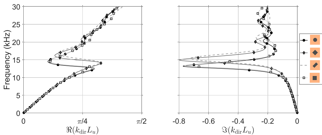
Figure 7.4 – Dispersion curves obtained using the direct inversion method for the four different units of surface area \mathcal{A} = 16 \text{ mm}^2 .
