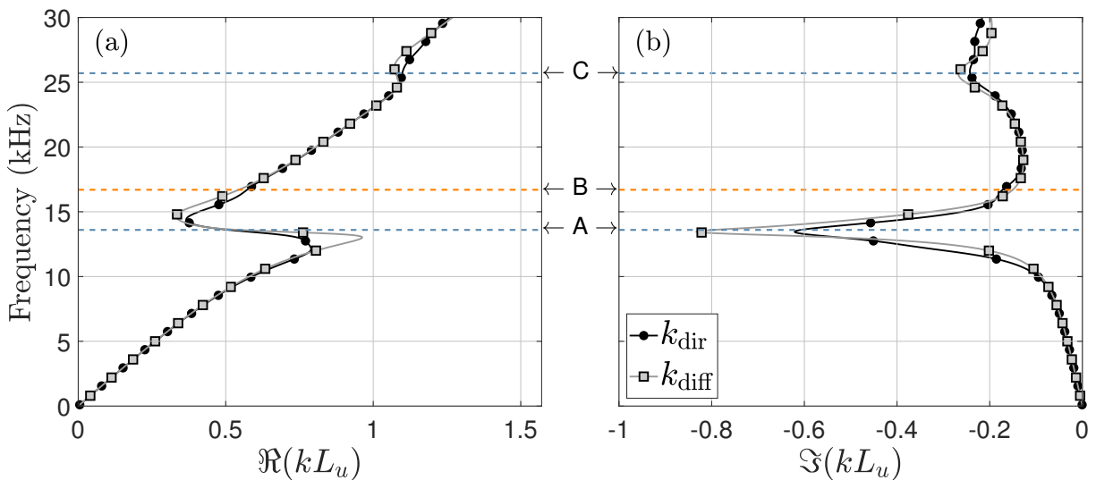
Figure 6.5 – Effective wavenumbers obtained using the direct inversion method and the differential method for the asymmetric unit with macro-inclusions.
