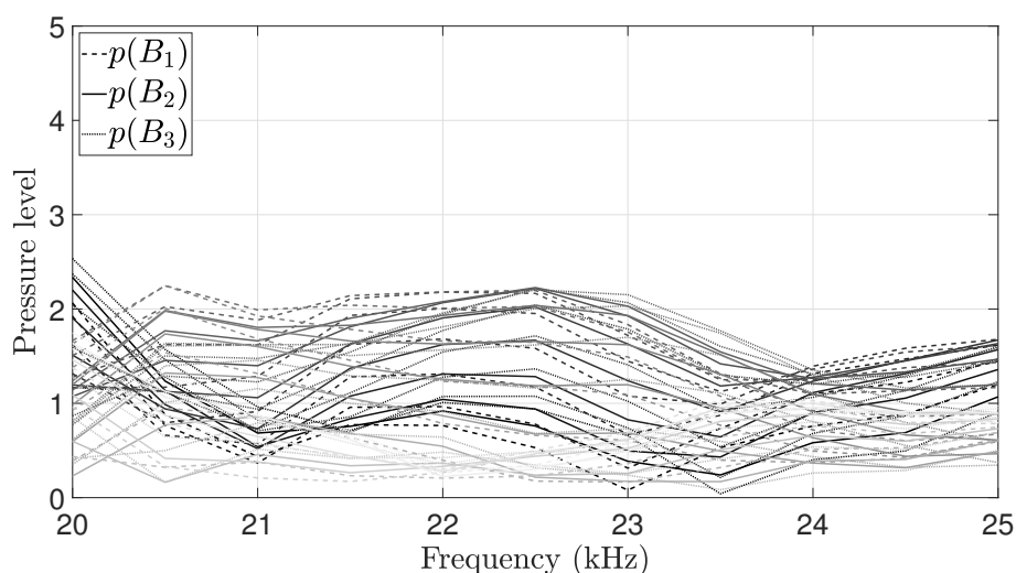
Figure 8.17 – Pressure amplitudes measured at the 3 positions B_1 , B_2 and B_3 on the transmission side. The graduation of grey represents the y -positions along the unit cell.
