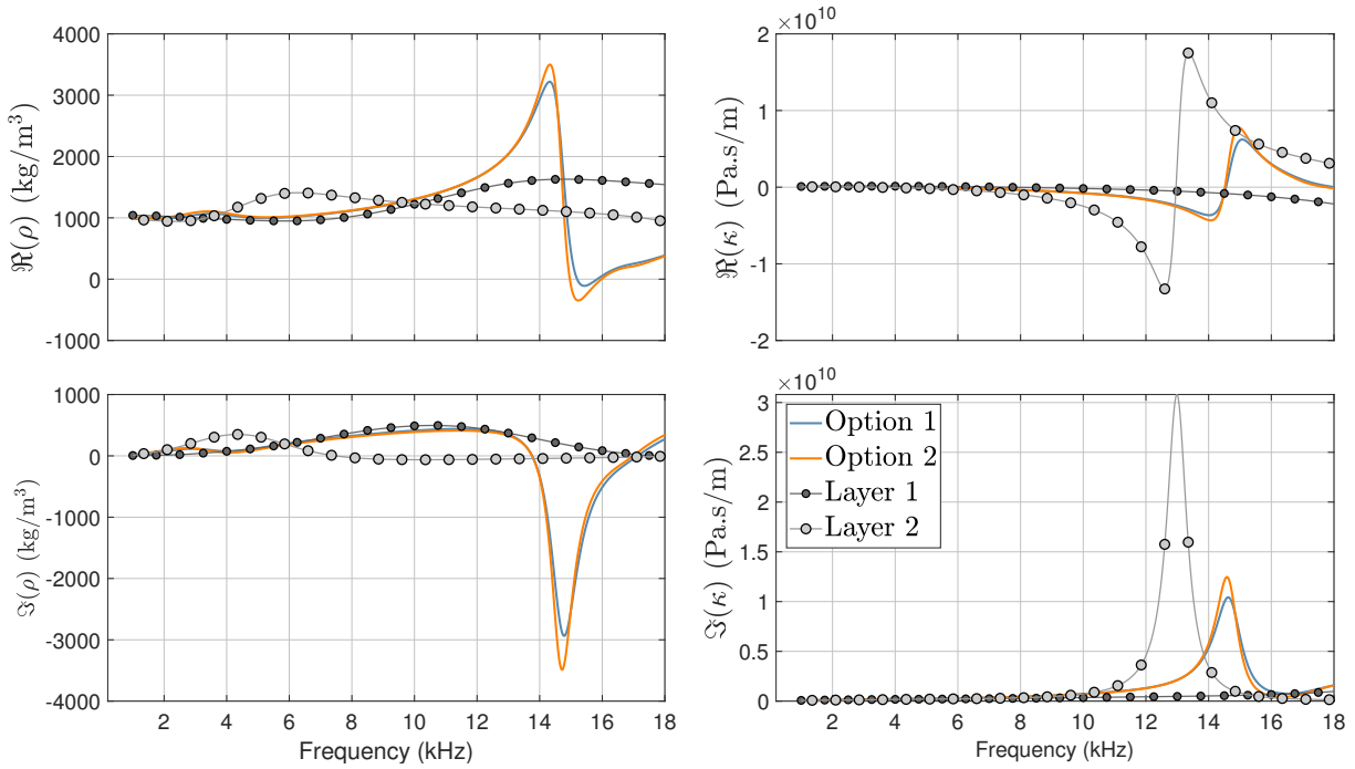
Figure 6.22 – Effective bulk Modulus and mass density for the bi-layer Alberich design.
