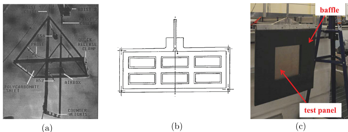
Figure 1.15 – (a) Measurement rig, sample and airbox [103]. (b) Surface hydrophone [99]. (c) Panel mounted in baffle [104].
