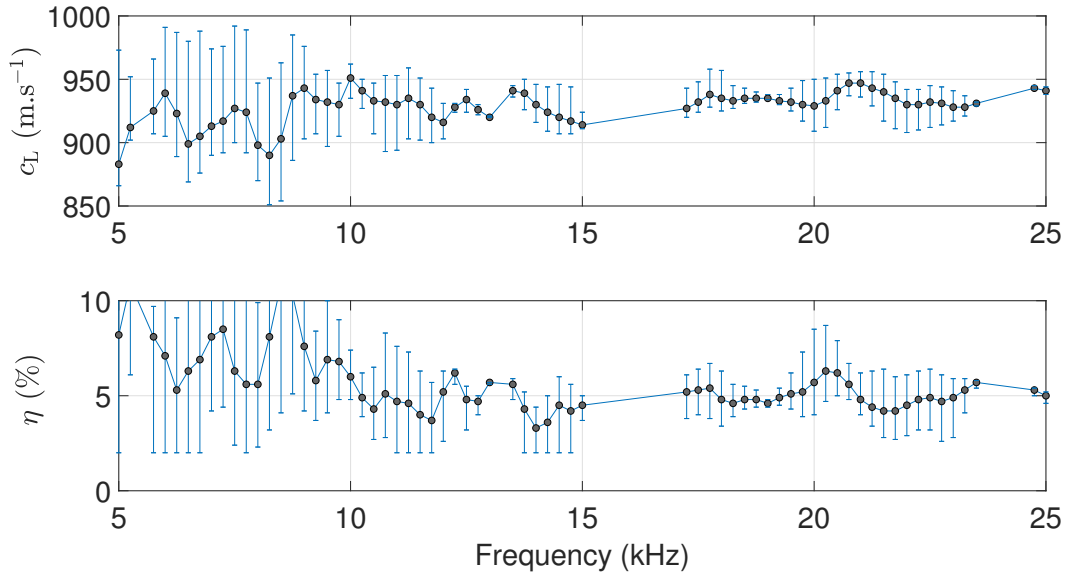
Figure 4.17 – Speed of sound obtained using the minimisation criterion C given in Equation (4.9) for C < \epsilon , with \epsilon = 0.13 . The grey dots are the values of the complex speed of sound that give the global minimum of C whereas the error bars are the sets of solutions that satisfy C < \epsilon .
