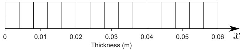
Figure 3.2 – Multilayered medium before the affectation of materials by the optimisation algorithm. Thicknesses are displayed in meters. The acoustic wave is incident on the face x = 0 whereas x = 0.06 corresponds to the transmission side. For the calculation of both the anechoism and hull decoupling coefficients, the hull is considered at on the right-hand side.
