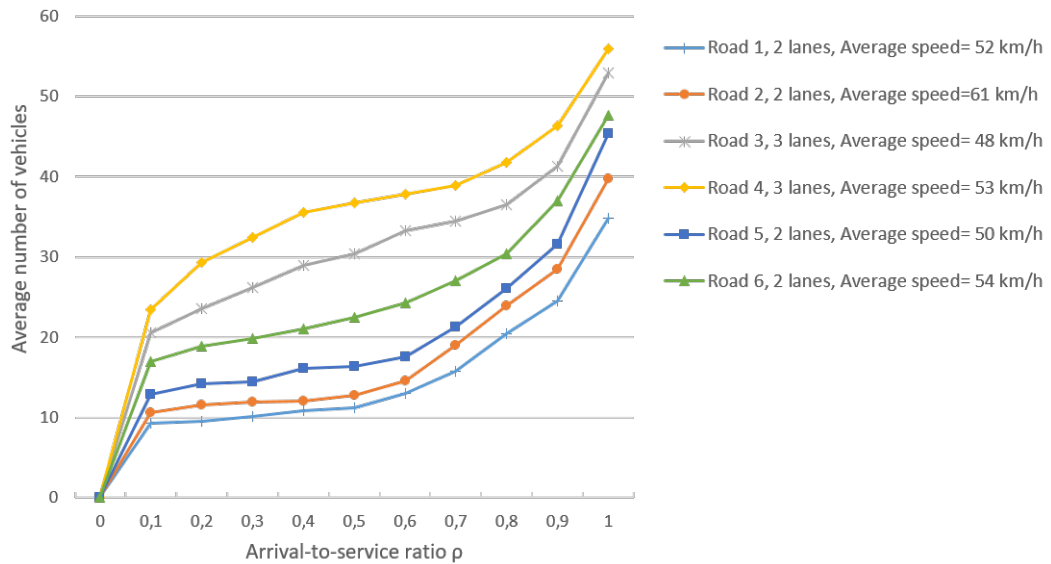
Figure 5.5: Per road average number of vehicle against density
