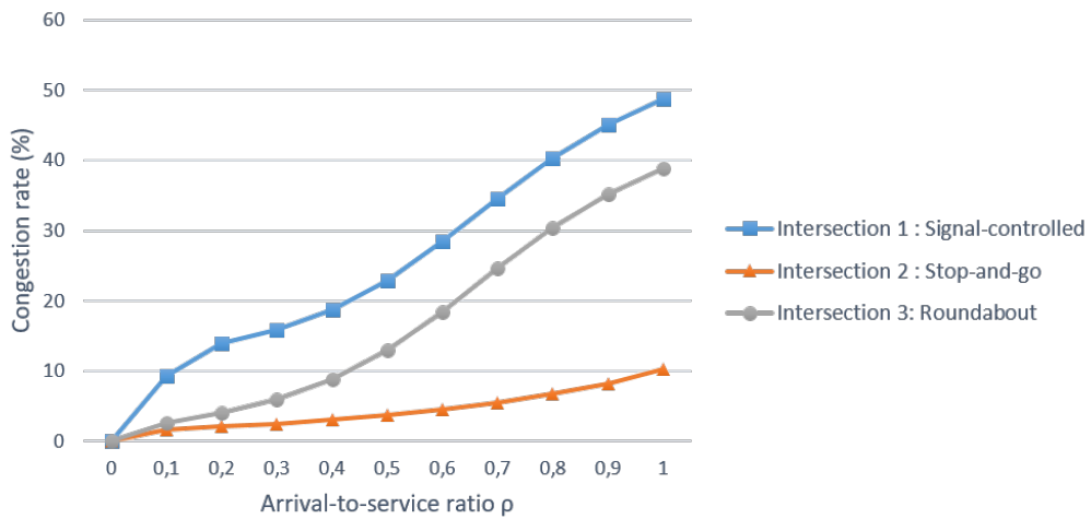
Figure 5.9: Per intersection congestion rate vs density
