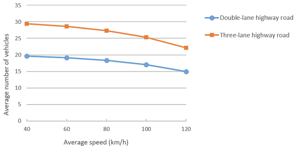
Figure 4.6: Average number of vehicles vs. Average speed
