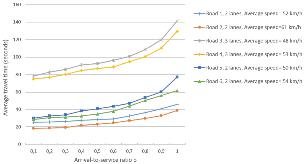
Figure 5.6: Per road average travel time against density
