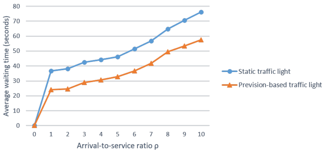
Figure 5.16: Average waiting time: Pre-timed traffic light vs Actuated traffic light
