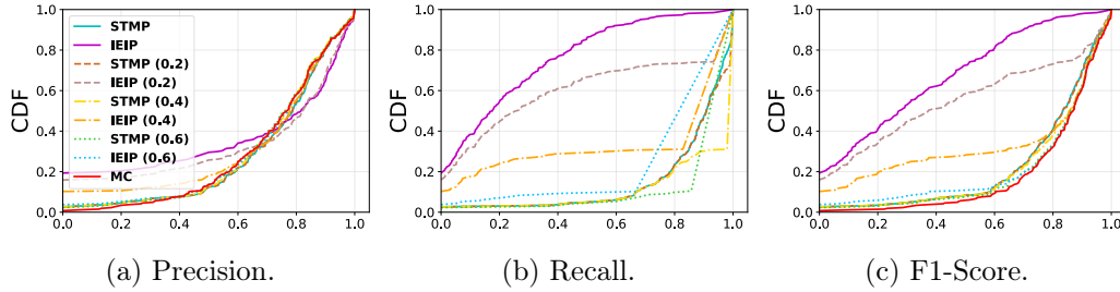
Figure 6.6: Performance comparison for returns forecasts.
