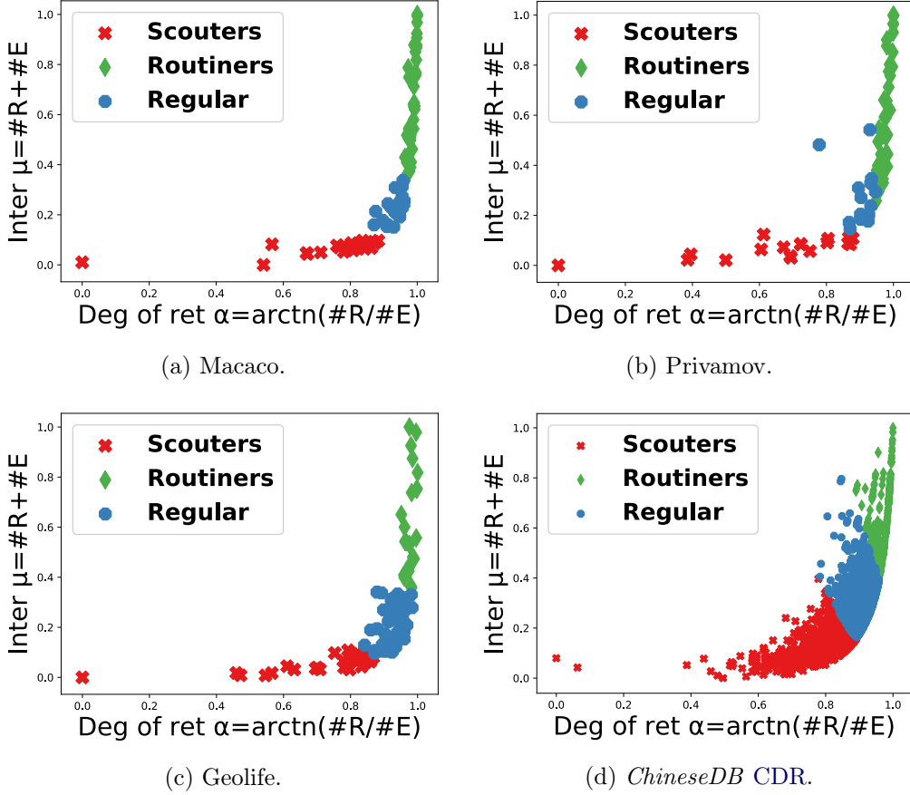
Figure 4.7: Mobility Profiling.
