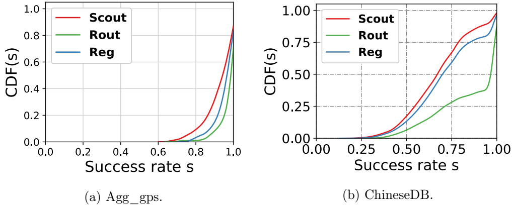
Figure 5.9: Effect of novelty-seeking records replacement with stationarity stuffing on the success rate score s_u of the \text{MC}(1) predictor per mobility profile.
