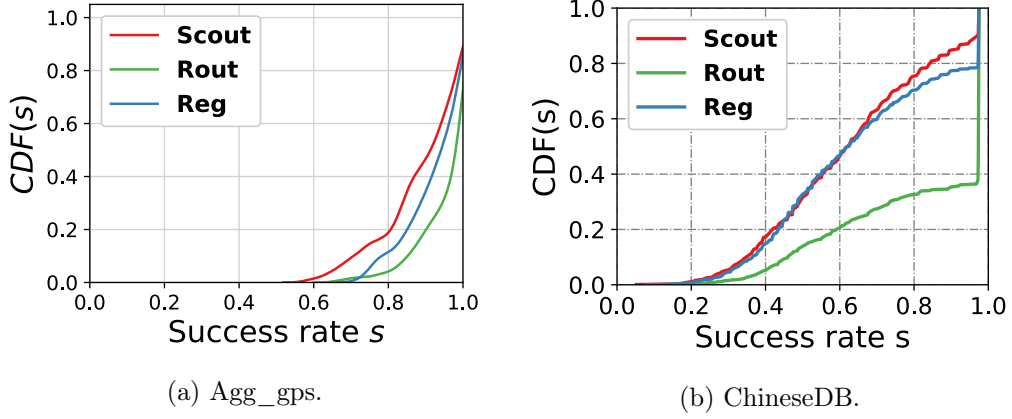
Figure 5.10: Effect of novelty-seeking records random replacement on the success rate score s_u of the \text{MC}(1) predictor per mobility profile.
