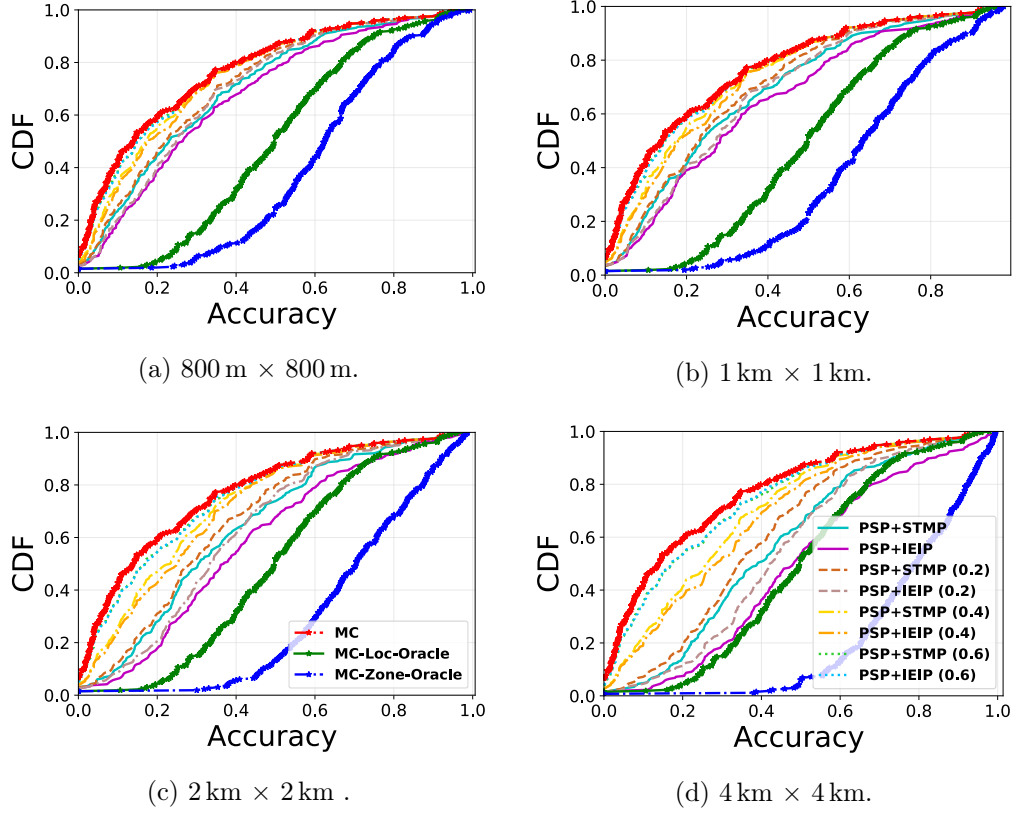
Figure 6.9: Accuracy of the PSP (common labels).
