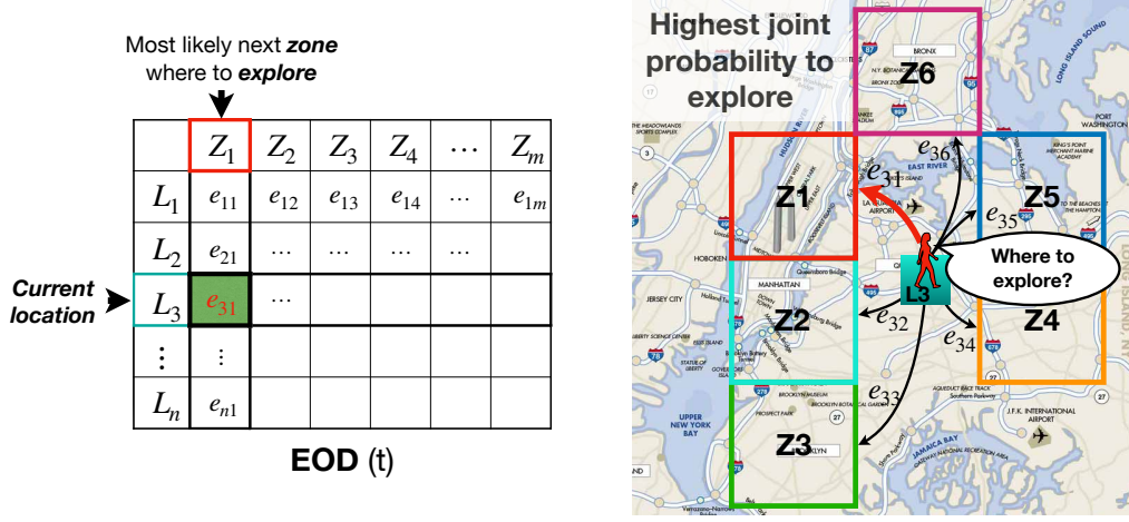
Figure 6.3: Joint Zone-Predictor.
