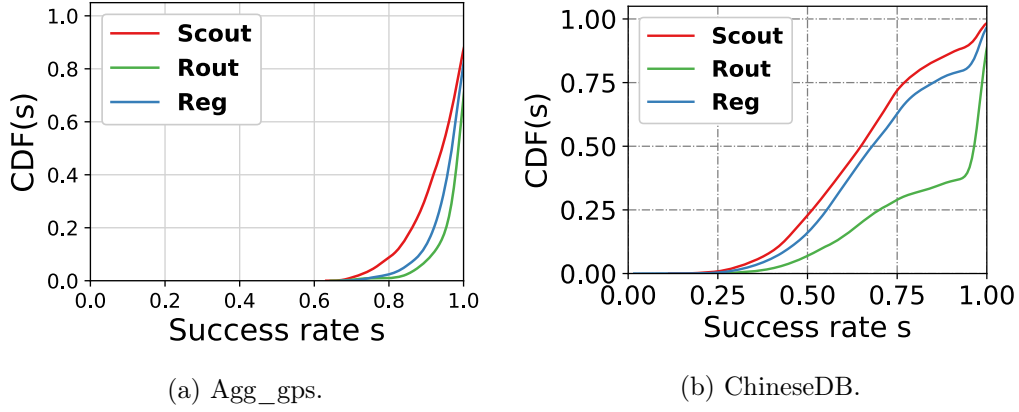
Figure 5.8: Effect of novelty-seeking records removal on the success rate score s_u of the \text{MC}(1) predictor per mobility profile.
