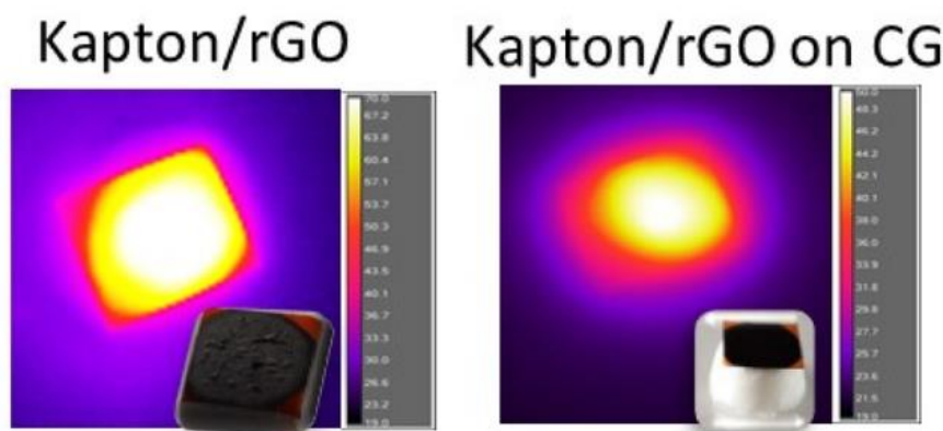
Figure 4.22: Thermal images captured by an infrared (IR) camera (Thermovision A40) of the Kapton/rGO substrate without and with a CG upon NIR illumination at 1 W cm -1 .
