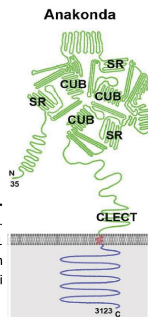
Figure 69. Anakonda structure. SR: Scavenger Receptors domain. CUB: Complement/UEGF/BMP1 domain. CLECT: C-type lectin domain. Adapted from (Higashi and Miller 2017)
