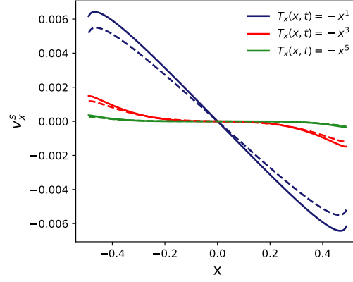
FIGURE 3.3: Comparison between exact (dashed line) and approximated zeroth-order (solid line) solutions of v_x^s with \epsilon = 10^{-3} . The traction force is chosen to be of the polynomial form T(x, t) = -x (blue), T(x, t) = -x^3 (red) and T(x, t) = -x^5 (green), in order to satisfy the constraint \int_{-1}^1 T_x(x, t) dx = 0 , imposed by the force balance.
