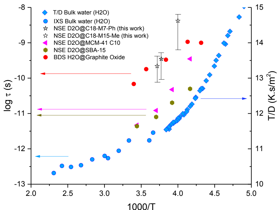
Figure 6.17: Dynamics of bulk and confined water. Relaxation times of Bulk H 2 O (blue circles), the continuation of the curve is given by the diffusion coefficient of H 2 O 25 (to be read using the right Y scale). Relaxation times of D 2 O confined in C18-M7-Ph and C18-M15-Me (stars, this work), D 2 O confined in MCM-41 C10 (pink triangles) and SBA-15 (green circles), and H 2 O intercalated in graphite oxide layers (red circles) 26 .
