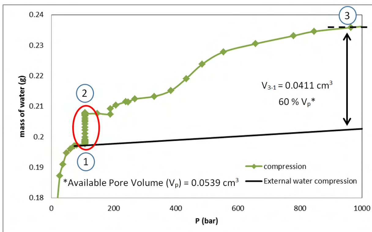
Figure 7.9 : Mass of water as a function of the pressure for a sample with 100 mg of C18-M15-Me SiMe 3 ( V_p = 0.539 \text{ cm}^3/\text{g} ).
