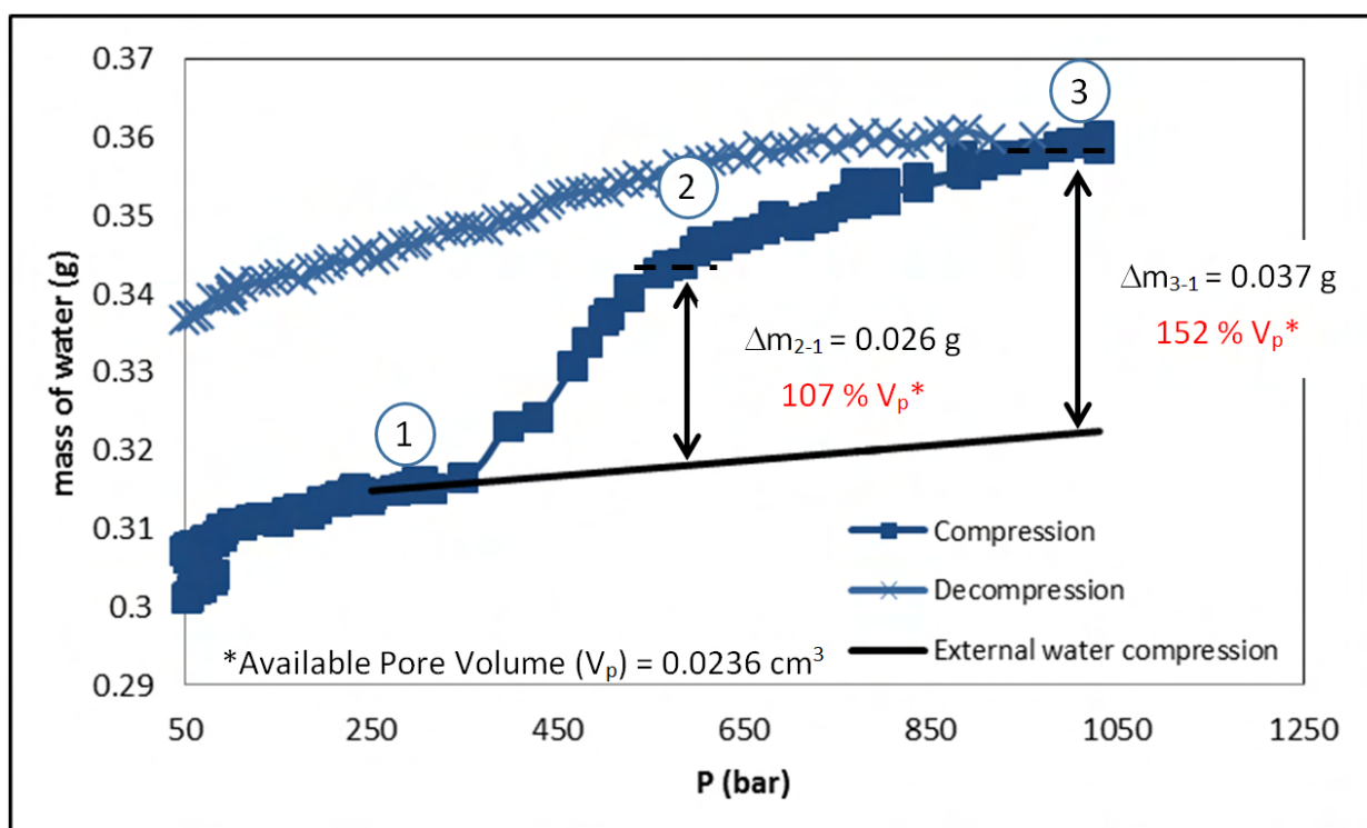
Figure 7.8: Mass of water as a function of the pressure for a sample with 122 mg of C14 MCM-41 SiMe 3 ( V_p = 0.194 \text{ cm}^3/\text{g} ).
