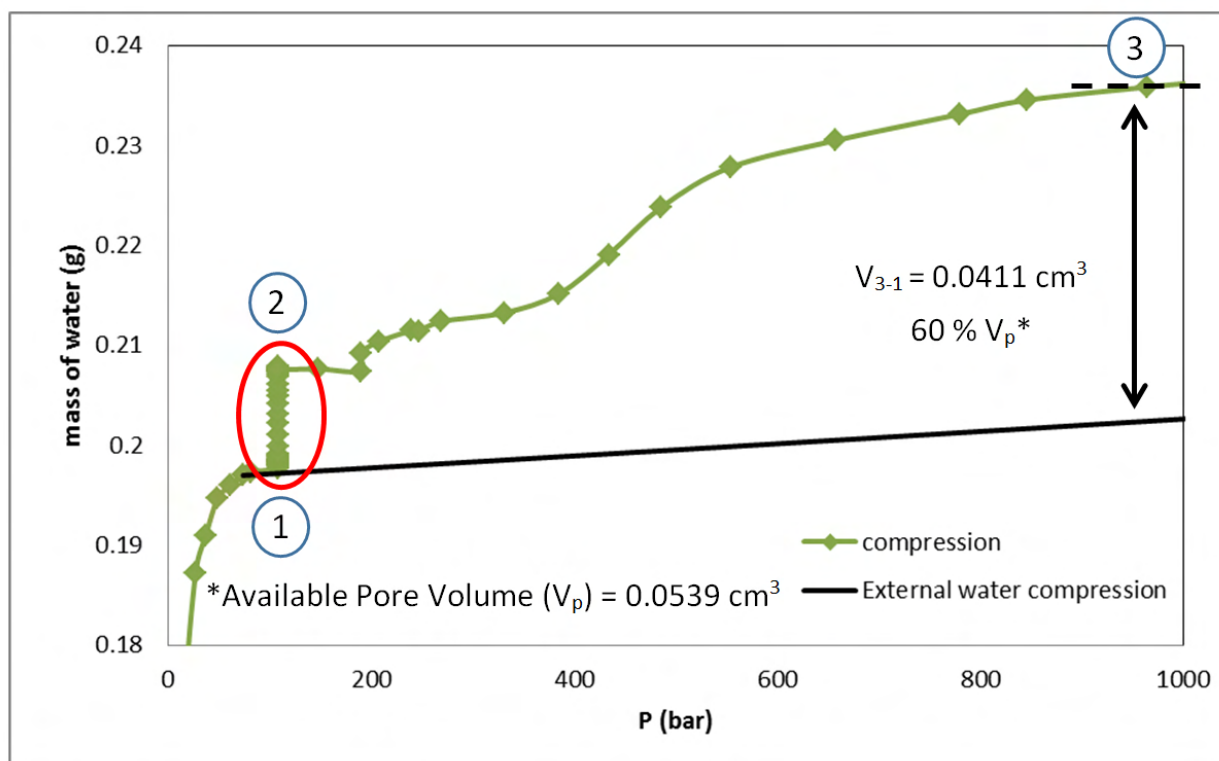
Figure 7.9 : Mass of water as a function of the pressure for a sample with 100 mg of C18-M15-Me SiMe 3 (V p = 0.539 cm 3 /g).
