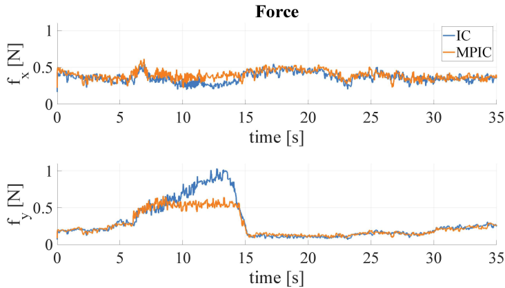
(b) Force measured at the end-effector under IC and MPIC.
