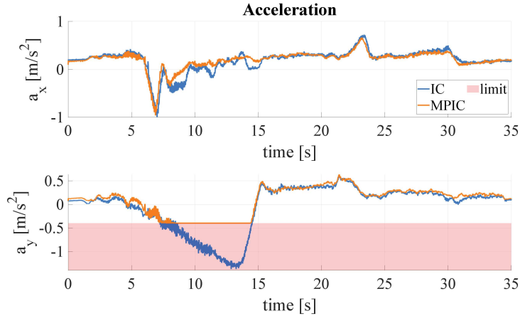
(a) End-effector accelerations under IC and MPIC.
