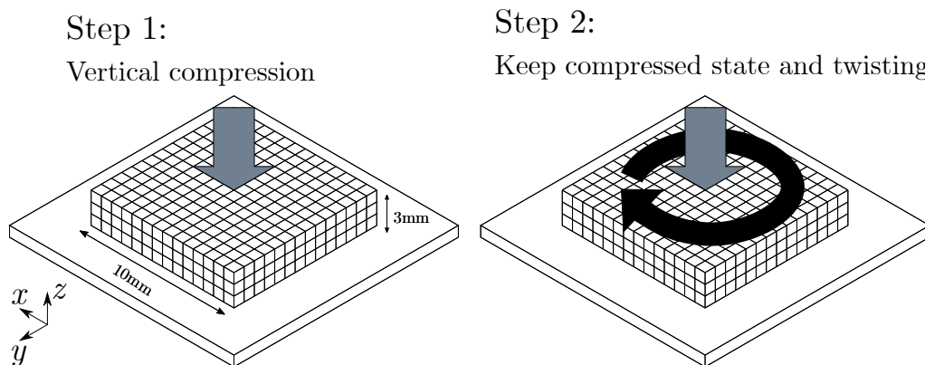
Figure 3.10: Comparison between isotropic and orthotropic adhesive twisting: Problem setup and loading sequence (Step 1, compression and adhesion process; Step 2, twisting and de-bonding process).
