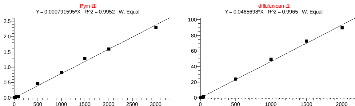
Supplementary materials S5-Figure 4s: Calibration curves of some analyzed compounds
