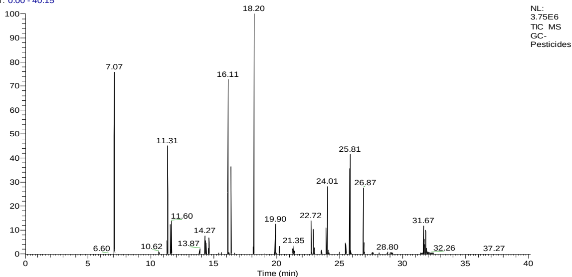
Supplementary materials S3-Figure 5: Chromatogram of PAHs, PCBs and OCPs analyzed by GC-MS/MS.
