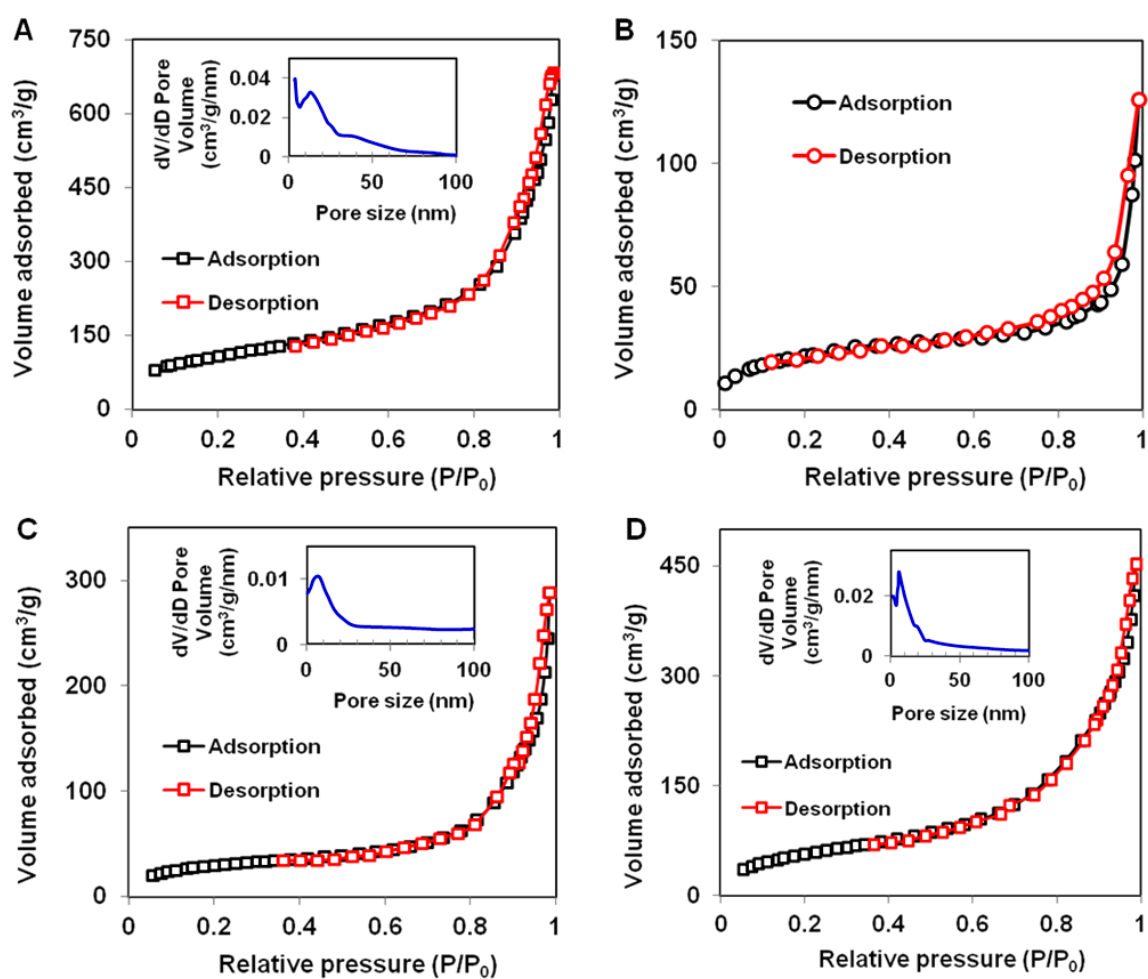
S.3-2 \text{N}_2 adsorption-desorption isotherm associated with the pore size distribution of (A) STMS, (B) pristine CNTs, (C) STMS@IBAM and (D) CNT@LPMS@IBAM
