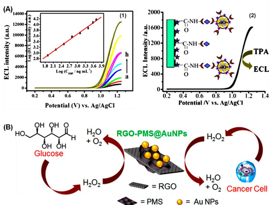
Fig.1-22 (A) MWCNTs/MS based immunosensor for detection of retinol-binding protein: (1) ECL signals of immunosensor incubated with different concentrations of RBP. Inset: calibration curve for RBP determination, (2) ECL response of electrodes modified with the designed immunosensor. 323 (B) Schematic representation of RGO-PMS@AuNPs for the electrochemical sensing of \text{H}_2\text{O}_2 liberated from cancer cells and glucose in human urine. 146
