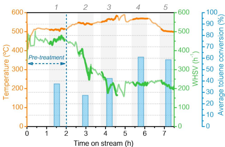
Figure 5.4. Operating conditions in the catalytic bed (T and WHSV) and average toluene conversion at atmospheric pressure for each tar sampling versus time on stream for Ni/CY/RSiC 8/5
