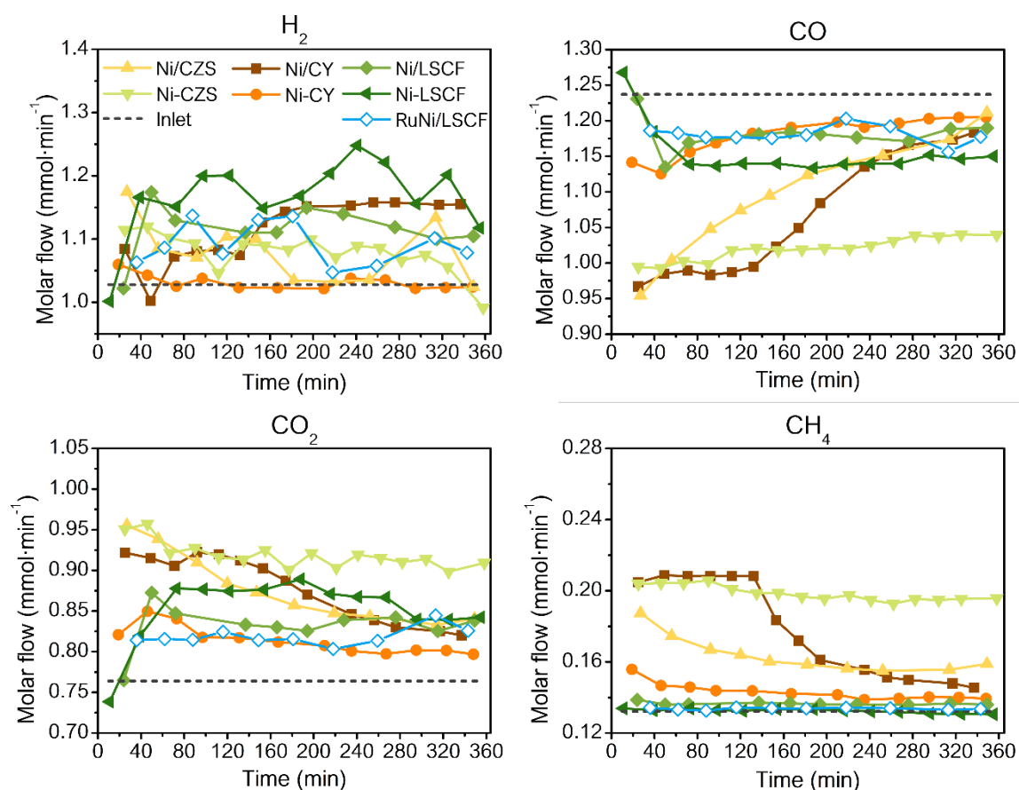
Figure 3.4. Partial molar flows at the outlet of the reactor vs time on stream during steam reforming of phenol at 550 °C over the Ni-based catalysts (WHSV gas = 370 h -1 ; WHSV tar,Ni 0 = 14 h -1 and S/C tar = 16.5)
