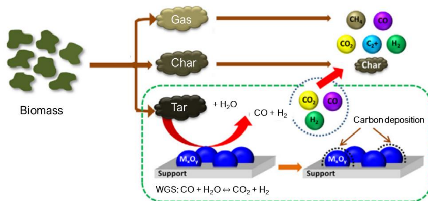
Figure 1.9. Tar abatement through catalytic steam reforming ( M_xO_y represents a metal oxide catalyst) [35]
