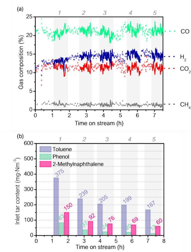
Figure 5.3. Conditions at the inlet of the catalytic reactor (a) inlet gas composition and (b) inlet tar content for each tar sampling versus time on stream
