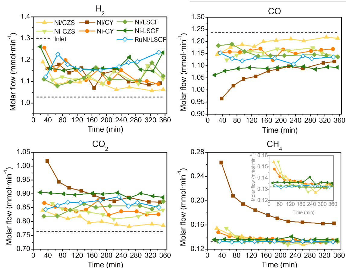
Figure 3.5. Partial molar flows at the outlet of the reactor vs time on stream during steam reforming of toluene at 550 °C over the Ni-based catalysts (WHSV gas = 370 h -1 ; WHSV tar = 26 h -1 and S/C tar = 7.7)
