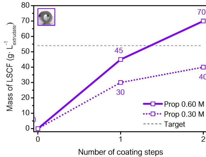
Figure 4.13. Effect of support precursor concentration (0.60 – 0.30 M) on the mass uptake of LSCF mixed oxide
