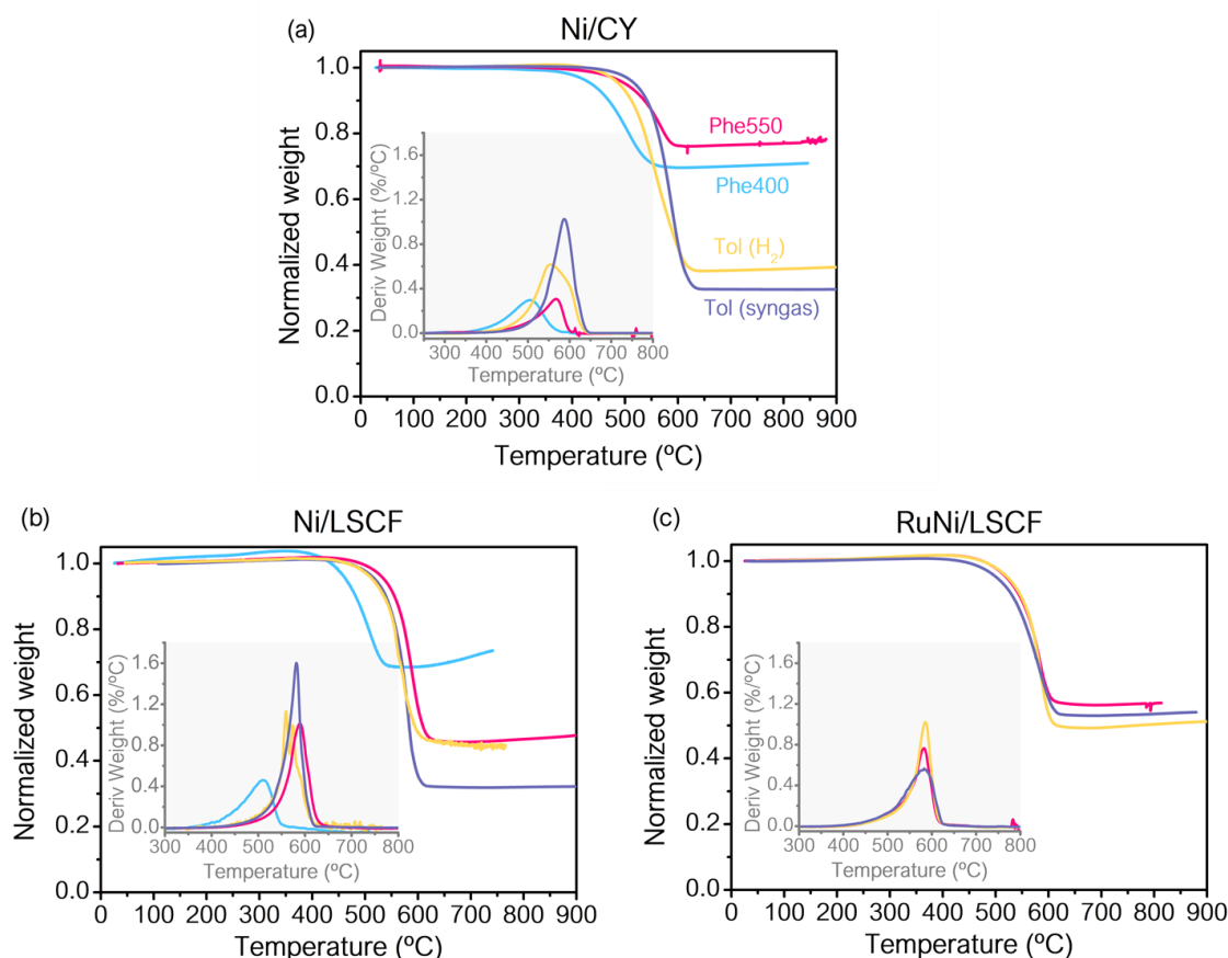
Figure 3.12. TGA analysis of the selected catalysts post steam reforming reactions: (a) Ni/CY, (b) Ni/LSCF and (c) RuNi/LSCF catalysts. Color code : phenol reforming at 400 °C (blue) and at 550 °C (pink), toluene reforming at 550 °C - \text{H}_2 (yellow) and - syngas (purple)
