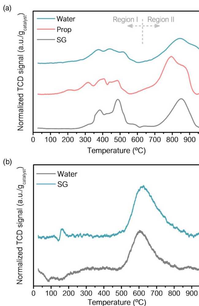
Figure 4.7. \text{H}_2 -TPR profile of selected supports obtained by gel (SG) and solution (prop or water) calcination: (a) LSCF- and (b) CY supports
