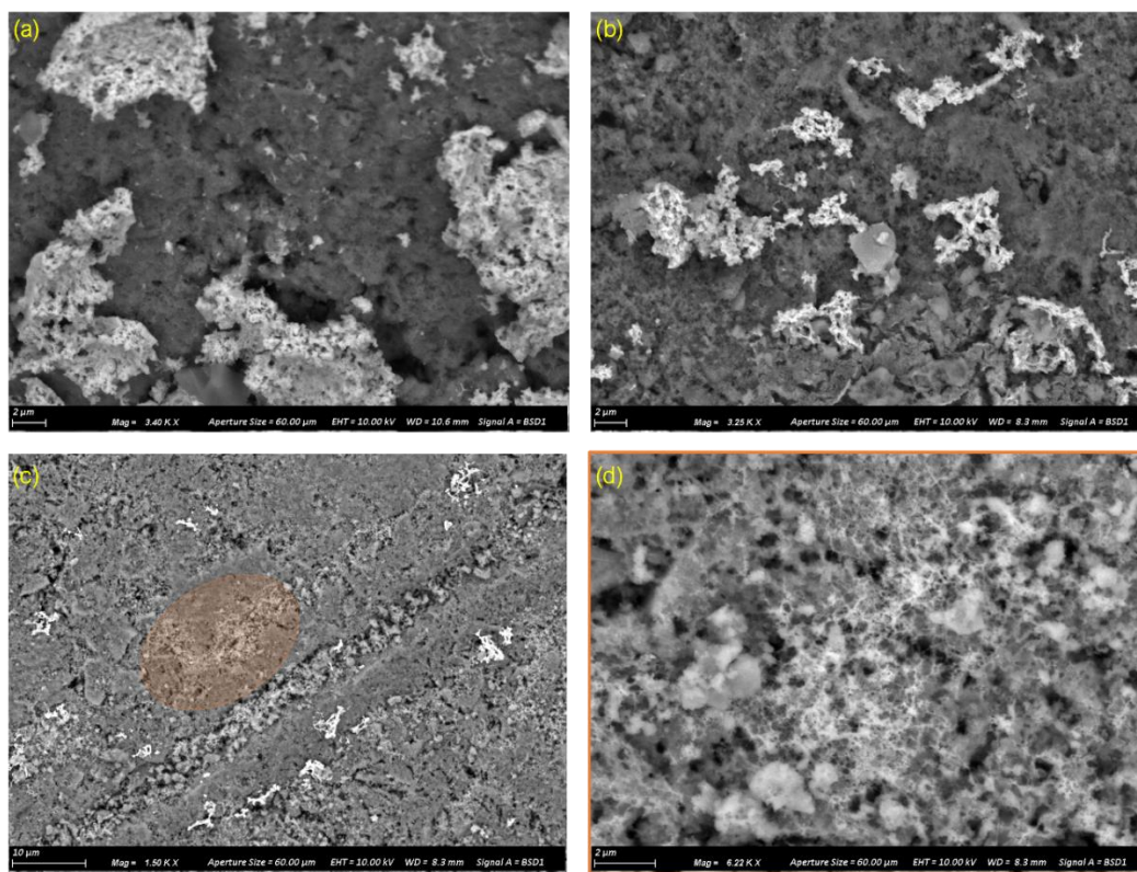
Figure 4.14. SEM images of \beta -SiC extrudates after (a) 1 st coating - 0.60 M solution; (b) 1 st coating - 0.30 M and (c-d) 2 nd coating - 0.30 M
