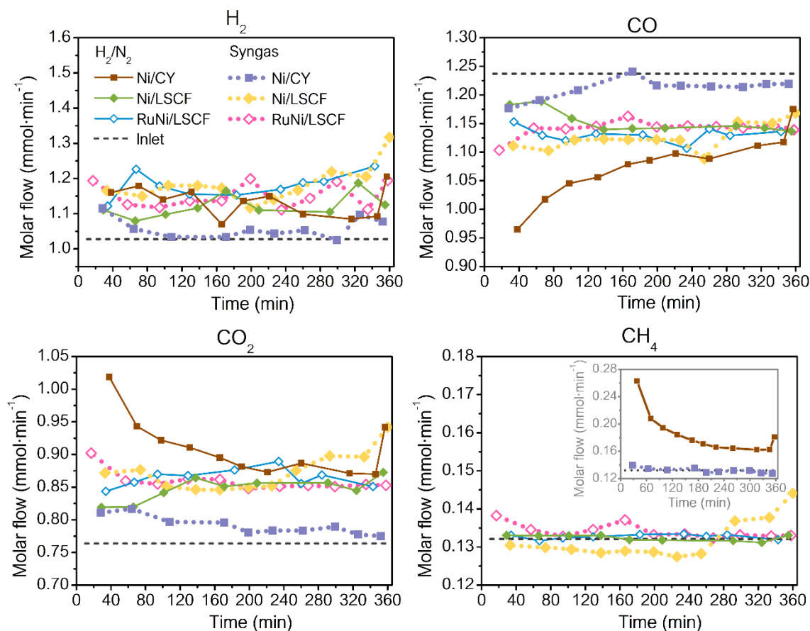
Figure 3.10. Partial molar flows at the outlet of the reactor vs time on stream during toluene reforming at 550 °C over Ni/CY, Ni/LSCF and RuNi/LSCF catalysts ( \text{WHSV}_{\text{gas}} = 370 \text{ h}^{-1} ; \text{WHSV}_{\text{tar}} = 26 \text{ h}^{-1} and \text{S/C}_{\text{tar}} = 7.7 ). Solid and dot lines: pretreatment under \text{H}_2/\text{N}_2 and syngas respectively.
