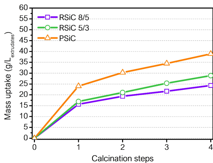
Figure 4.8. Mass uptake due to \beta -SiC oxidation through successive calcination steps at 800 °C for 6 h (heating ramp of 2 °C·min -1 )
