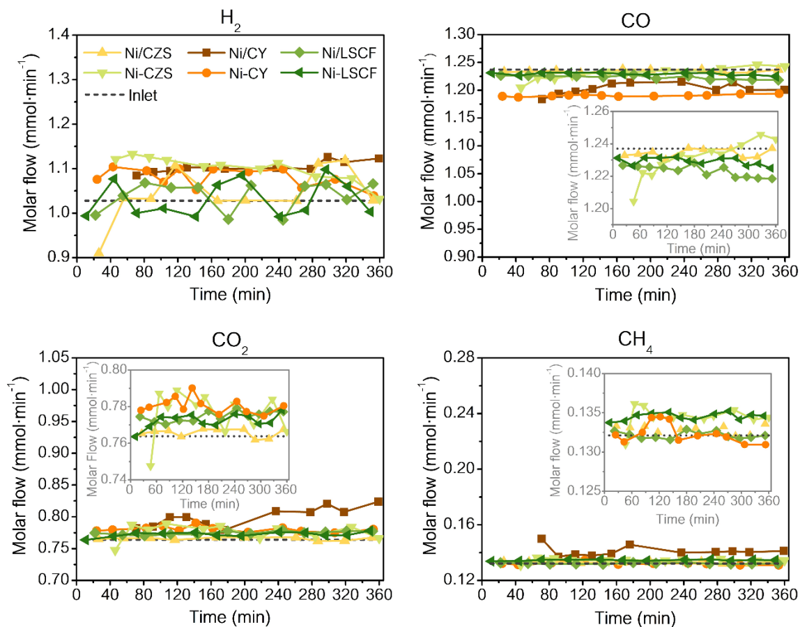
Figure 3.3. Partial molar flows at the outlet of the reactor vs time on stream during steam reforming of phenol at 400 °C over the Ni-based catalysts (WHSV gas = 370 h -1 ;
