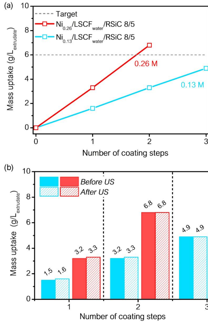
Figure 4.18. Effect of \text{Ni}(\text{NO}_3)_2 solution concentration (0.13 – 0.26 M) on (a) the mass uptake of \text{Ni}^0 and (b) the anchoring strength for \text{LSCF}_{\text{water}}/\text{RSiC } 8/5 after successive coating steps
