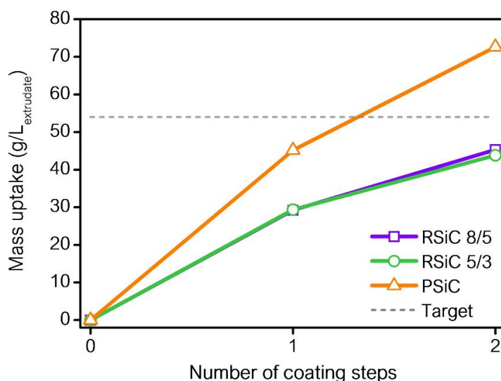
Figure 4.21. Effect of \beta -SiC extrudate shapes on the mass uptake of CY mixed oxide
