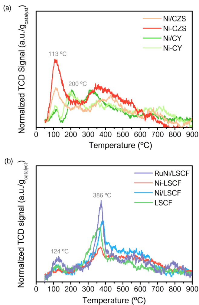
Figure 2.8. H 2 -TPD profiles of the synthesized materials: (a) Ce-based systems (CZS and CY) and (c) LSCF-based systems
