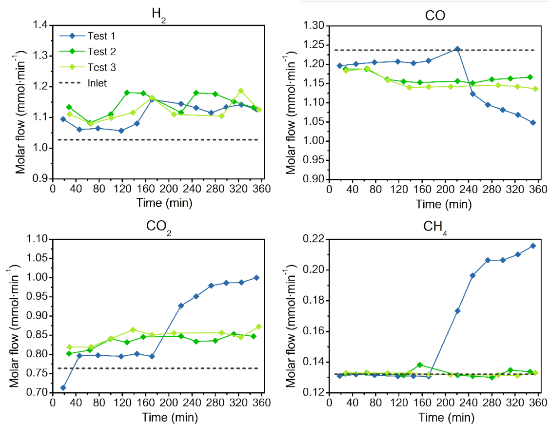
Figure 3.15. Partial molar flows at the outlet of the reactor vs time on stream during toluene reforming at 550 °C over Ni/LSCF catalyst ( \text{WHSV}_{\text{gas}} = 370 \text{ h}^{-1} ; \text{WHSV}_{\text{tar}} = 26 \text{ h}^{-1} and \text{S/C}_{\text{tar}} = 7.7 ). Reproducibility test
